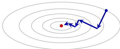
gradient descent
