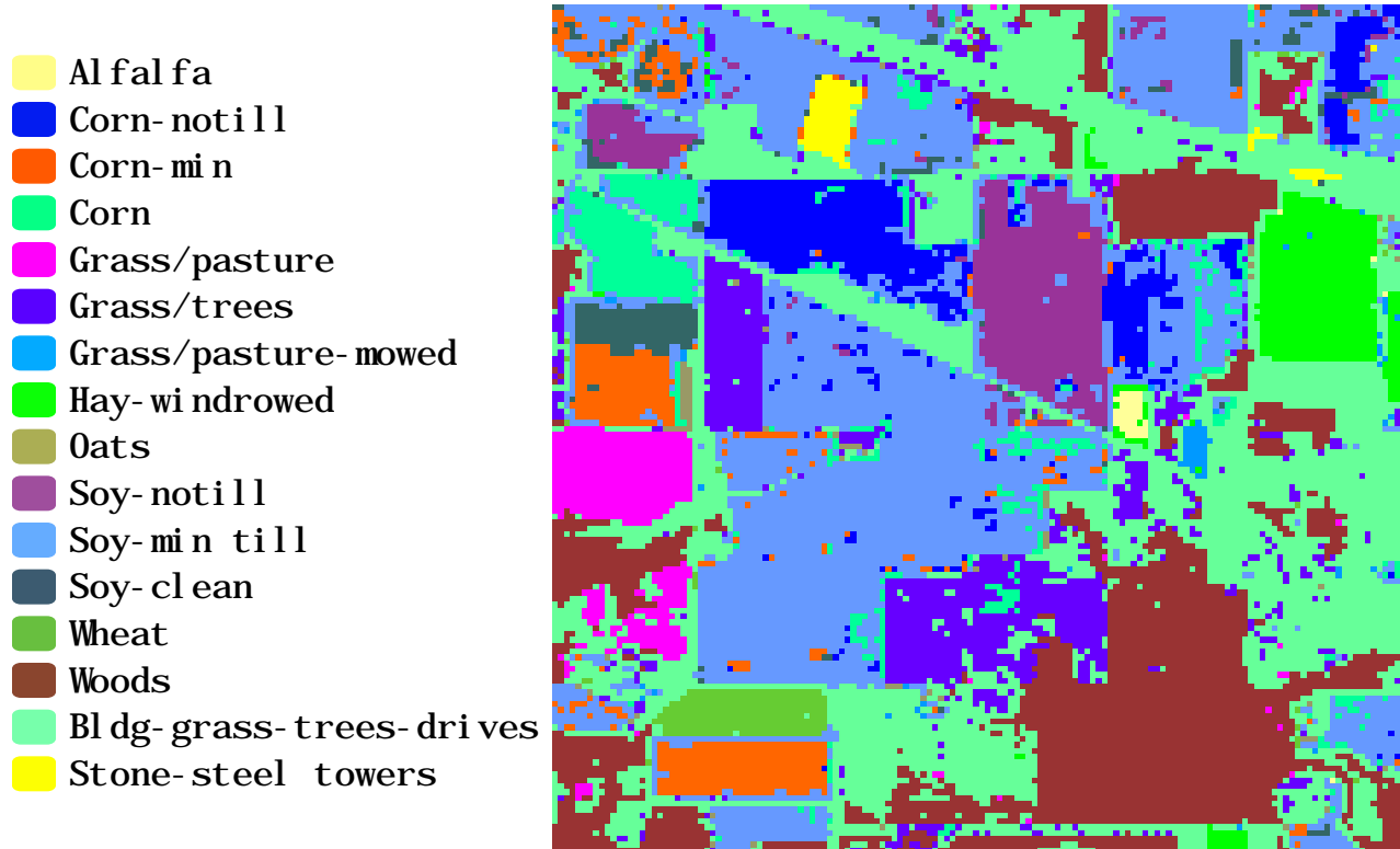
Figure 15. ECHO classification with 3 new training fields added (in color). 56 seconds
