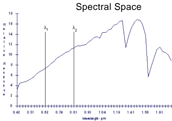
(a) The spectral response of a specific soil.
