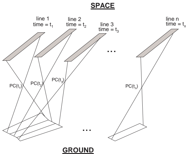
Figure 6. Pushbroom Camera
