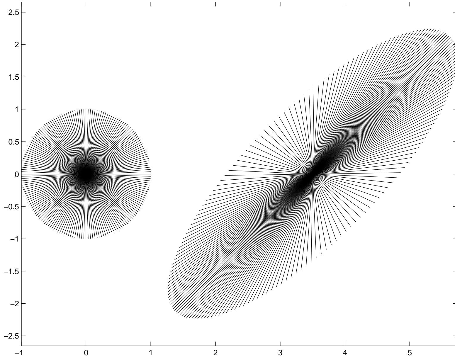
cluster of unit vectors (x) around origin, transformed by A^*x , A=[2 \ 1; 1 \ 2]
