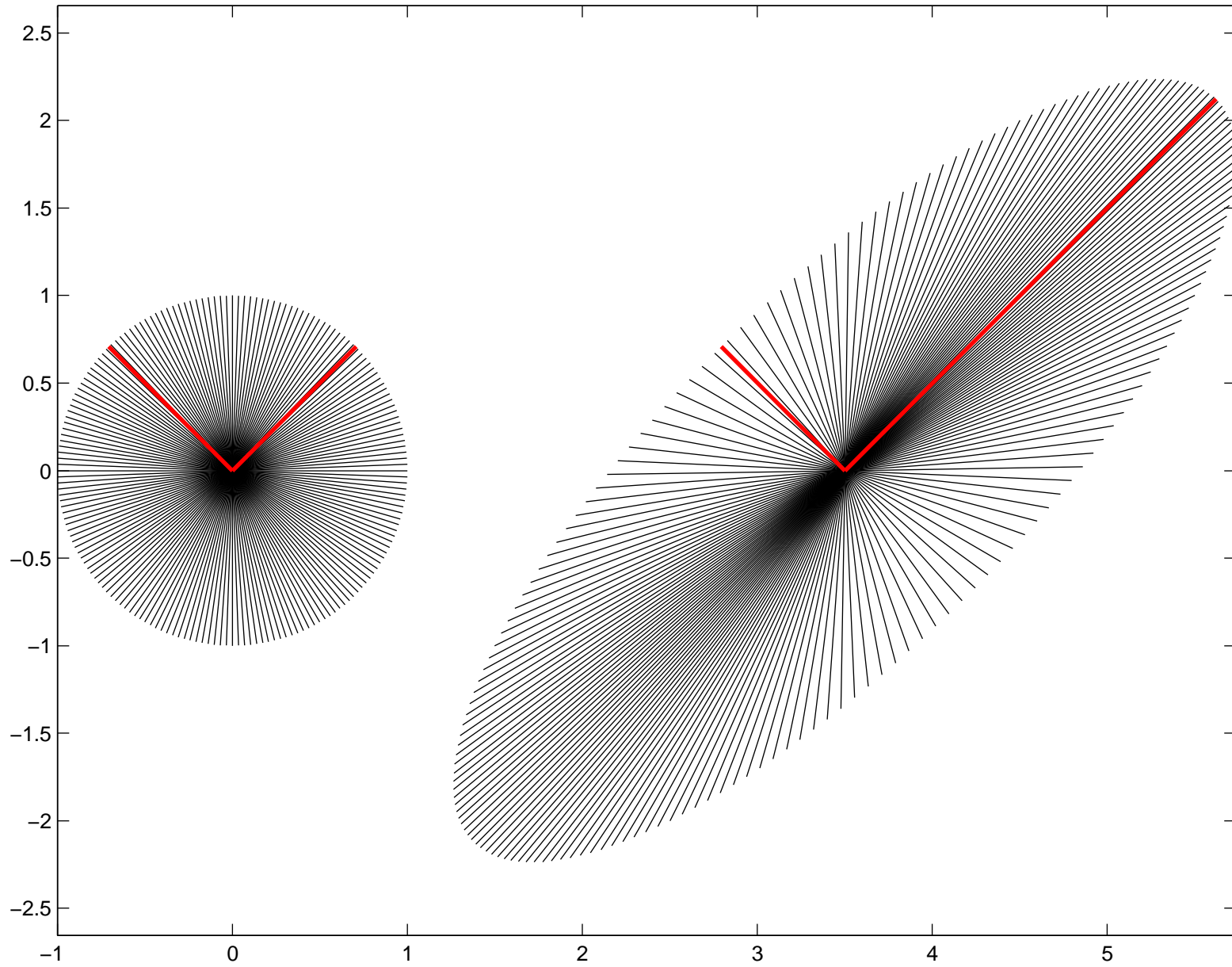
eigenvectors left, transformed by A*x , same direction, but scaled
