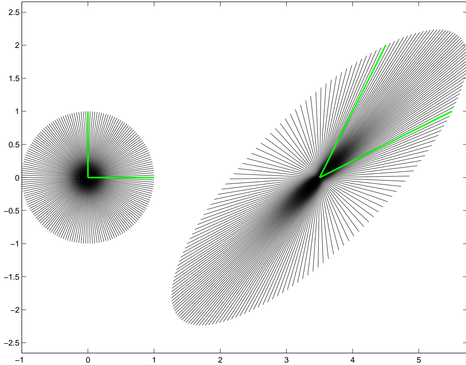
unit vectors along axes left, transformed by A \cdot x
