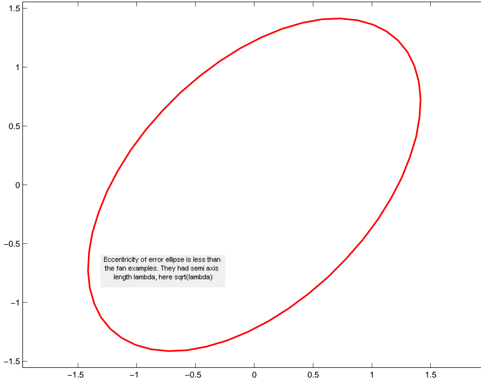
standard error ellipse, chi-sqr=1.0, for SIG=[2 1;1 2]
