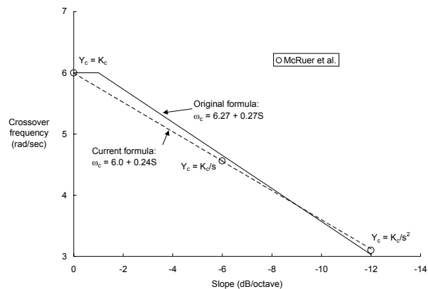
Figure 3. Smith-Geddes criterion frequency (data from fixed-base simulation; 35 figure reproduced from Mitchell and Hoh 32 )
