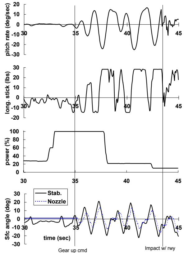
Figure 11. Time history of the YF-22 PIO
