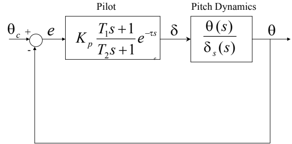
Figure 7. Closed-loop pilot-vehicle system
