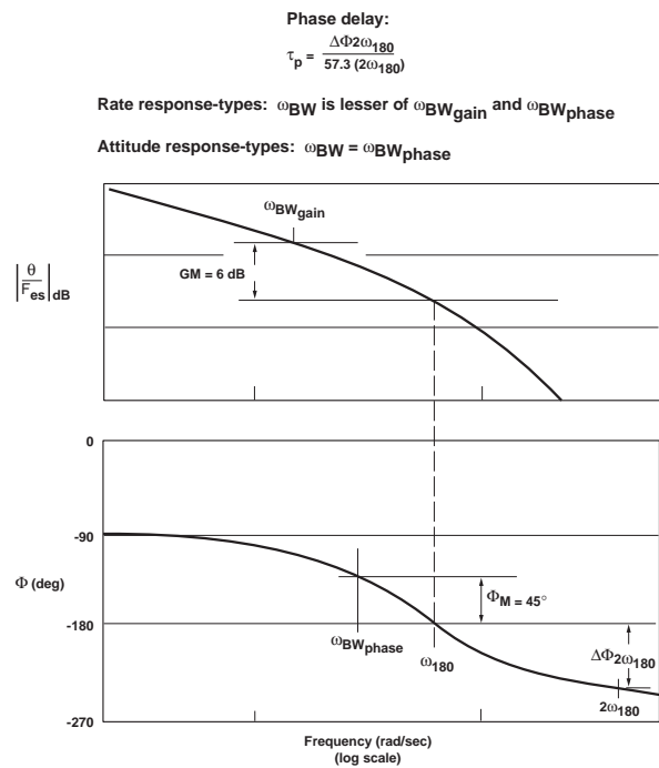
Figure 12. Definitions of pitch attitude Bandwidth and Phase Delay 32 (flight path Bandwidth \omega_{BW\gamma} is measured from \gamma/F_{es} and is defined as \omega_{BWphase} )
