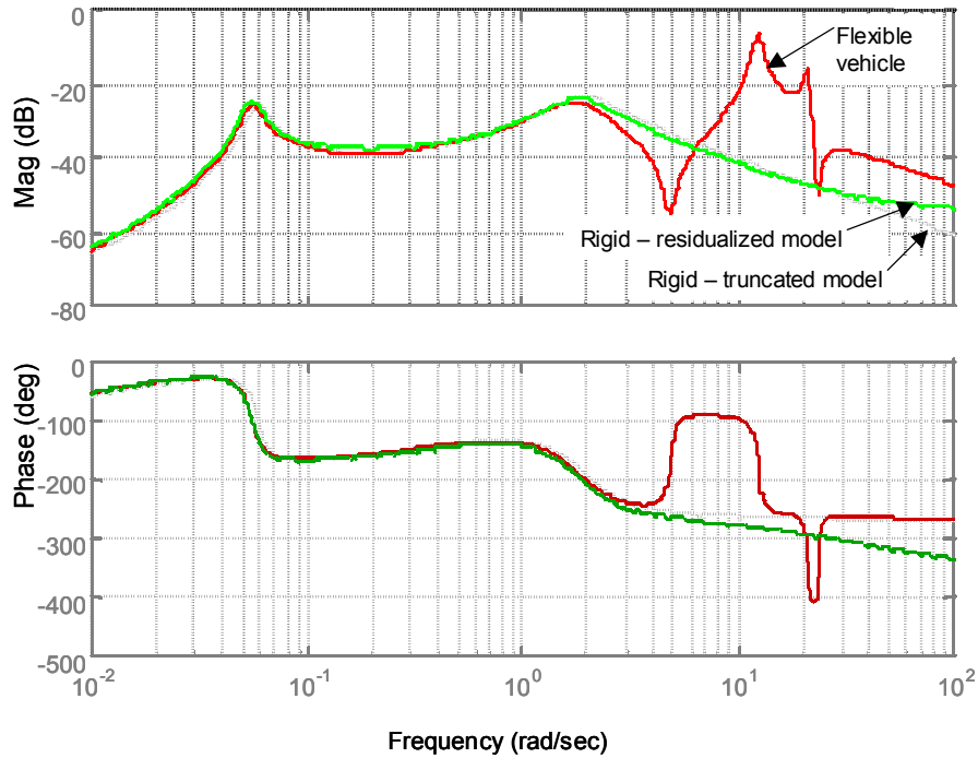
Figure 15. Pitch rate to elevator frequency responses - flexible and rigid models
