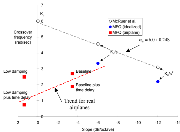
Figure 4. Identified crossover frequencies in fixed-base compensatory pitch tracking from Minimum Flying Qualities (MFQ) study 36 (figure modified from Mitchell and Hoh 32 )
