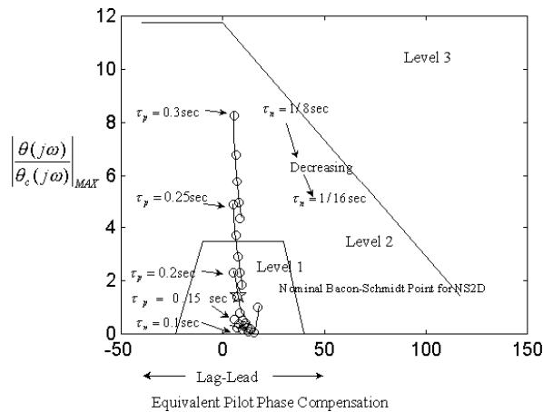
Figure 9. Sensitivity of estimated pilot ratings to variations in physiological parameters
