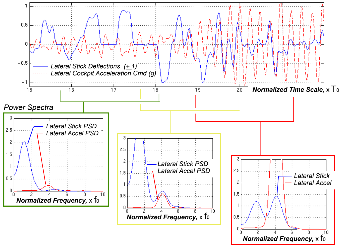
Figure 17. Example of biodynamic coupling incident
