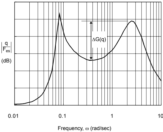
Figure 13. Definition of pitch rate overshoot parameter, \Delta G(q)
