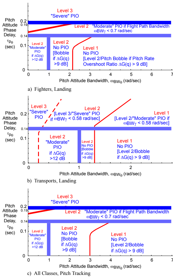
Figure 14. PIO criteria for pitch response 32 (dynamics of the cockpit control feel system included)
