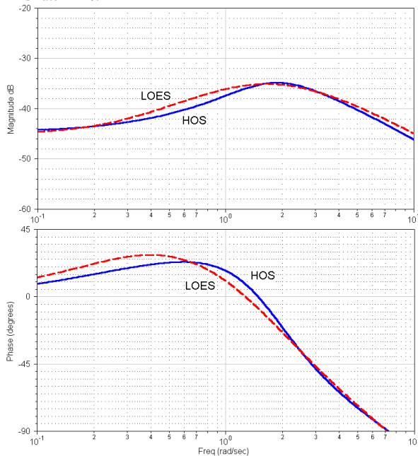
Figure 2. Example application of the equivalent systems approach (F-18 in power approach 30 )
