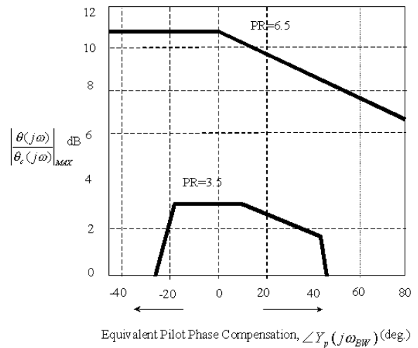
Figure 8. Neal-Smith criteria
