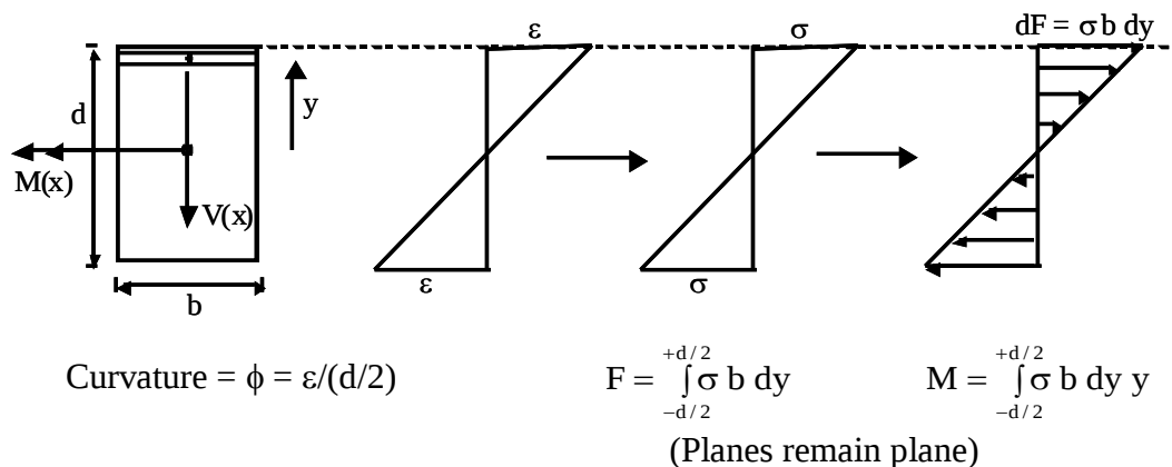
Figure 2. Longitudinal axial stresses caused by internal bending moment.
