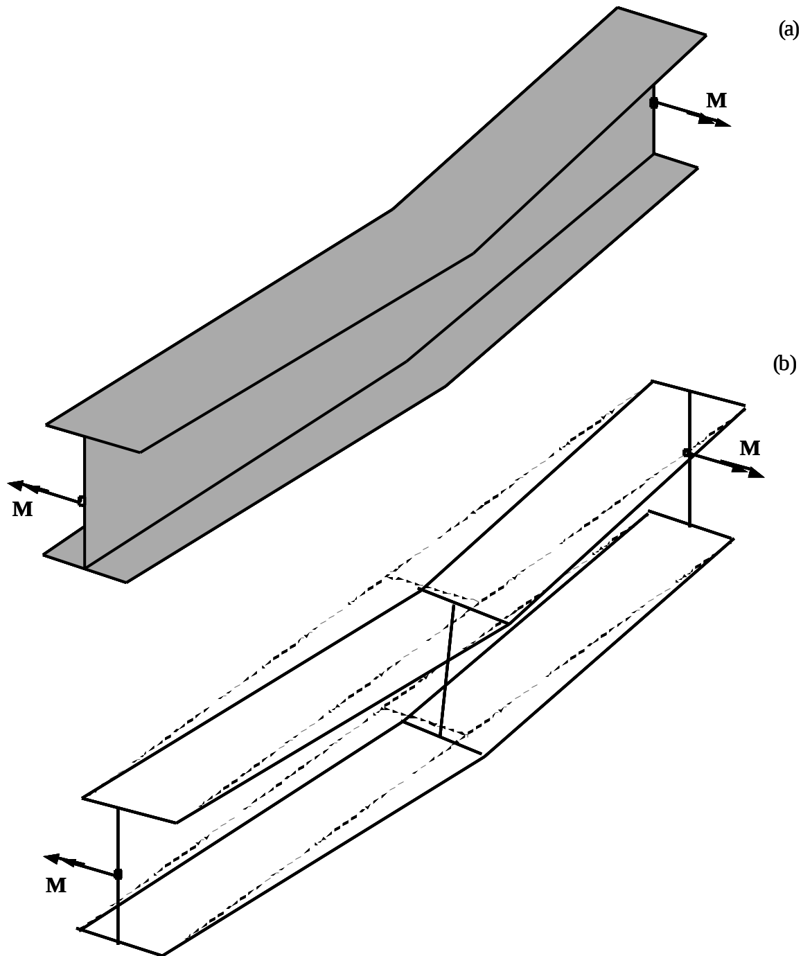
Figure 9. Lateral-torsional buckling of a wide-flange beam subjected to constant moment.
