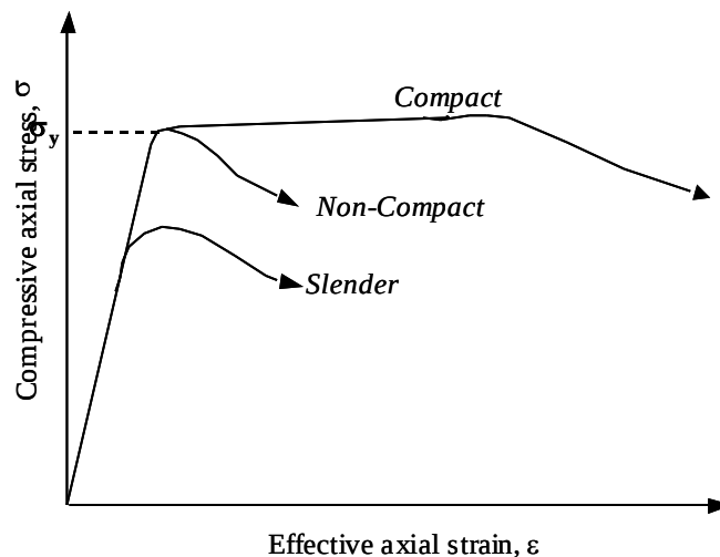
Figure 8. Stress-strain response of plates subjected to axial compression and local buckling.
