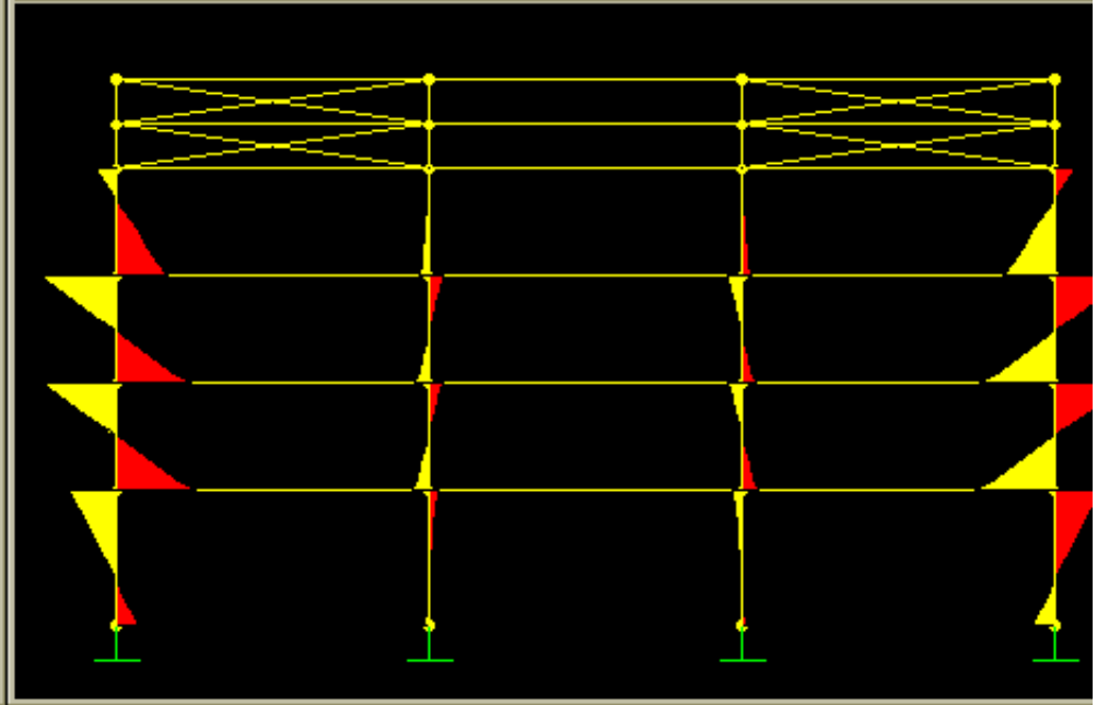
Moment 2-2 Diagram (GRAVITY)
