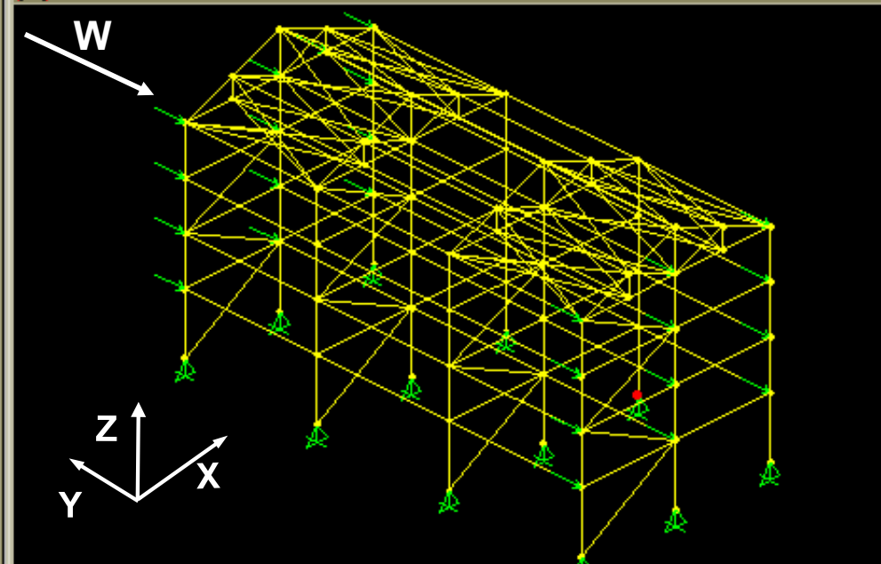
Deformed Shape (WINDY)
