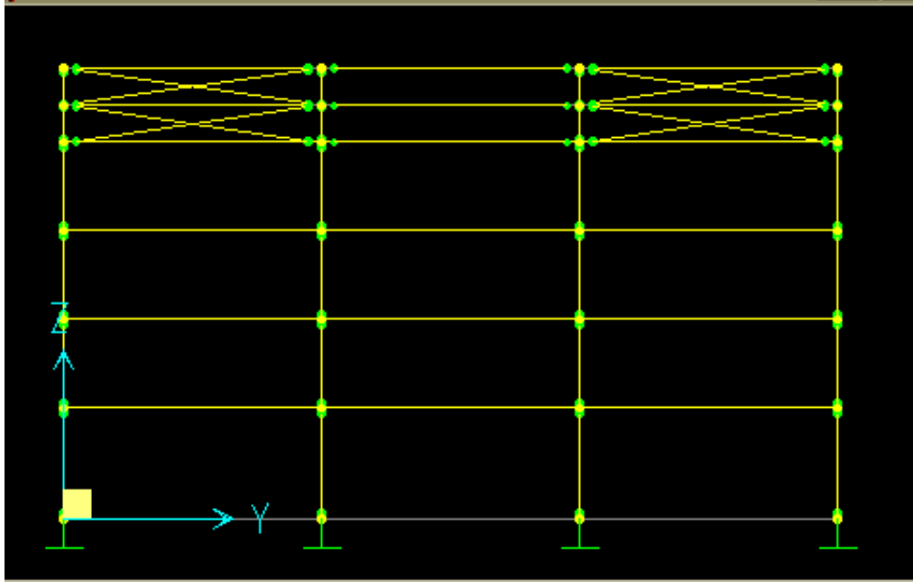
ELEVATION OF MOMENT FRAME
