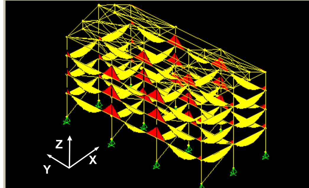
Moment 3-3 Diagram (GRAVITY)
