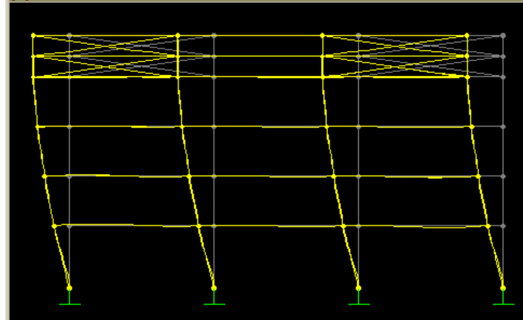
Deformed Shape (WINDY)
