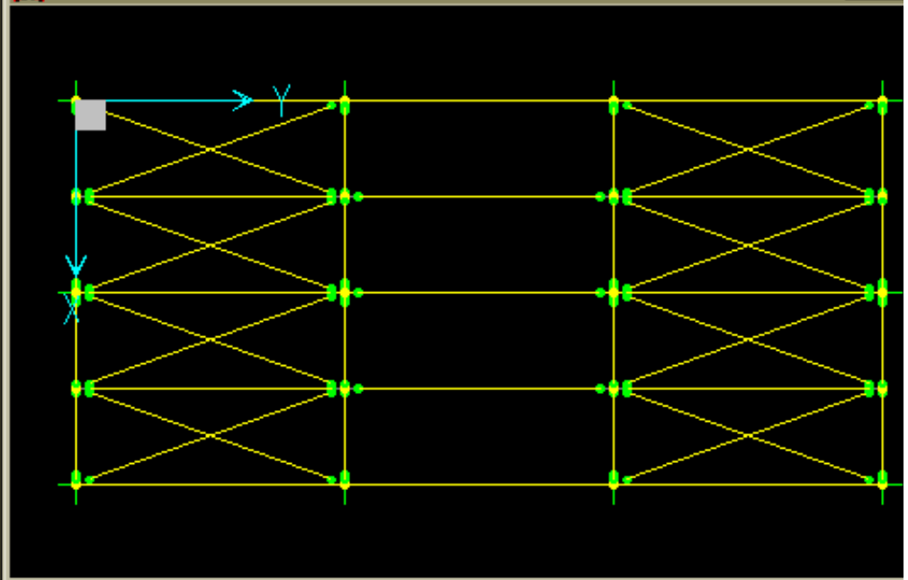
PLAN OF ROOF TRUSS
