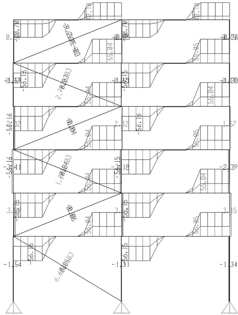
Shear Force 2-2 Diagram (Envelope)
