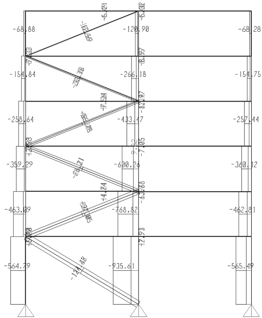
Axial Force Diagram (Envelope)
