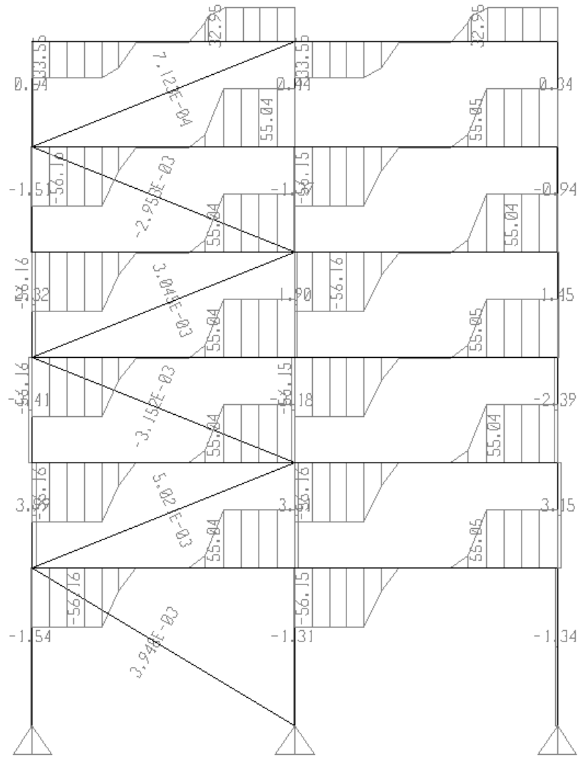
Shear Force 2-2 Diagram (1.2D+1.6L+0.5Lr)
