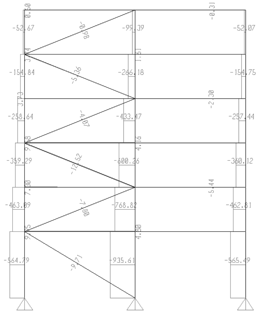
Axial Force Diagram (1.2D+1.6L+0.5Lr)
