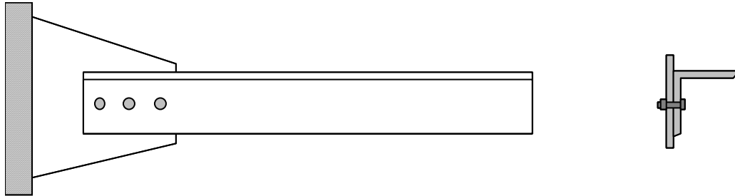
Figure 2.3 Single angle with bolted connection to only one leg.
