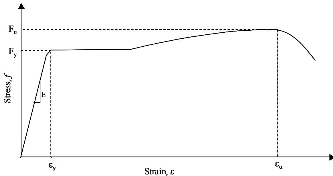
Figure 2.2 Stress-strain behavior of steel
