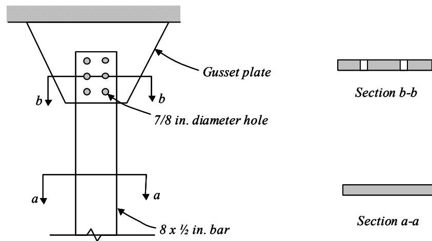
Figure 2.1 Example of tension member.
