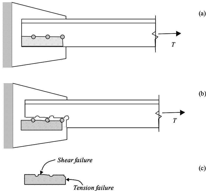
Figure 2.4 Block shear failure of single angle tension member
