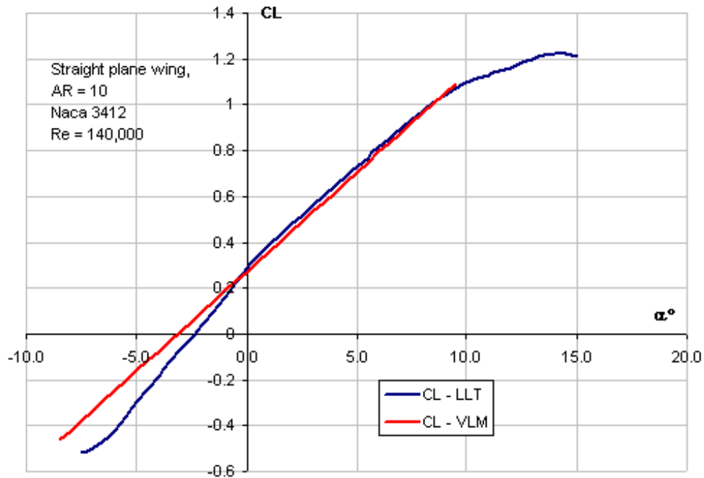
Figure 27 – Linear and Non-Linear modeling
