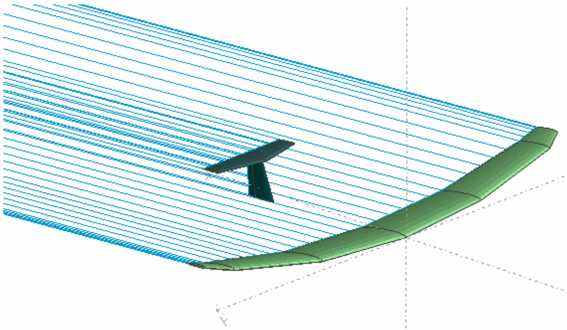
Figure 13: Straight wake
