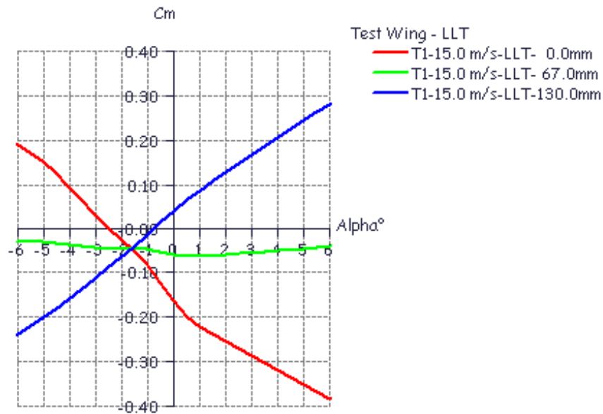
Figure 30 – Wing Neutral Point
