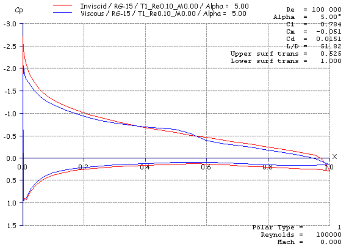
Figure 2 : C_p calculation
