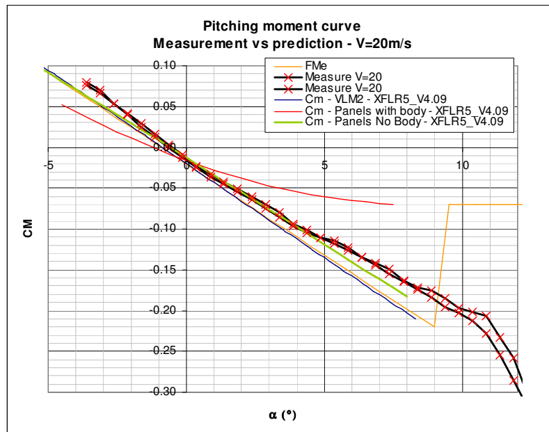
Figure 36 – Predicted pitch moment vs. experimental results
