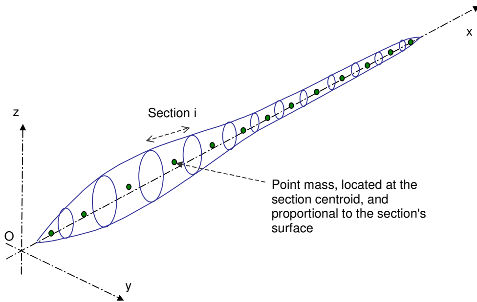
Figure 9 – Mass representation for the body
