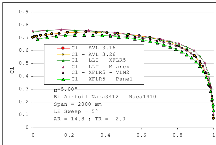
Figure 38 – Lift coefficient - Comparison to AVL and Miarex
