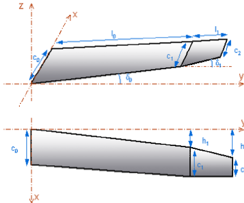
Figure 7 – Wing Definition
