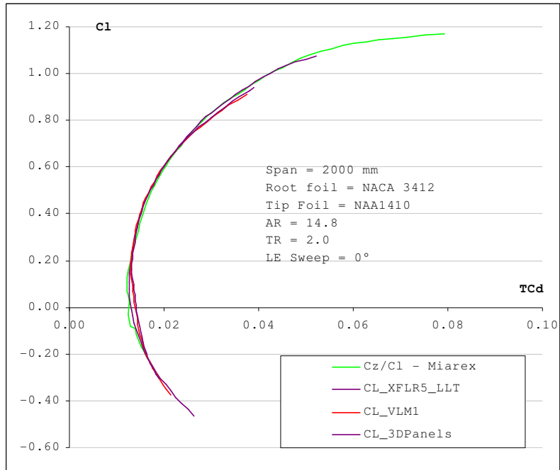
Figure 37 – Comparison to results from Miarex
