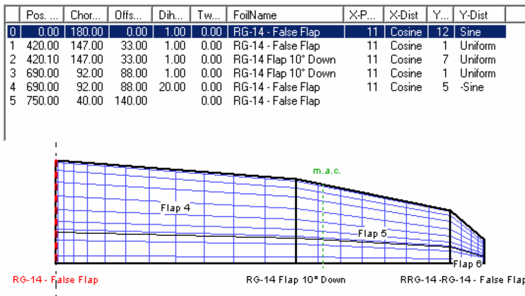
Figure 8 – Flap Definition
