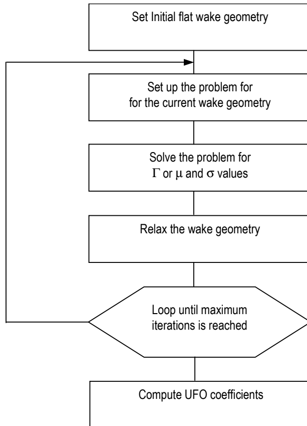
Figure 29 – Wake roll-up iteration process
