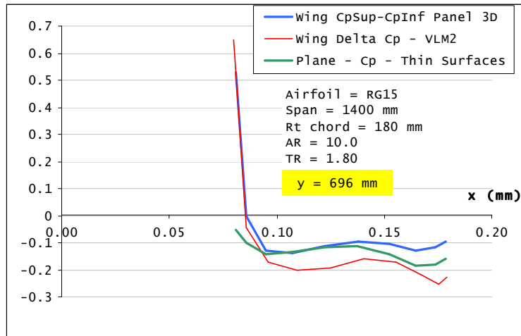
Figure 25 – Cp comparison for different analysis methods
