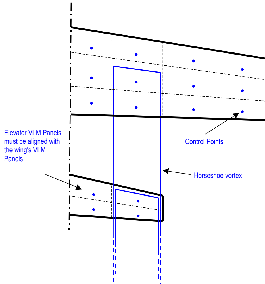
Figure 12: VLM Panel arrangement for a plane
