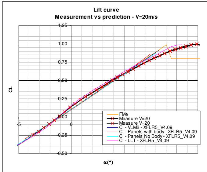
Figure 34 – Predicted lift curve vs. experimental results
