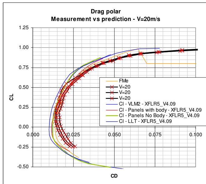
Figure 35 – Predicted drag polar vs. experimental results
