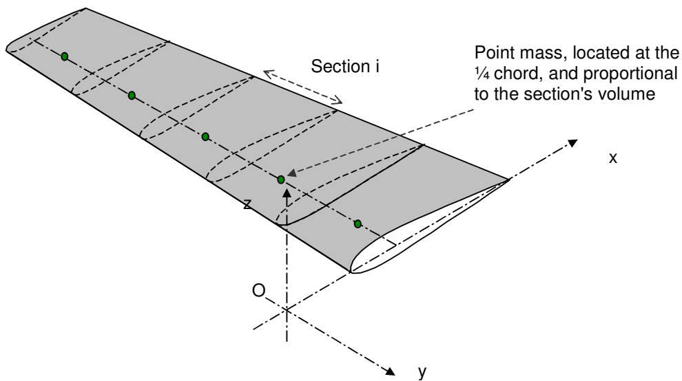
Figure 10 – Mass representation for the wing
