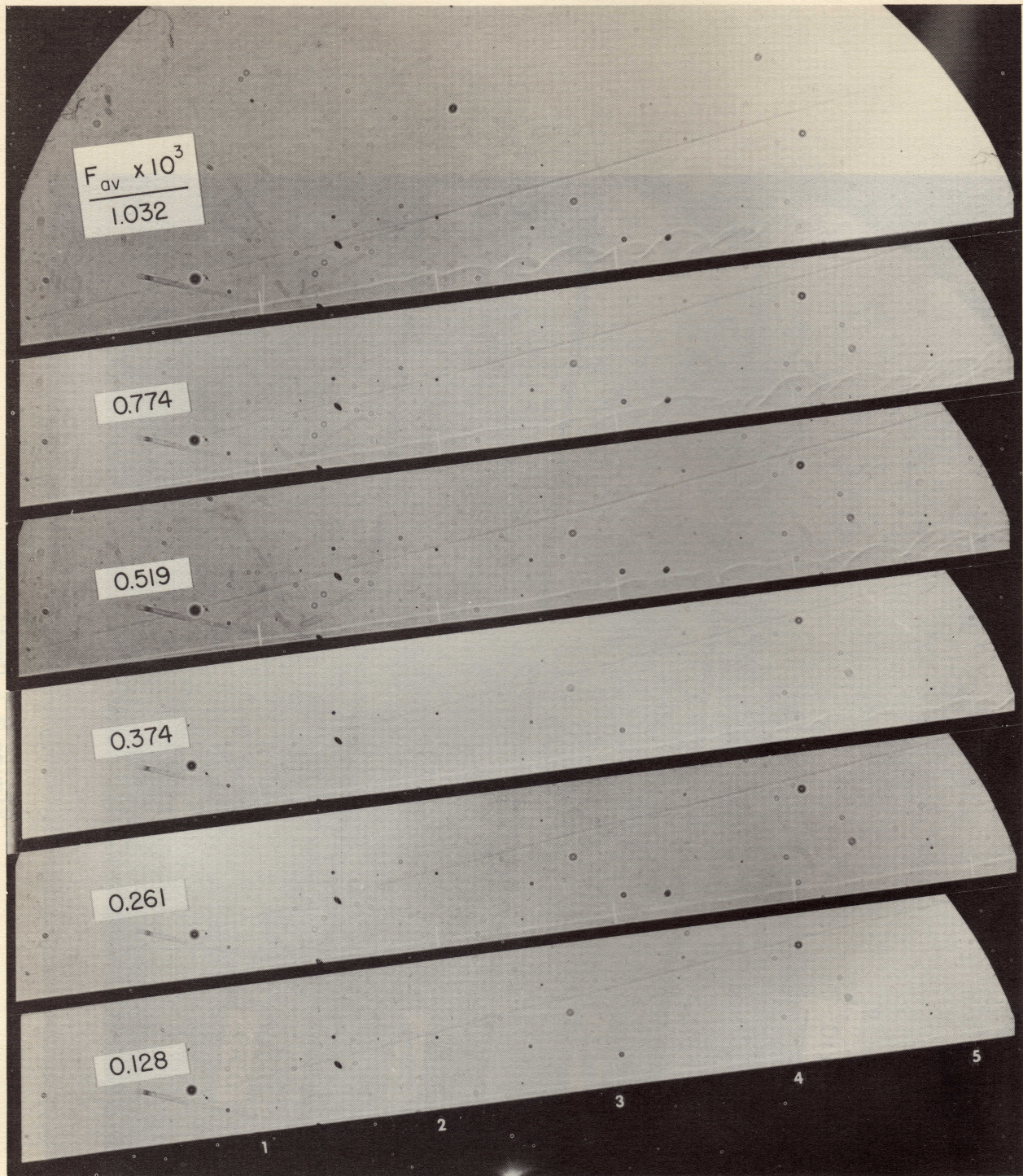
(d) Helium injection; M_c = 4.34 ; F_{av} \times 10^3 = 0.128, 0.261, 0.374, 0.519, 0.774, 1.032 .
