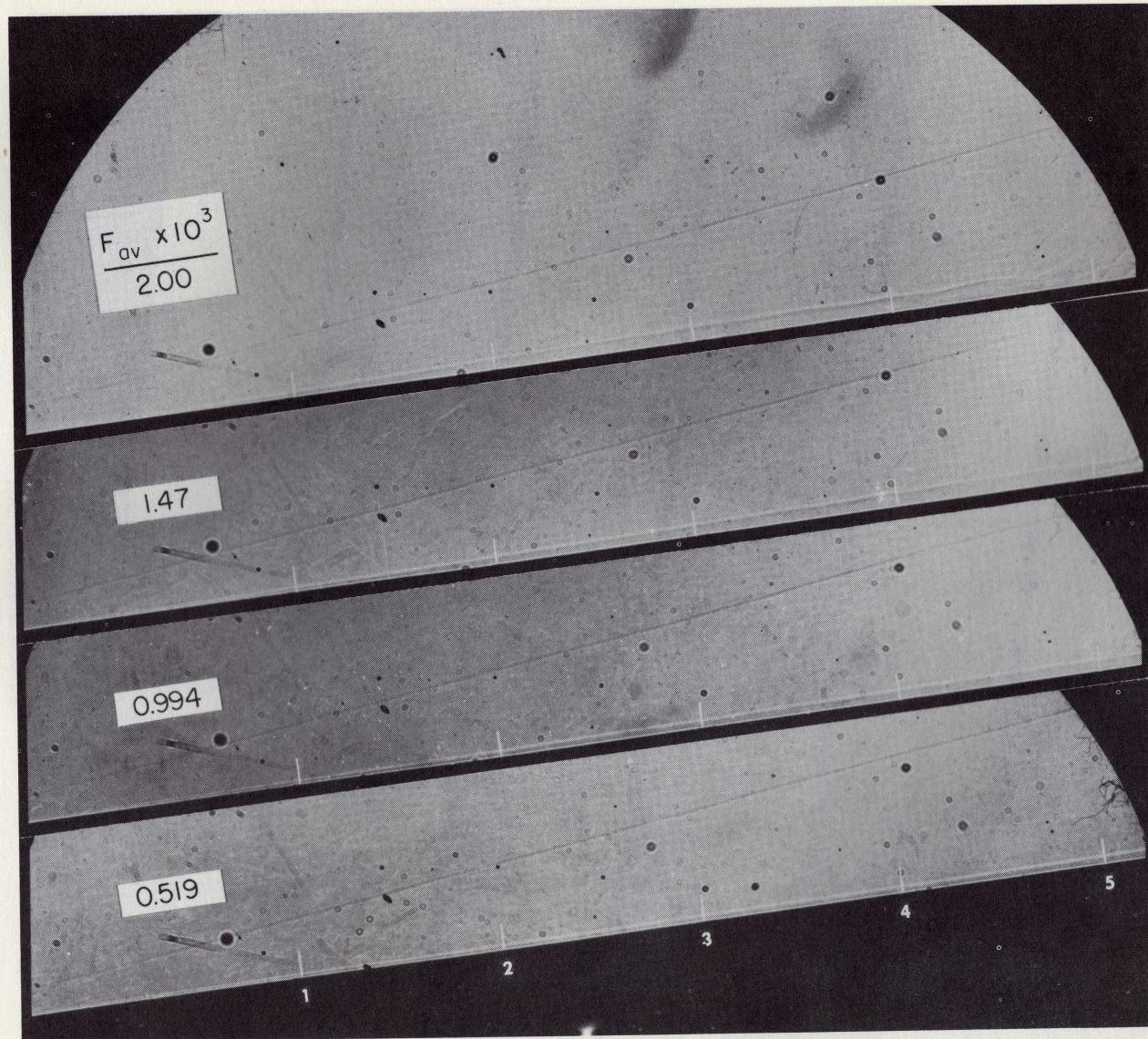
(c) Freon-12 injection; M_c = 4.34 ; F_{av} \times 10^3 = 0.519, 0.994, 1.47, 2.00 .
