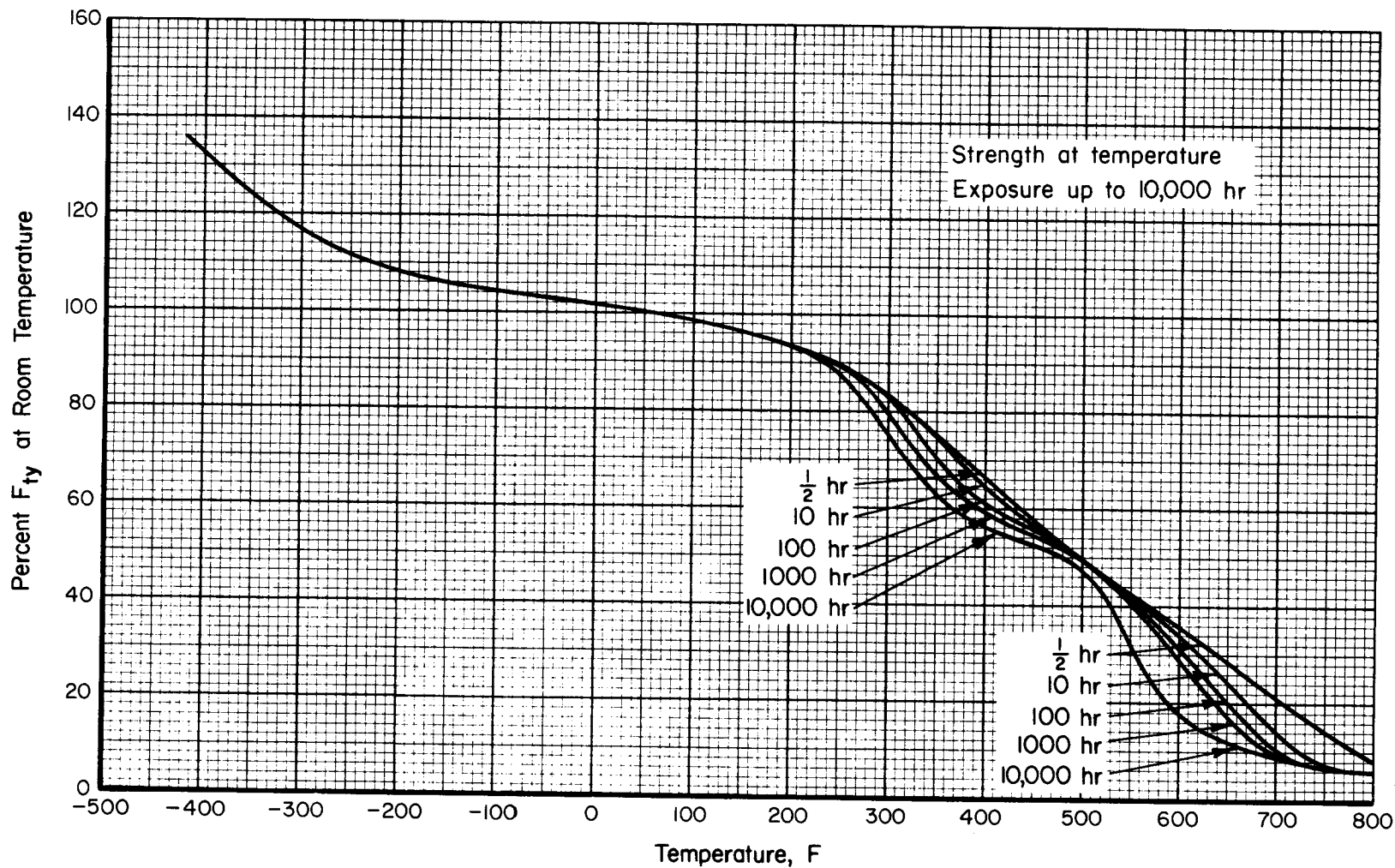
FIGURE 3.2.6.1.1(b). Effect of temperature on the tensile yield strength ( F_{ty} ) of 2219-T62 aluminum alloy bare and clad sheet and plate 0.040-1.000 in. thick.
