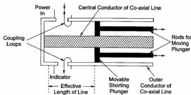
Fig. 16.1 Co-axial Wavemeter
