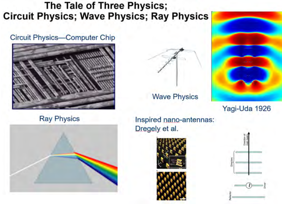
Figure 30.1: The world of electromagnetics morphs from circuit physics to wave physics, and then ray physics. The plethora of physics that emerges in electromagnetics is fascinating. Different mathematical tools are devised to solve electromagnetics problems in these regimes. At low frequencies, KCL, KVL, and potential theory can be used to describe the working of most devices. At mid-frequencies, full Maxwell's equations have to be solved to capture the wave physics correctly. At high frequencies, electromagnetic waves behave like particles and rays. Ray tracing algorithms are often used to capture their wave physics. What is missing here is the quantum nature of electromagnetic fields that will be discussed at the end of this course.
