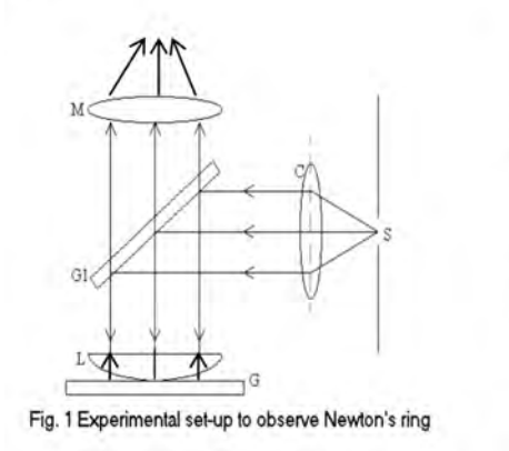
Figure 38.1: A Newton's rings experiment that indicates the wave nature of light (courtesy of [309]).
