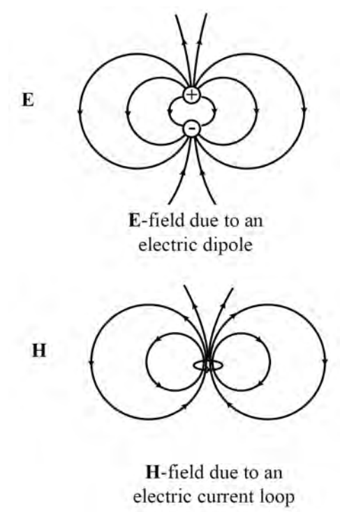
Figure 17.11: Sketches of the electric field \mathbf{E} due to an electric dipole and the magnetic field \mathbf{H} due to a electric current loop. The \mathbf{E} and \mathbf{H} fields have the same pattern, and can be described by the same formula. Hence, the magnetic field of a current loop resembles that of a magnetic dipole. As such, a current loop is a good mimicry of a magnetic dipole.
