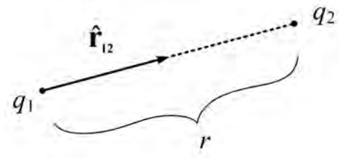
Figure 1.5: The force between two charges q_1 and q_2 . The force is repulsive if the two charges have the same sign.
