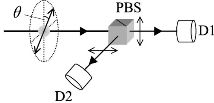
Figure 39.4: Polarization of the incident photon can be detected with a polarizing beam splitter (PBS) and single photon detectors (from Quantum Optics, M. Fox [332]). In quantum theory, the polarization is random.
