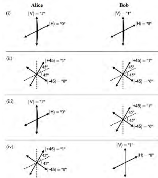
Figure 39.5: Communication between Alice and Bob using single-photon source and simplified polarizer measurement schemes (from DAB Miller [77]).
