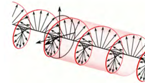
Figure 9.3: The rotation of the field vector of a right-hand circular polarization wave as it propagates in the right direction [86] (courtesy of Wikipedia).
