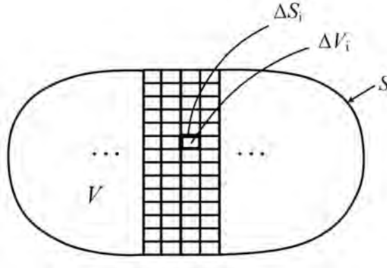
Figure 2.1: The discretization of a volume V into a sum of small volumes \Delta V_i each of which is a small cuboid. Stair-casing error occurs near the boundary of the volume V but the error diminishes as \Delta V_i \rightarrow 0 .
