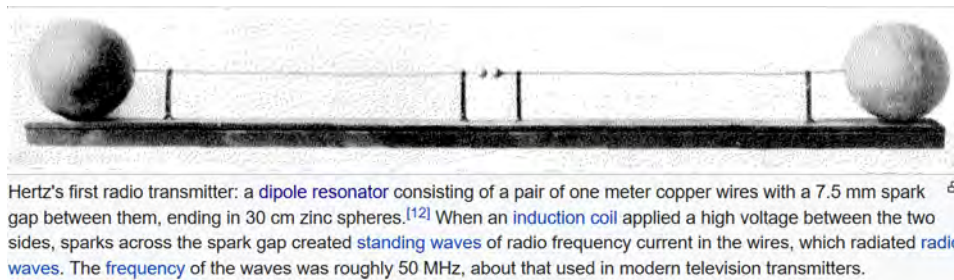
Figure 28.1: Hertz's original experiment on a small dipole (courtesy of Wikipedia [19]).
