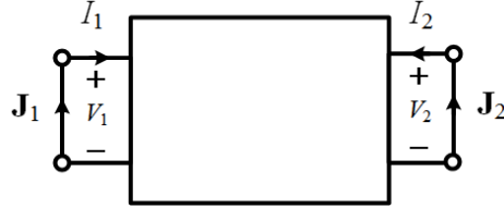
Figure 12.6: The interaction between two antennas in the far field of each other can be reduced to a circuit theory description since the input and output ports of the antennas are small compared to wavelength. But inside the box, any linear time invariant medium can be there.
