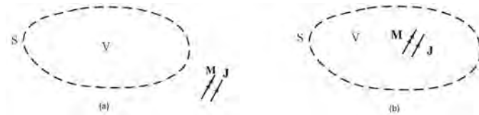
Figure 12.3: The geometry for proving reciprocity theorem when the surface S : (a) does not enclose the sources, and (b) encloses the sources. In the figure, the sources are supposed to be either (\mathbf{M}_1, \mathbf{J}_1) producing fields (\mathbf{E}_1, \mathbf{H}_1) or (\mathbf{M}_2, \mathbf{J}_2) producing fields (\mathbf{E}_2, \mathbf{H}_2) .
