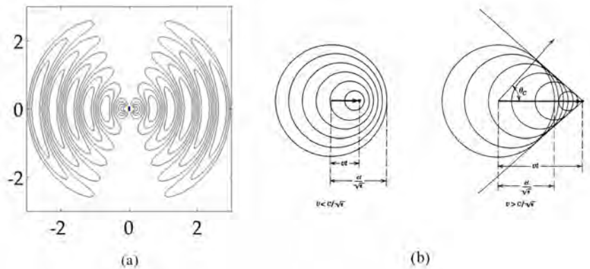
Figure 29.1: (a) Electric field around a time-oscillating dipole (courtesy of physics stack exchange). (b) Equipotential lines around a moving charge that gives rise to Cherenkov radiation (courtesy of J.D. Jackson [49]). We will not study Cherenkov (Cerenkov) radiation in this course, but it is written up in [49] and [34]. Its discovery and its explanation led to a Nobel Prize.
