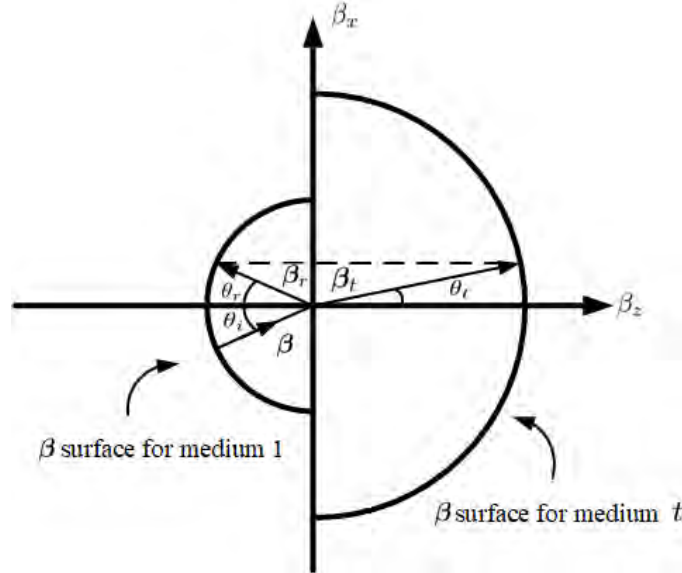
Figure 18.2: Wave-number ( \beta or k ) surfaces in two regions showing the phase matching condition. In this case, the wave number in medium t is larger (with larger \beta vector) than the wave number in medium 1. Then the wave vectors for the incident wave, reflected wave, and transmitted wave have to be aligned in such a way that their components parallel to the interface are equal because of the phase-matching condition. Also, one can see that Snell's law is satisfied as required by the phase-matching condition.
