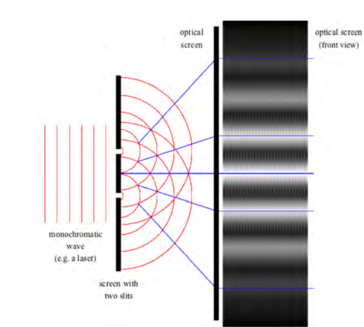
Figure 38.2: A Young's double-slit experiment. Again, the interference pattern reveals the wave nature of light (courtesy of [310]).
