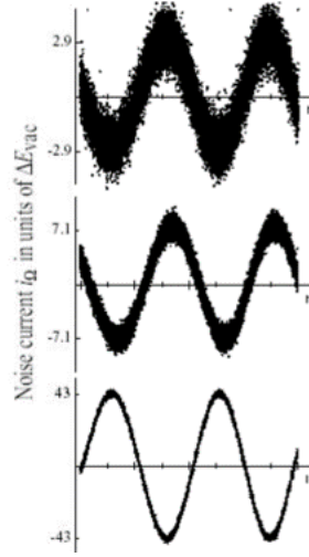
Figure 39.3: The time evolution of the coherent state at the very low signal level. It is sinusoidal, but with great uncertainty innate in it (courtesy of Wikipedia [335]).
