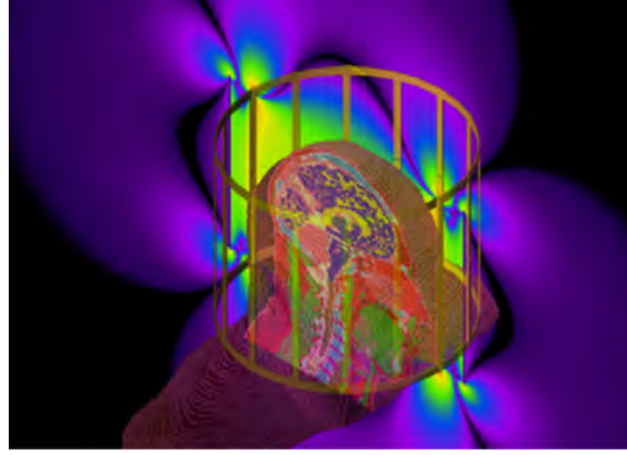
Figure 37.5: FDTD simulation of human head in a squirrel cage of an MRI (magnetic resonance imaging) system. A static magnetic field biases the spins in the human body. Then an RF field is used to tilt the spins causing them to precess. Their precession gives rise to electromagnetic radiation (also called spin echo) that can be measured by the squirrel cage coils (courtesy of REMCOM).
