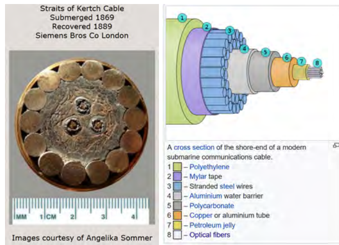
Figure 18.9: The picture of an old 1869 submarine cable made of coaxial cables (left), and modern submarine cable made of optical fibers (right) (courtesy of Atlantic-Cable [145], and Wikipedia [146]). Comparing them to the optical fiber now, we have come a long way!
