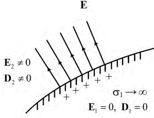
Figure 5.3: The behavior of the electric field and electric flux at the interface of a perfect electric conductor and free space (or air).
