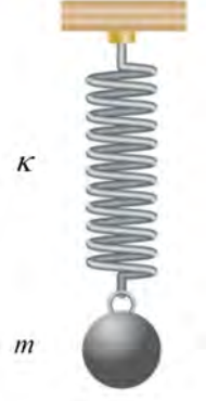
Figure 38.3: A classical pendulum can be used to illustrate classical Hamiltonian theory. The equation of motion of a classical pendulum can be derived using Newton's law or Hamiltonian theory. As such, it is easier to illustrate quantum theory of a pendulum starting with classical Hamiltonian theory. In the figure, \kappa and m are spring constant and mass, respectively of the pendulum (courtesy of pngwing.com).
