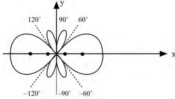
Figure 30.6: By changing the phase of the linear array, the radiation pattern of the antenna array can be changed to become an endfire array as shown.
