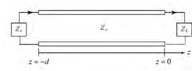
Figure 25.1: A simple ideal resonator is made by terminating a transmission line with two reactive loads at its two ends, the source end with Z_S and the load end with Z_L .
