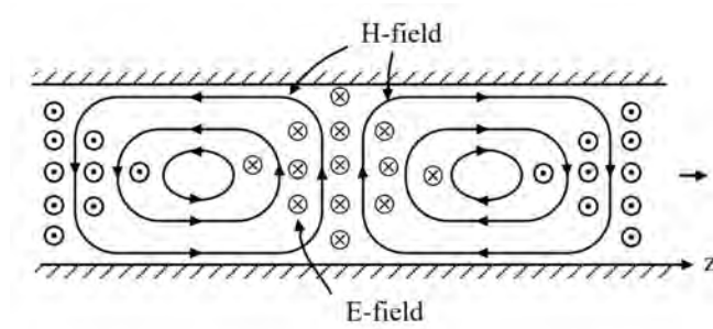
Figure 23.5: A snapshot of the field plot of a TE_{10} mode propagating in the z direction of a rectangular waveguide. Notice that the \mathbf{E} and \mathbf{H} fields do not exactly curl around each other because of the time delay.
