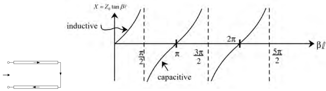
Figure 16.2: The input reactance ( X ) of a short-circuited transmission line as a function of its length l . The input impedance of the transmission line alternates between being inductive and capacitive as the length varies. A standing wave develops on this short-circuit terminated transmission line. This can make the input impedance look inductive or capacitive depending on if the input port is current or voltage dominated, respectively. Large current flow on a short-circuited line generating stored magnetic energy and hence, the impedance becomes inductive depending on the value of l .
