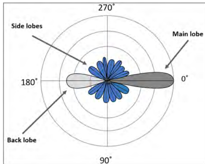
Figure 29.6: The directive gain pattern of an array antenna. The directivity is increased by constructive interference among the elements of the array antenna (courtesy of Wikipedia).
