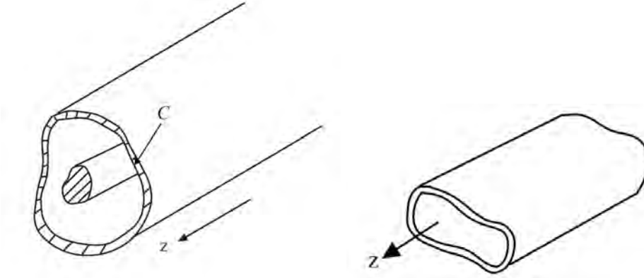
Figure 22.2: A hollow metallic waveguide with a center conductor (left), and without a center conductor (right).
