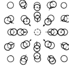
Fig. 8 The polaron . The electron (broken circle in the centre) displaces the ions of the polar crystal from their positions of equilibrium. This alters its effective mass.
