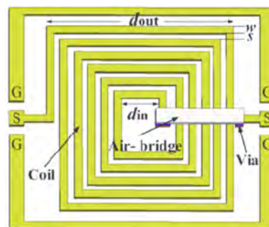
Figure 14.16: Spiral inductors are difficult to build on a chip, but by using laminal structure, it can be integrated into the IC fabrication process (courtesy of Quan Yuan, Research Gate). The fabrication of circuit components has to be commensurate with the photolithography and chemical processes used.
