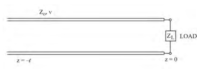
Figure 16.1: A schematic for a transmission line terminated with an impedance load Z_L at z = 0 .
