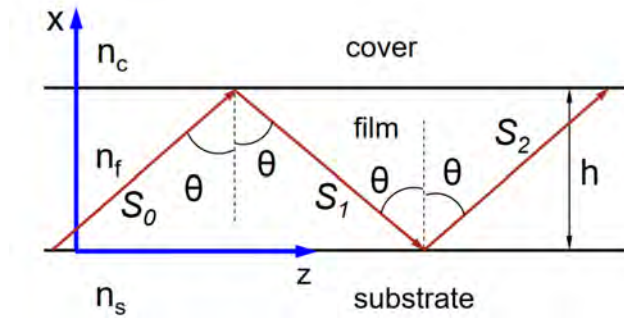
Figure 18.7: The total internal reflections (TIR) at the two interfaces of a thin-film waveguide can be used to guide an optical wave (courtesy of E.N. Glytsis, NTUA, Greece [143]).
