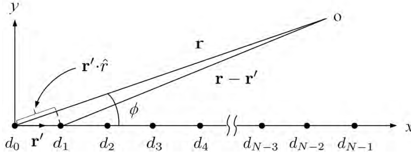
Figure 30.3: Schematic of a dipole array where the dipoles are aligned on the x axis, and we observe the field on the xy plane. To simplify the math, the far-field approximation can be used to find its far field or radiation field.
