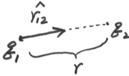
Figure 3: The force between two charges q_1 and q_2 . The force is repulsive if the two charges have the same sign.
