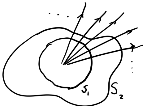
Figure 8: Same amount of electric flux from a point charge passes through two surfaces S_1 and S_2 .
