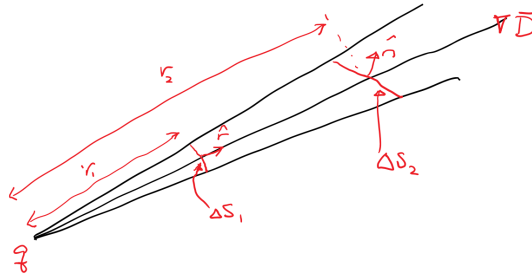
Figure 9: When a sliver of angular sector is taken, same amount of electric flux from a point charge passes through two incremental surfaces \Delta S_1 and \Delta S_2 .
