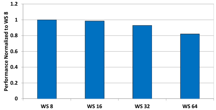
Fig. 14. Performance of Memcached at Various Wavefront Sizes (normalized to a warp size of 8)
