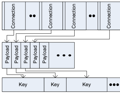
Fig. 5. Contiguous Memory Layout
