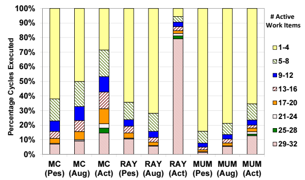
Fig. 10. SIMD Efficiency
