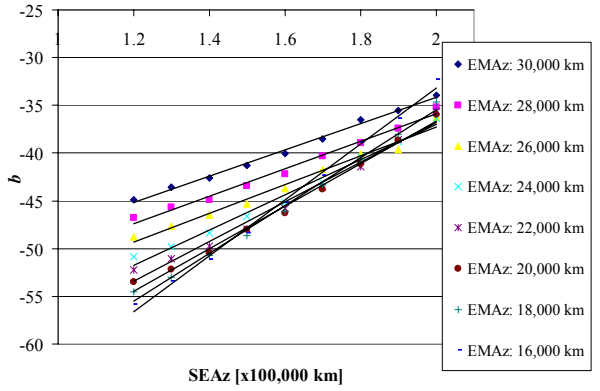
Fig. 14: Relationship between b and SEAz for each EMaZ.
