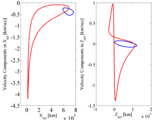
Fig. 7: Velocity vs. position at Poincaré Section; Earth-Moon manifolds (blue) and Sun-Earth manifolds (red).
