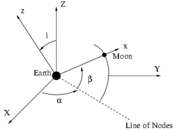
Fig. 1: Angle Definitions; X, Y, and Z define the Sun-Earth rotating frame; x, y, and z are fixed in the Earth-Moon rotating frame.
