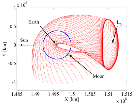
Fig. 2: Sun-Earth unstable manifolds near L_2 ; A_y=699,000 km, A_z=200,000 km.
