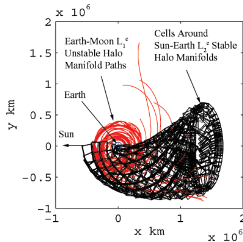
Fig. 17: EM manifolds intersect cells.
