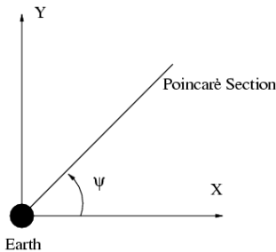
Fig. 5 : Definition of \psi .
