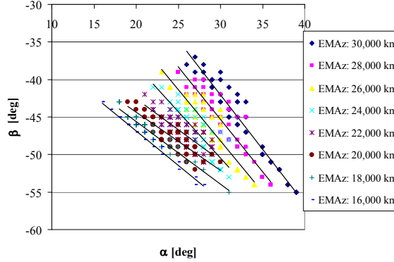
Fig. 16: Relationship between \alpha and \beta for SEAz = 200,000 km; various EMAz orbits.
