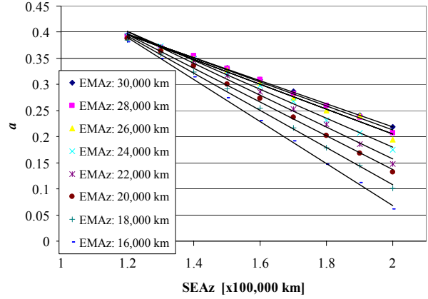
Fig. 13: Relationship between a and SEAz for each EMaZ.
