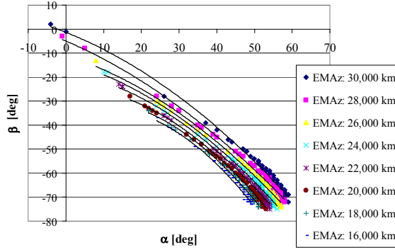
Fig. 15: Relationship between \alpha and \beta for SEAz = 120,000 km; various EMAz orbits.
