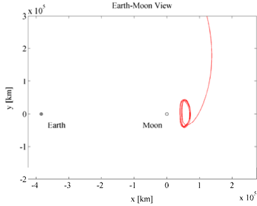
Fig. 11: Earth-Moon manifold asymptotically approaching an Earth-Moon Lissajous orbit.
