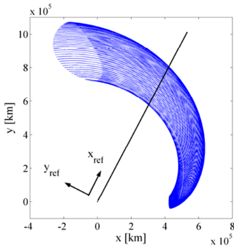
Fig. 8: New local PS_{EM} reference frame in Earth-Moon rotating frame.
