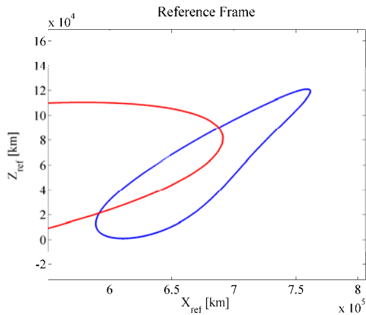
Fig. 6: EM manifolds (Blue) and SE manifolds (Red) in the PS reference frame.
