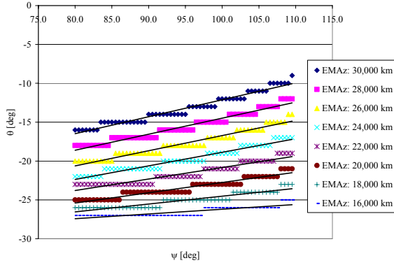
Fig. 12: Relationship between \theta and \psi ; SEAz = 200,000 km.
