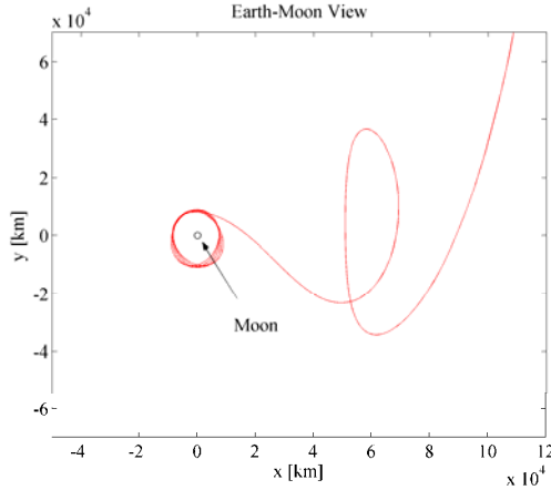
Fig. 20: Transfer to the Moon via a transit orbit; Earth-Moon A_z = 24,000 km; ephemeris model.
