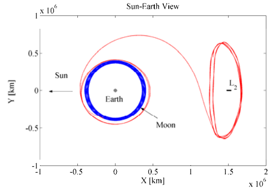
Figure 19: Lissajous-to-Moon transfer in the Sun-Earth rotating frame; ephemeris model.
