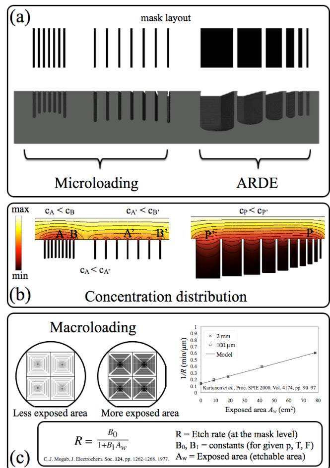
Figure 1: (a) Definition of microloading and ARDE. (b) Local consumption of the etching species leads to lower etchant concentration at feature-dense areas ( c_A < c_{A'} ) and higher etchant concentration at increasingly wider trenches ( c_P' > c_P ). (c) Etchant consumption and slow transport from regions faraway from the mask level leads to macroloading.
