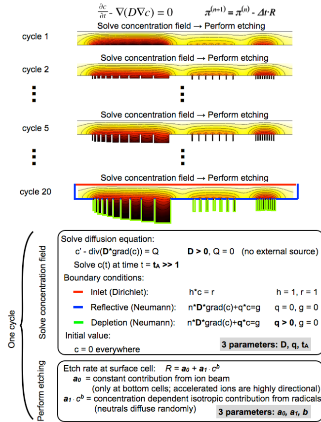
Figure 2: Proposed simulation procedure, consisting in solving the diffusion equation and performing etching at every Bosch cycle, according to the shown details. The diffusion equation for the concentration c is solved using a finite element method (FEM) continuum description while etching is simulated using a Cellular Automaton (CA).
