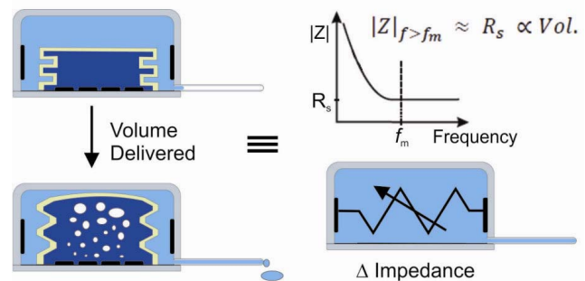
Figure 2: System operation concept.
