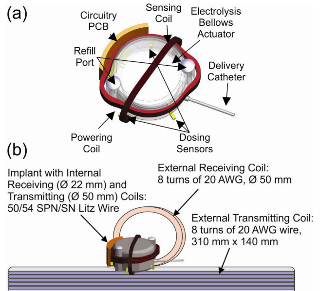
Figure 1: (a) Schematic diagram of wireless implantable drug delivery micropump with integrated dosing sensors, (b) system setup (not to scale): the micropump is placed on top of the external transmitting coil. The external coils are situated perpendicular to each other.
