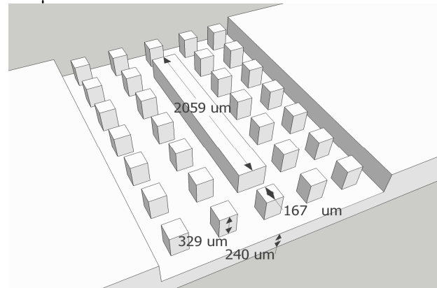
Figure 1: Schematic illustration of the gap waveguide resonator, displaying the dimensions and placements of the pin and the ridge.
