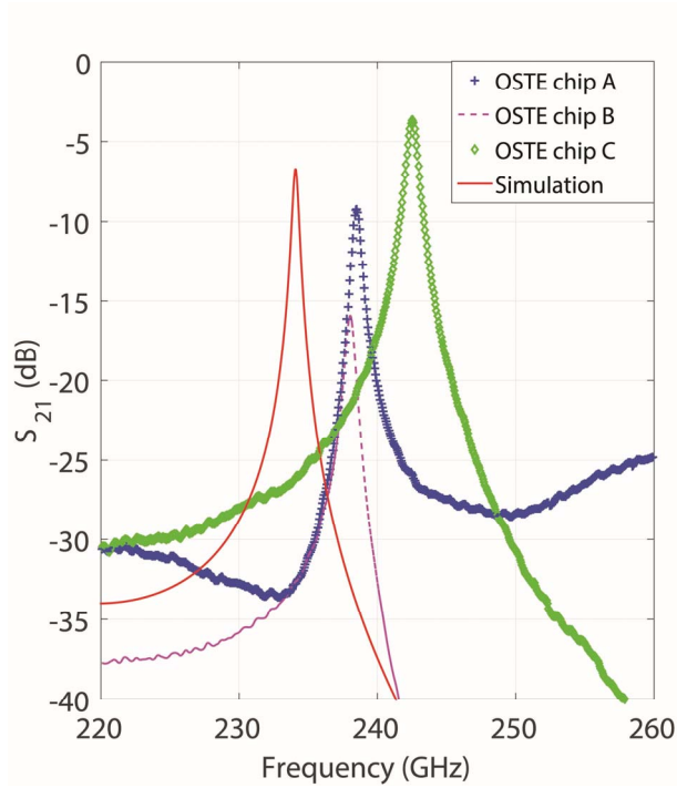
Figure 5: Measurements results of the three OSTE resonators and the simulations at 220-260 GHz
