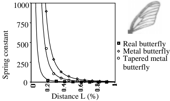
Figure 8: Spring constant of butterfly wings
