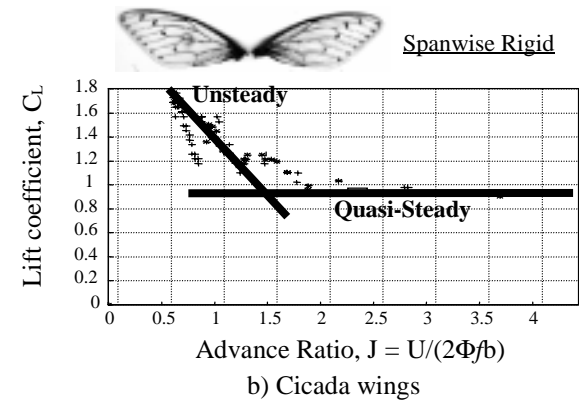
Figure 10: Spanwise stiffness effect
