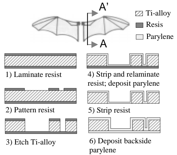
Figure 6: Fabrication process of titanium-alloy MEMS wings
