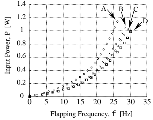
Figure 12: Input power
