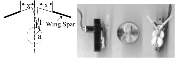
Figure 9: Transmission system
