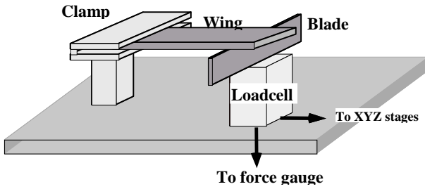
Figure 7: Spring constant test setup schematic
