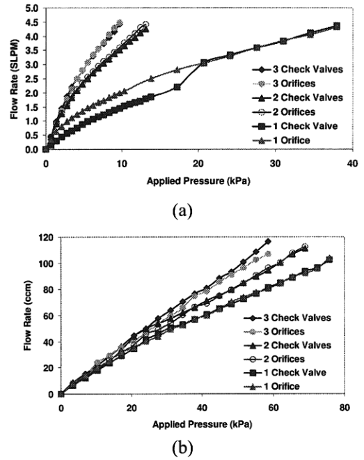
Figure 15: Flow Rate vs. Pressure in Check Valve Array for (a) Air & (b) Water
