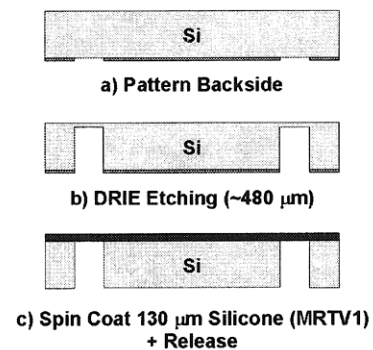
Figure 6: Bossed Silicone Membrane Process Flow
