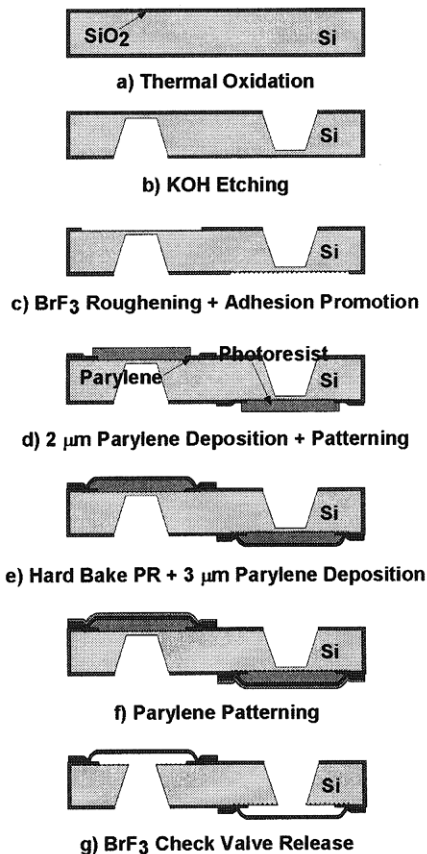
Figure 3: Double-Sided Check Valve Process Flow
