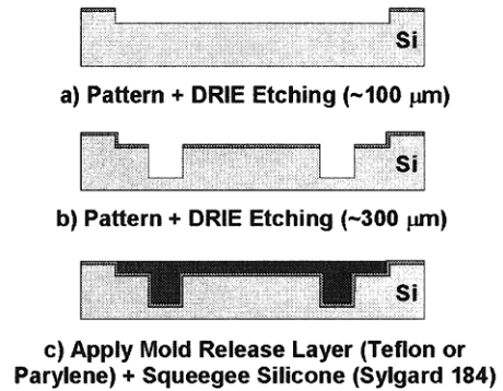
Figure 11: Silicon Gasket Process Flow
