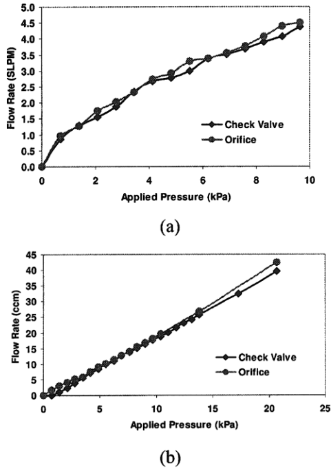
Figure 14: Flow Rate vs. Applied Pressure Plots for (a) Air & (b) Water
