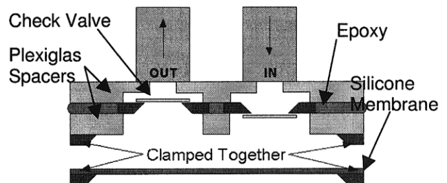
Figure 1: 2D Cross Section of 1st Generation Pump
