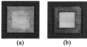
Figure 7: KOH Etched Silicone Membrane
