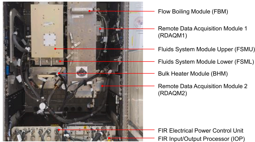
Fig. 1. Photograph of FBCE modules installed into the Fluid Integrated Rack on the ISS.
