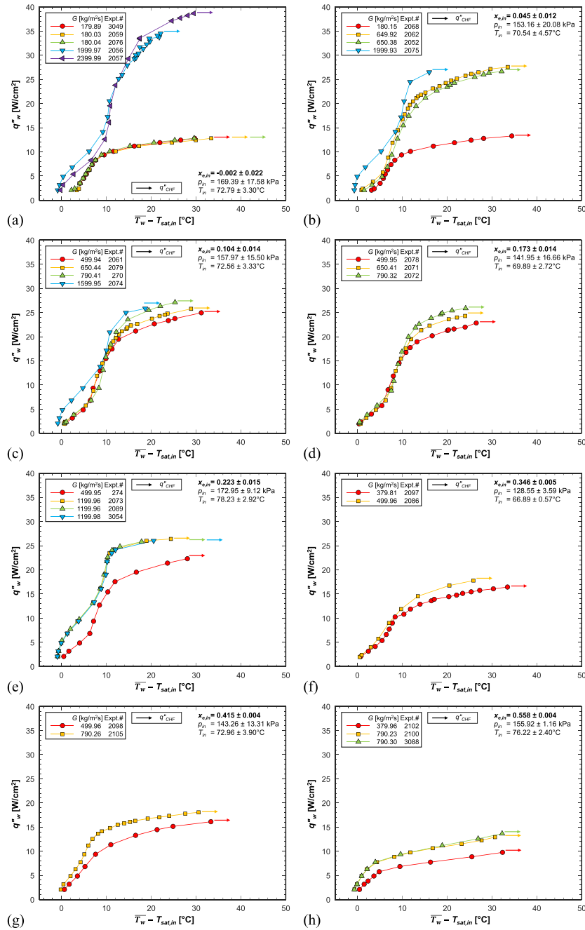
Fig. G.1. Microgravity flow boiling curves for two-phase inlet with double-sided heating, showing the effects of mass velocity at various fixed inlet qualities of x_{e,in} = (a) -0.002, (b) 0.045, (c) 0.104, (d) 0.173, (e) 0.223, (f) 0.346, (g) 0.415, and (h) 0.558.
