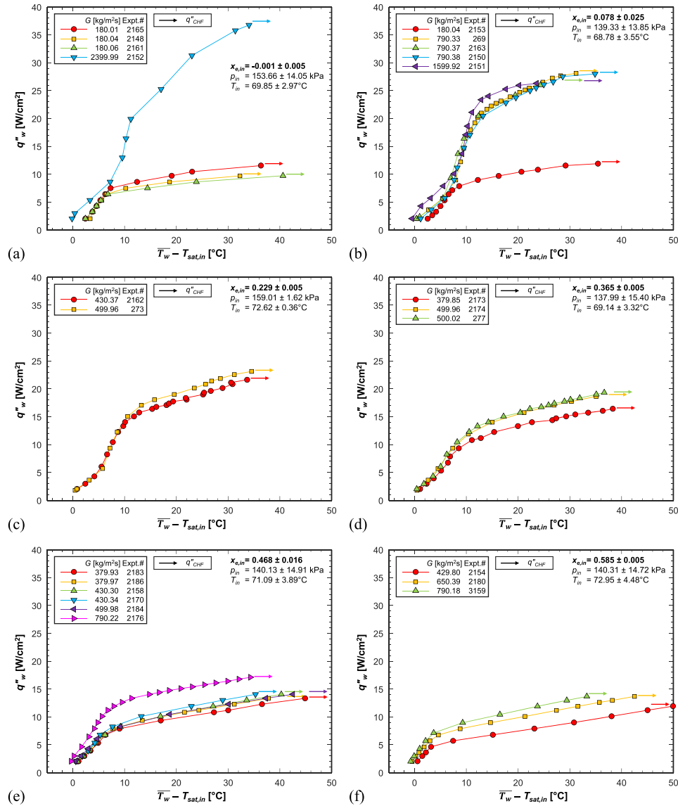
Fig. 25. Microgravity flow boiling curves for two-phase inlet with single-sided heating, showing the effects of mass velocity at various fixed inlet qualities of x_{e,in} = (a) -0.001, (b) 0.078, (c) 0.229, (d) 0.365, (e) 0.468, and (f) 0.585.
