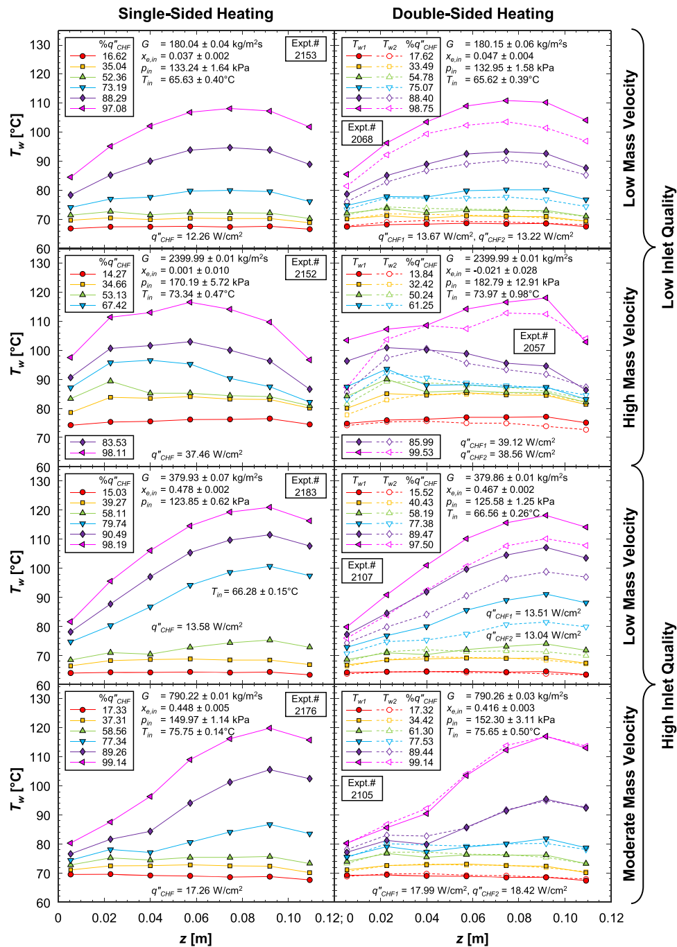
Fig. 27. Streamwise profiles of local wall temperature ( T_w versus z ) for different heat fluxes ( q''_w ) at a variety of inlet conditions with single- and double-sided heating.
