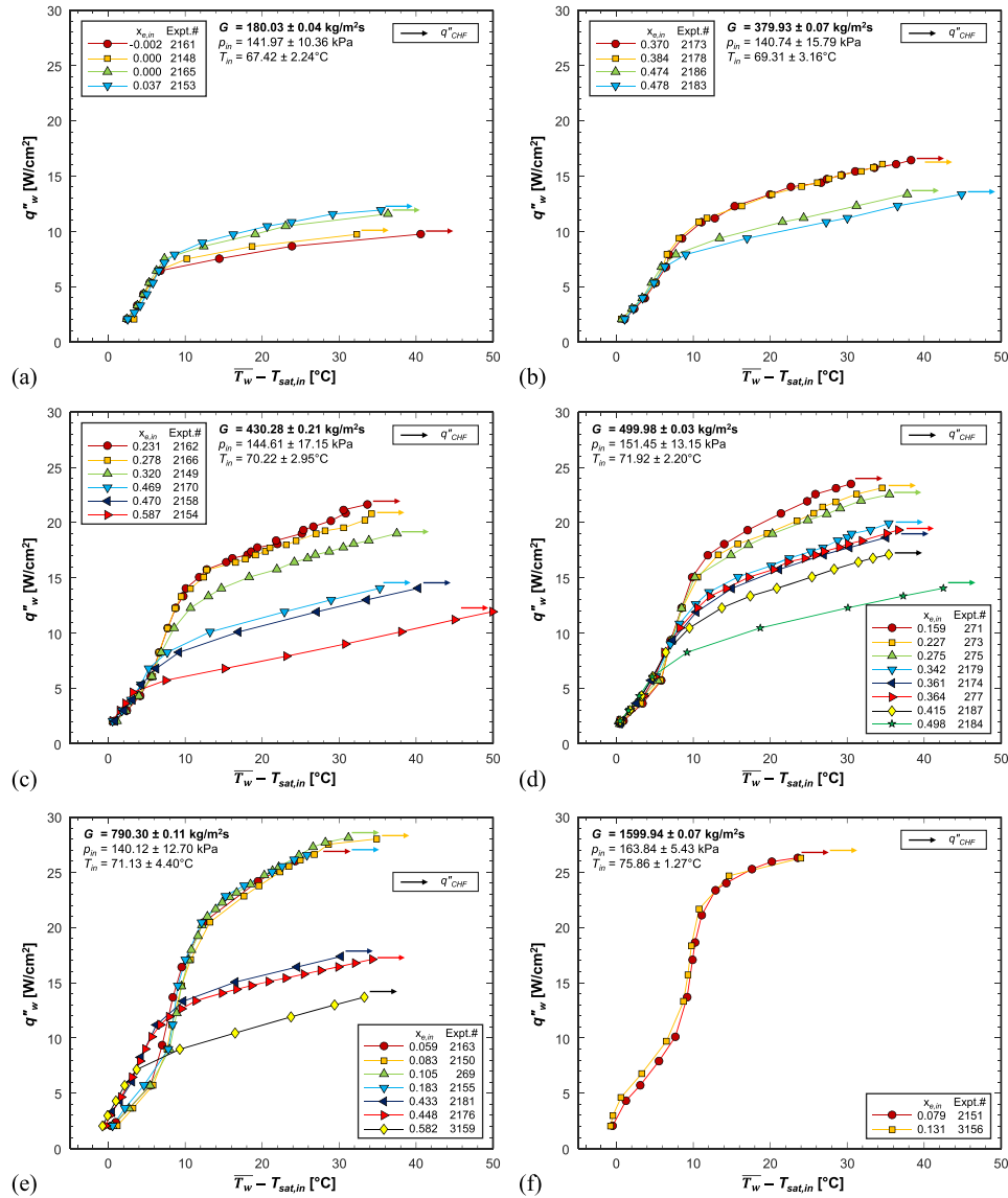
Fig. 26. Microgravity flow boiling curves for two-phase inlet with single-sided heating, showing the effects of inlet quality at various fixed mass velocities of G \approx (a) 180, (b) 380, (c) 430, (d) 500, (e) 790, and (f) 1600 kg/m 2 s.
