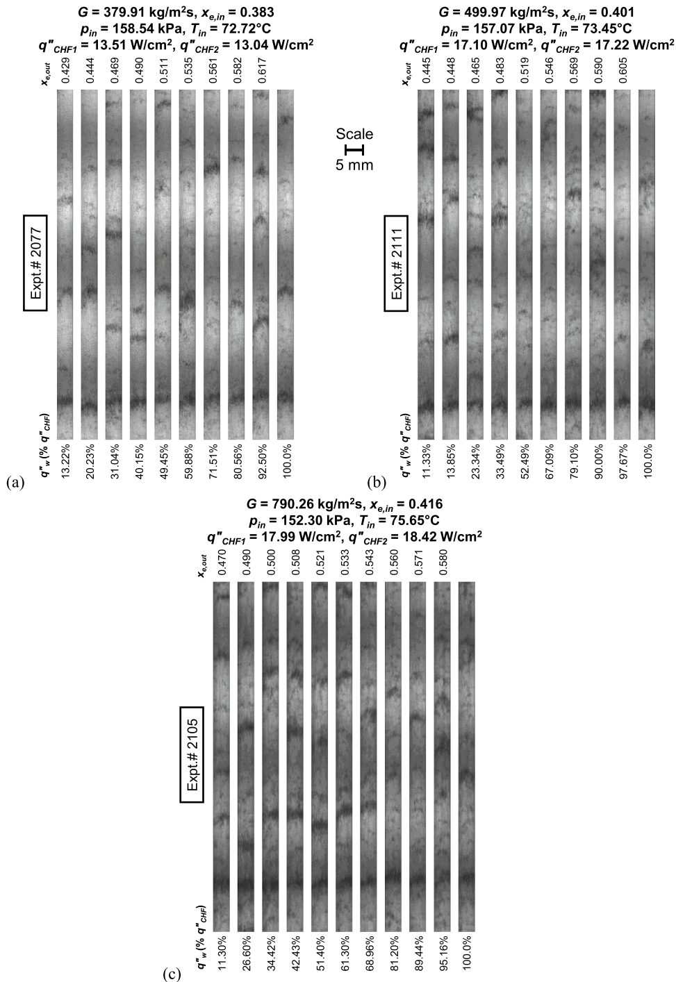
Fig. E.1. Flow patterns for increasing heat fluxes until CHF for double-sided heating at a fixed high inlet quality of x_{e,in} \approx 0.400 but different mass velocities of G \approx (a) 380, (b) 500, and (c) 790 \text{kg/m}^2\text{s} . Channel width is 5 mm.
