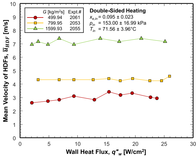
Fig. 23. Variations of mean velocity of HDFs along the channel versus wall heat flux until CHF with double-sided heating for different mass velocities. The time instants of HDF measurement correspond to the average flow pattern images shown in Fig. 22.
