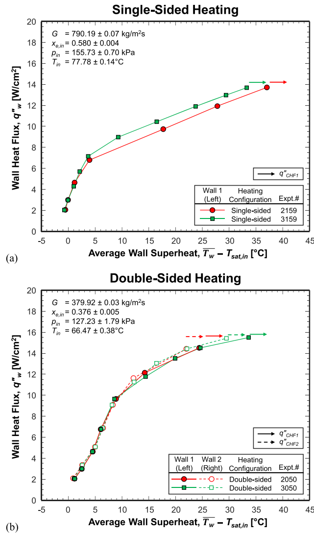
Fig. F.1. Boiling curves showing heat transfer symmetry and repeatability in microgravity flow boiling experiments for both (a) single- and (b) double-sided heating with two-phase inlet.
