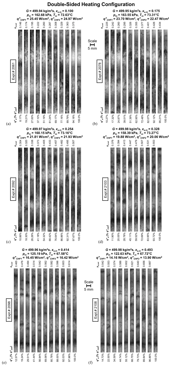
Fig. 18. Flow patterns for increasing heat fluxes until CHF for double-sided heating at a fixed mass velocity of G \approx 500 \text{ kg/m}^2\text{s} but different inlet qualities of x_{e,in} = (a) 0.100, (b) 0.175, (c) 0.254, (d) 0.328, (e) 0.414, and (f) 0.493. Channel width is 5 mm.
