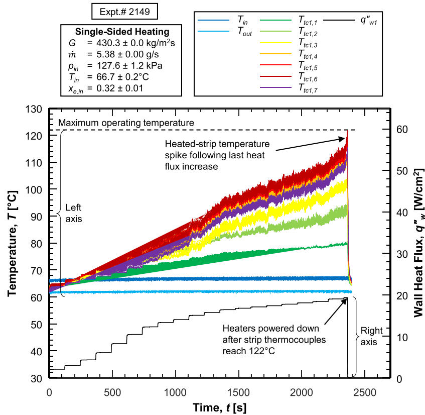
Fig. B.1. Temporal variations of fluid inlet ( T_{in} ), fluid outlet ( T_{out} ), and heating-strip temperatures ( T_{tc} ) for heat flux ( q''_w ) increments from a minimum until CHF for a typical experimental case with the following mean operating conditions: mass velocity of G = 430.3 \text{ kg/m}^2\text{s} , mass flow rate of \dot{m} = 5.38 \text{ g/s} , inlet pressure of p_{in} = 127.6 \text{ kPa} , fluid inlet temperature of T_{in} = 66.7^\circ\text{C} , and inlet quality of x_{e,in} = 0.32 .
