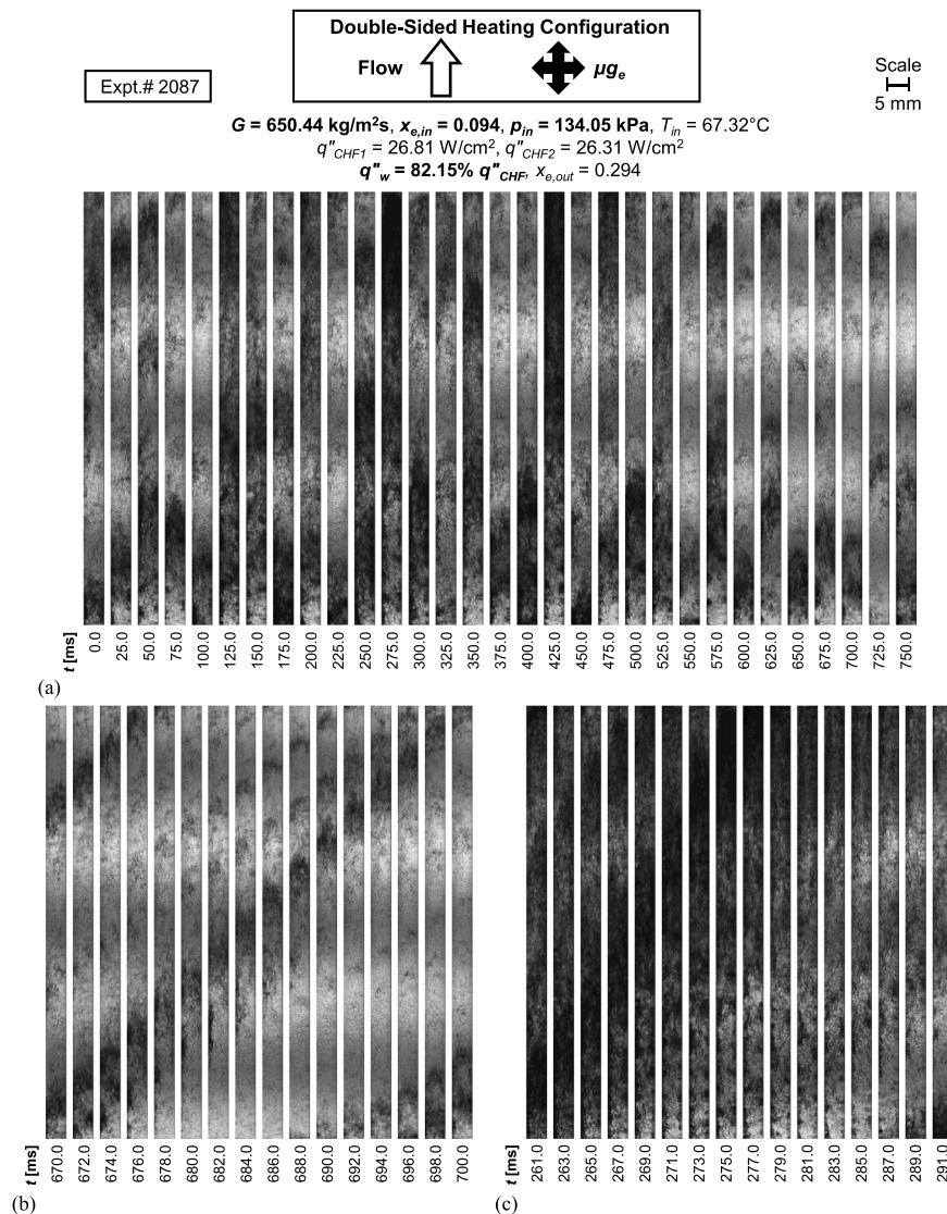
Fig. 17. Flow visualization image sequences for double-sided heating with mass velocity of G \approx 650 \text{ kg/m}^2\text{s} , inlet quality of x_{e,in} = 0.094 , and wall heat flux of q''_w = 82.15\% q''_{CHF} . Shown are (a) the overall transient behavior over an extended time period (25 ms between images), (b) low-density-dominant period (2 ms between images), and (c) high-density-dominant period (2 ms between images). Channel width is 5 mm.
