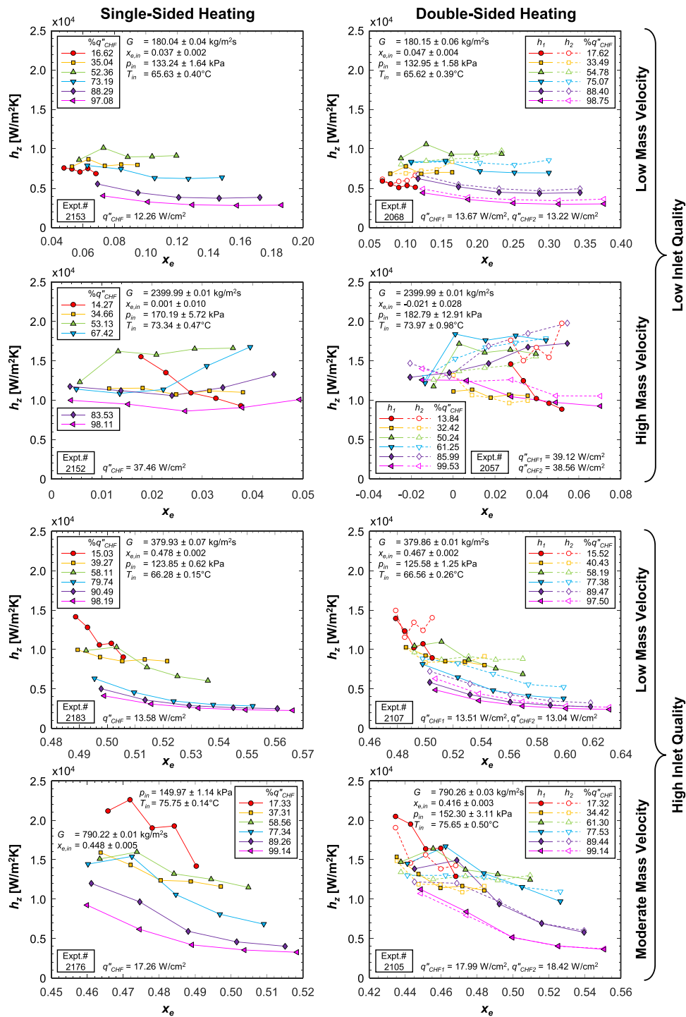
Fig. 29. Variations of local heat transfer coefficient at each heated wall, h_z , versus local thermodynamic equilibrium quality, x_{e,in} , for different heat fluxes, q''_w , with single- and double-sided heating at a variety of inlet conditions.
