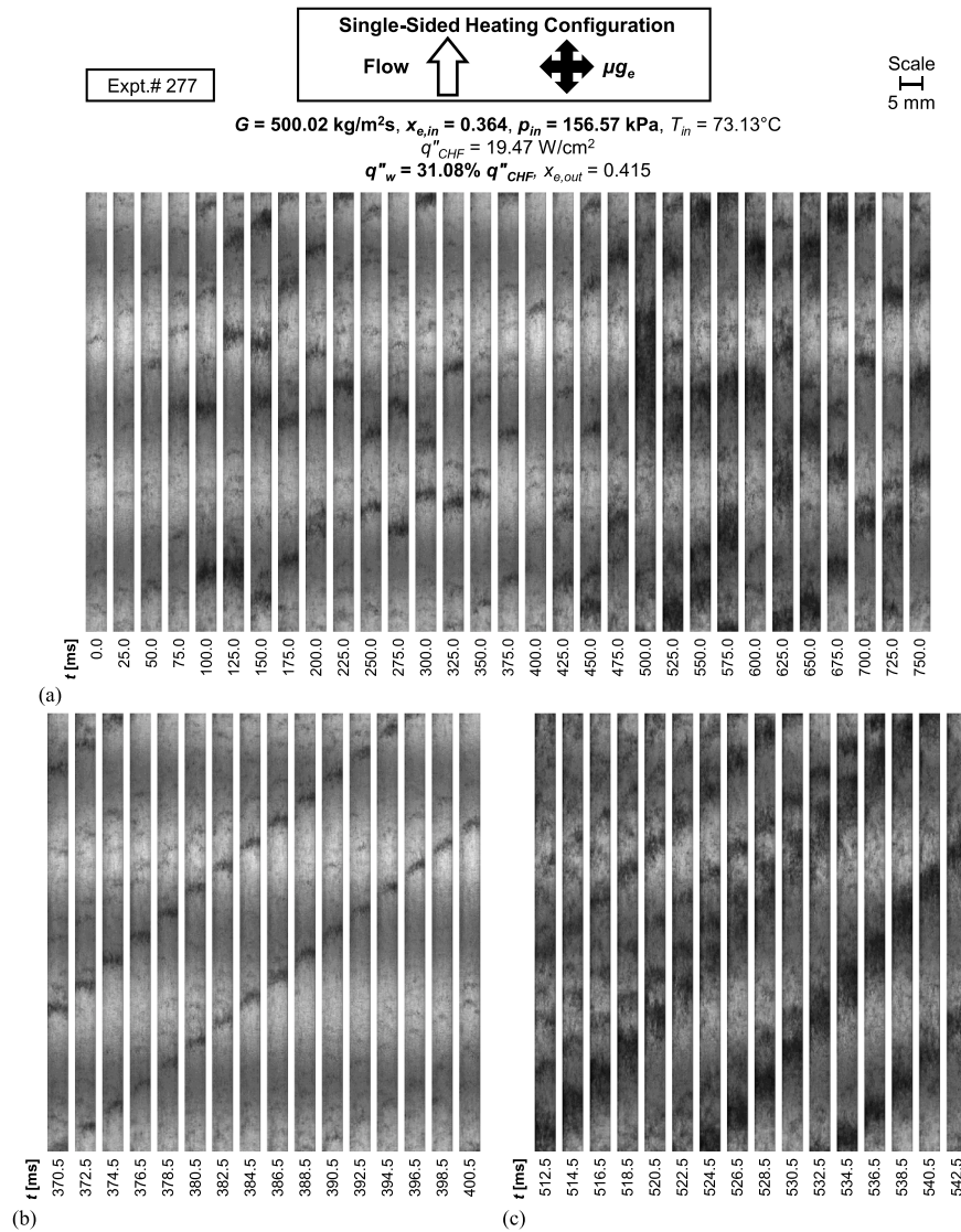
Fig. 7. Flow visualization image sequences for single-sided heating of left wall with mass velocity of G \approx 500 \text{ kg/m}^2\text{s} , inlet quality of x_{e,in} = 0.364 , and wall heat flux of q''_w = 31.08\% q''_{CHF} . Shown are (a) the overall transient behavior over an extended time period (25 ms between images), (b) low-density-dominant period (2 ms between images), and (c) high-density-dominant period (2 ms between images). Channel width is 5 mm.
