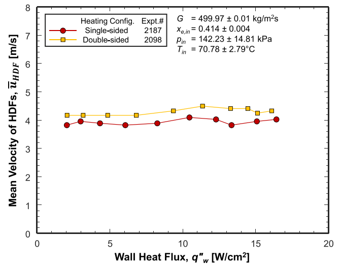
Fig. 21. Variations of mean velocity of HDFs along the channel versus wall heat flux until CHF with single- and double-sided heating at near-identical mass velocity and inlet quality. The time instants of HDF measurement correspond to the average flow pattern images shown in Figs. 18(e) and 20(d).
