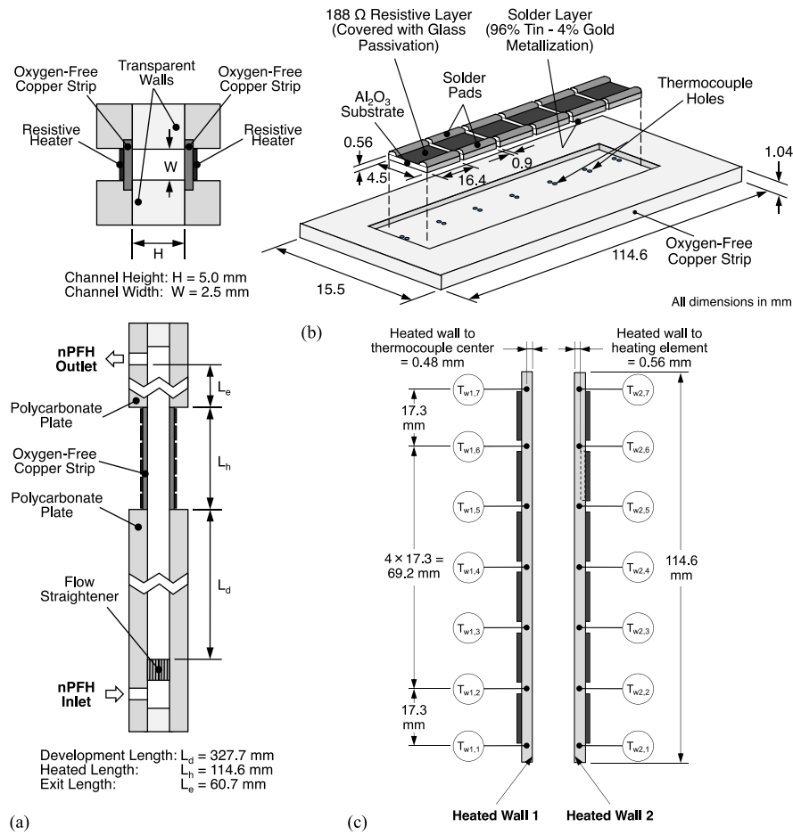
Fig. 3. Schematics of (a) overall construction of Flow Boiling Module (FBM), (b) construction of heating strips, and (c) designation of heated walls and local wall temperatures. Adapted from the authors' prior study [19].
