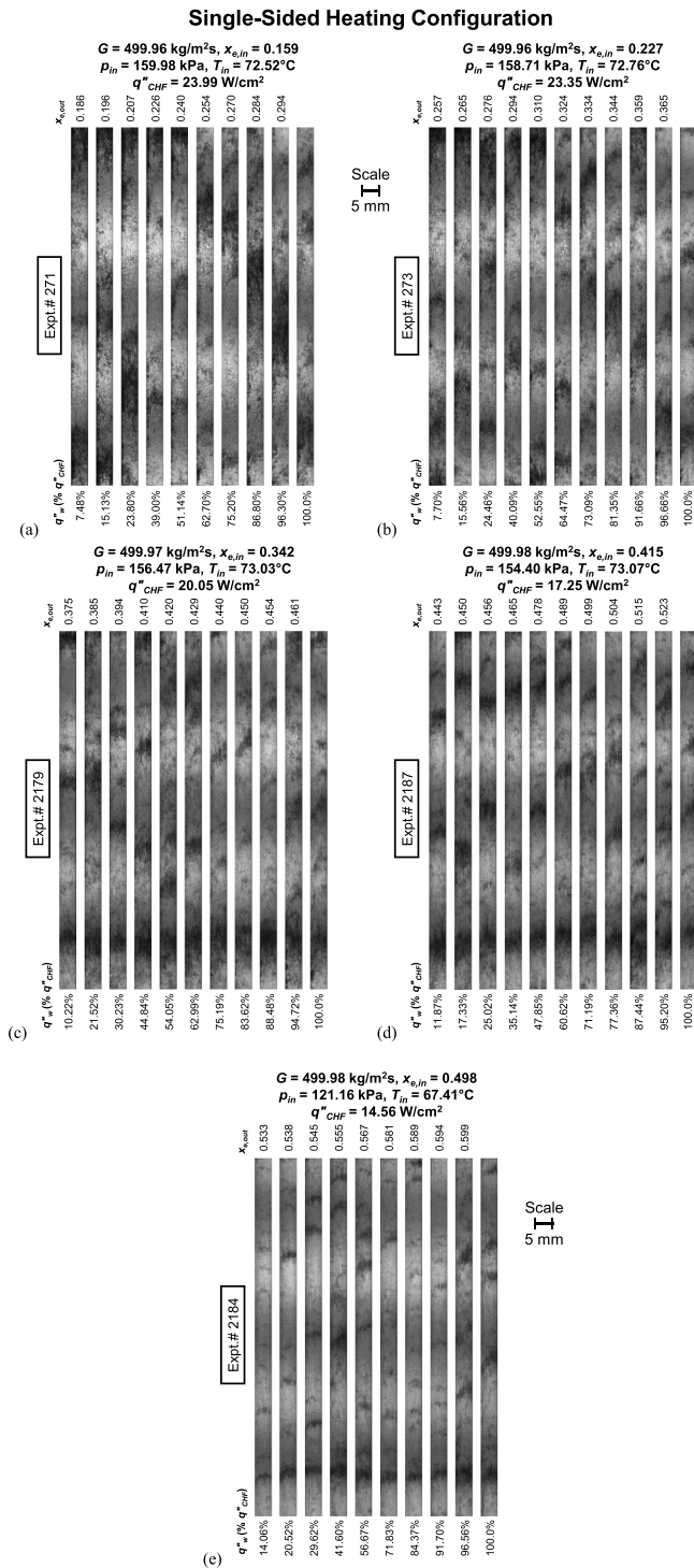
Fig. 20. Flow patterns for increasing heat fluxes until CHF for single-sided heating of left wall at a fixed mass velocity of G \approx 500 \text{ kg/m}^2\text{s} but different inlet qualities of x_{e,in} = (a) 0.159, (b) 0.227, (c) 0.342, (d) 0.415, and (e) 0.498. Channel width is 5 mm.
