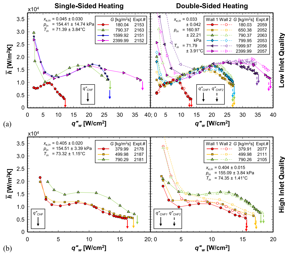
Fig. 31. Variations of average heat transfer coefficient, \bar{h} , versus wall heat flux, q''_w , for different mass velocities, G , with single- and double-sided heating at (a) low and (b) high inlet qualities, x_{e,in} .
