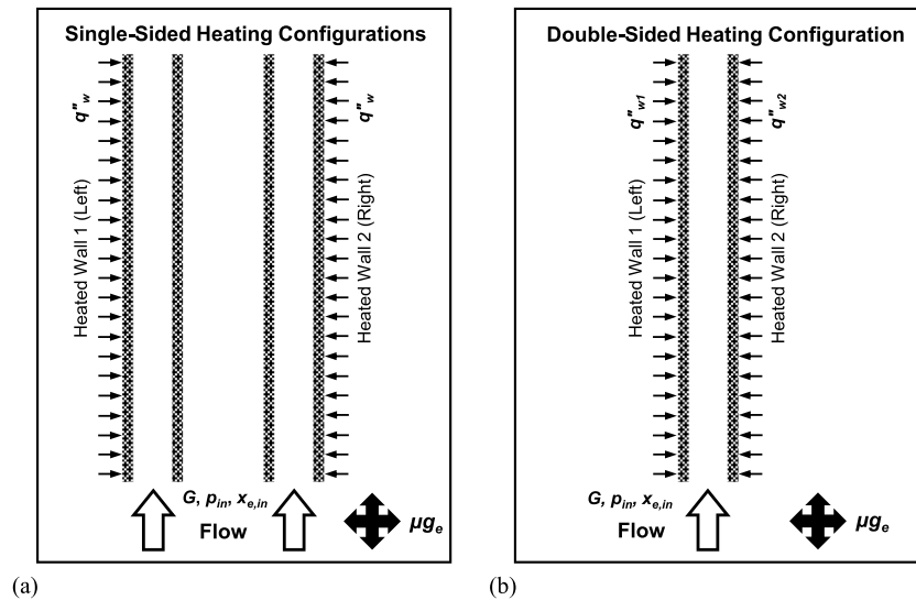
Fig. 4. Schematics of (a) single- and (b) double-sided heating configurations. A liquid-vapor mixture of nPFH enters the channel at the specified mass velocity of G , inlet pressure of p_{in} , and inlet quality of x_{e,in} while the walls are heated with a heat flux of q''_w . Adapted from the authors' prior study [19,32].
