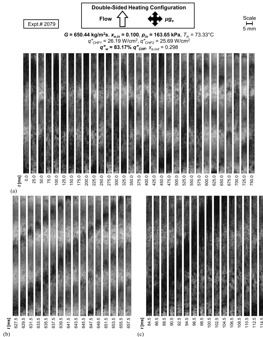
Fig. 14. Flow visualization image sequences for double-sided heating with mass velocity of G \approx 650 \text{ kg/m}^2\text{s} , inlet quality of x_{e,in} = 0.100 , and wall heat flux of q''_w = 83.17\% q''_{CHF} . Shown are (a) the overall transient behavior over an extended time period (25 ms between images), (b) low-density-dominant period (2 ms between images), and (c) high-density-dominant period (2 ms between images). Channel width is 5 mm.
