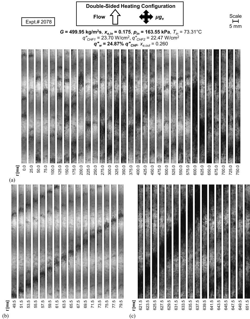
Fig. D.1. Flow visualization image sequences for double-sided heating with mass velocity of G \approx 500 \text{ kg/m}^2\text{s} , inlet quality of x_{e,in} = 0.175 , and wall heat flux of q''_w = 24.87\% q''_{CHF} . Shown are (a) the overall transient behavior over an extended time period (25 ms between images), (b) low-density-dominant period (2 ms between images), and (c) high-density-dominant period (2 ms between images). Channel width is 5 mm.
