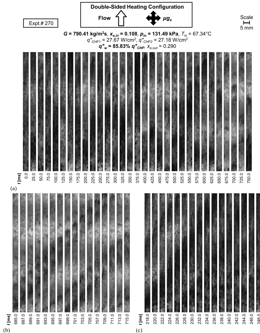
Fig. 15. Flow visualization image sequences for double-sided heating with mass velocity of G \approx 790 \text{ kg/m}^2\text{s} , inlet quality of x_{e,in} = 0.108 , and wall heat flux of q''_w = 85.83\% q''_{CHF} . Shown are (a) the overall transient behavior over an extended time period (25 ms between images), (b) low-density-dominant period (2 ms between images), and (c) high-density-dominant period (2 ms between images). Channel width is 5 mm.
