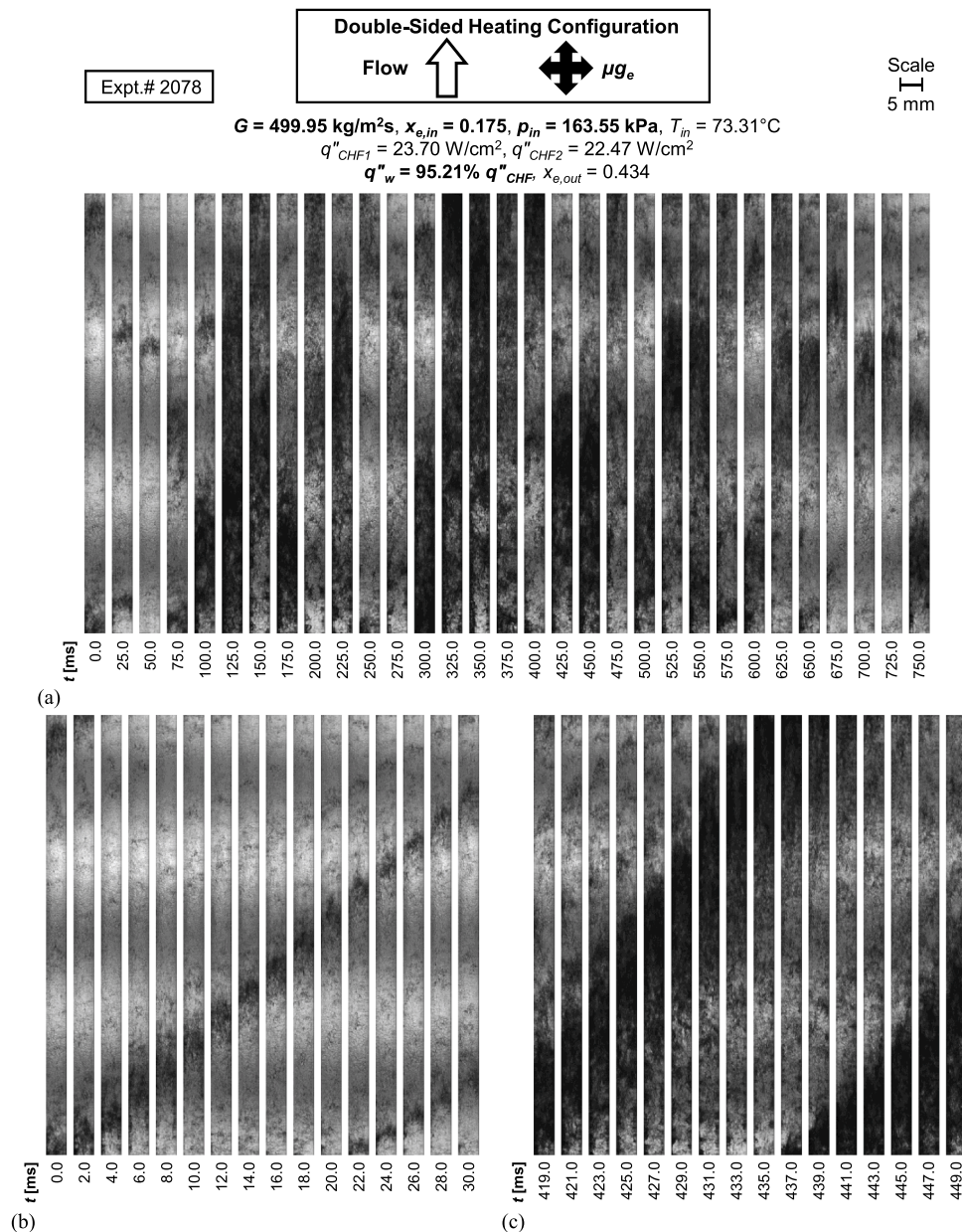
Fig. D.2. Flow visualization image sequences for double-sided heating with mass velocity of G \approx 500 \text{ kg/m}^2\text{s} , inlet quality of x_{e,in} = 0.175 , and wall heat flux of q''_w = 95.21\% q''_{CHF} . Shown are (a) the overall transient behavior over an extended time period (25 ms between images), (b) low-density-dominant period (2 ms between images), and (c) high-density-dominant period (2 ms between images). Channel width is 5 mm.
