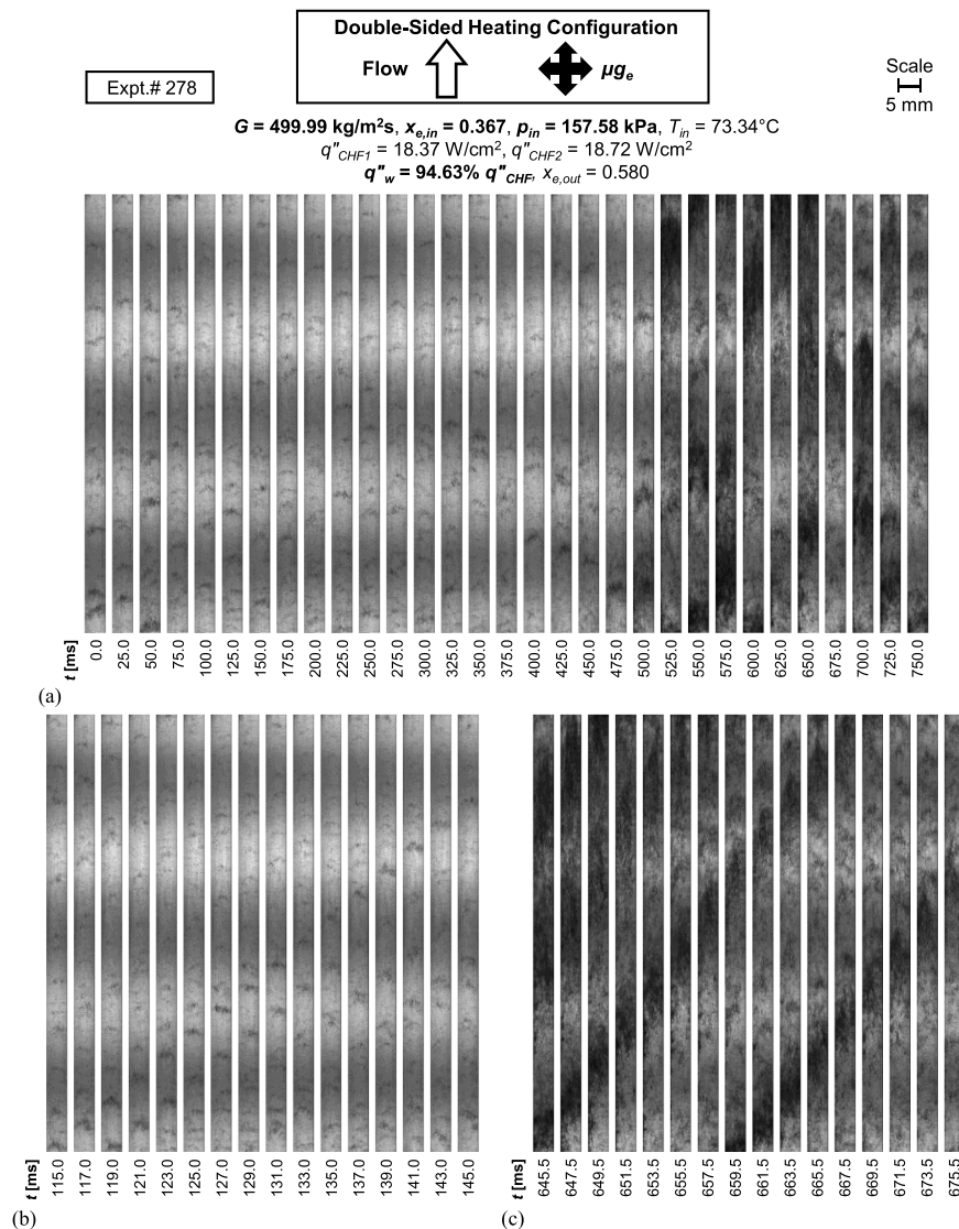
Fig. 10. Flow visualization image sequences for double-sided heating with mass velocity of G \approx 500 \text{ kg/m}^2\text{s} , inlet quality of x_{e,in} = 0.367 , and wall heat flux of q''_w = 94.63\% q''_{CHF} . Shown are (a) the overall transient behavior over an extended time period (25 ms between images), (b) low-density-dominant period (2 ms between images), and (c) high-density-dominant period (2 ms between images). Channel width is 5 mm.
