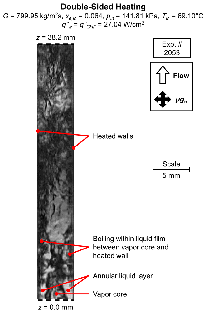
Fig. 5. Flow features in the channel's upstream region as distinct annular flow enters the channel for double-sided heating with a mass velocity of G \approx 800 \text{ kg/m}^2\text{s} and inlet quality of x_{e,in} = 0.064 . Channel width is 5 mm.
