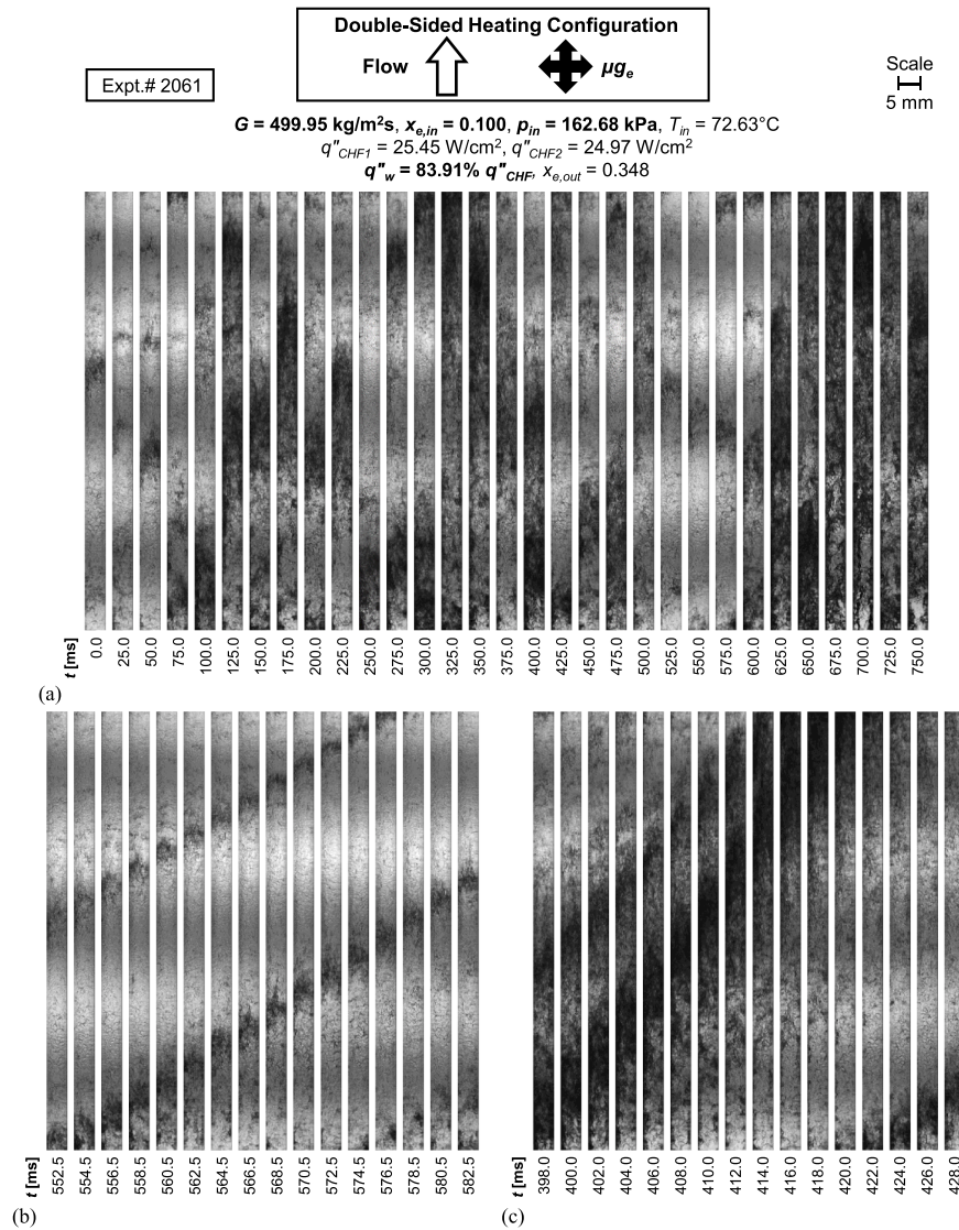
Fig. 13. Flow visualization image sequences for double-sided heating with mass velocity of G \approx 500 \text{ kg/m}^2\text{s} , inlet quality of x_{e,in} = 0.100 , and wall heat flux of q''_w = 83.91\% q''_{CHF} . Shown are (a) the overall transient behavior over an extended time period (25 ms between images), (b) low-density-dominant period (2 ms between images), and (c) high-density-dominant period (2 ms between images). Channel width is 5 mm.
