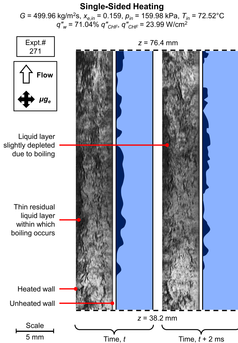
Fig. 6. Flow features in the channel's middle portion showing a liquid layer sliding along the heated wall. This is accompanied by interpreted contours of the liquid and vapor phases. Operating conditions are noted above the images. Time interval between successive images is 2 ms and channel width is 5 mm.
