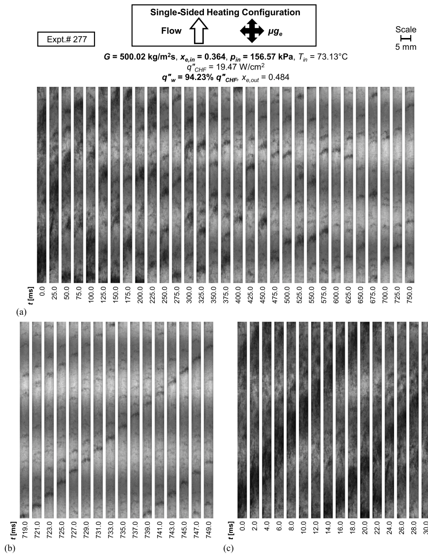
Fig. 8. Flow visualization image sequences for single-sided heating of left wall with mass velocity of G \approx 500 \text{ kg/m}^2\text{s} , inlet quality of x_{e,in} = 0.364 , and wall heat flux of q''_w = 94.23\% q''_{CHF} . Shown are (a) the overall transient behavior over an extended time period (25 ms between images), (b) low-density-dominant period (2 ms between images), and (c) high-density-dominant period (2 ms between images). Channel width is 5 mm.
