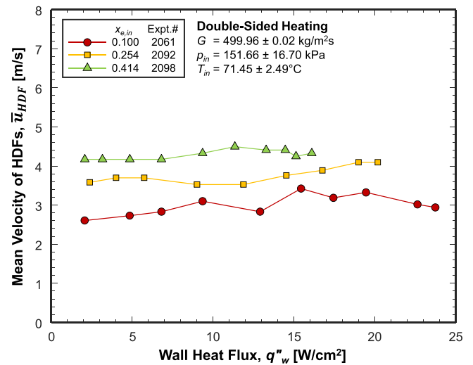
Fig. 19. Variations of mean velocity of HDFs along the channel versus wall heat flux until CHF with double-sided heating for different inlet qualities. The time instants of HDF measurement correspond to the average flow pattern images shown in Fig. 18.
