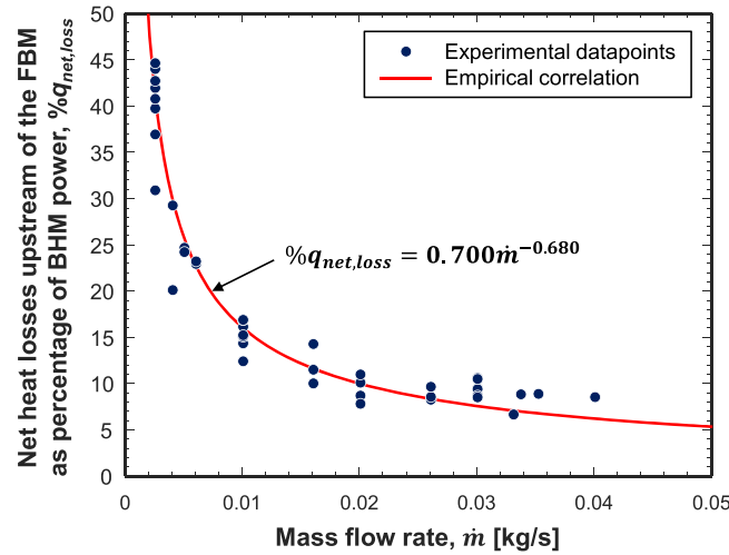
Fig. C.1. Heat loss correlation for experimental datapoints of heat loss for near-saturated inlet cases with no bubbles within the channel’s heated section.
