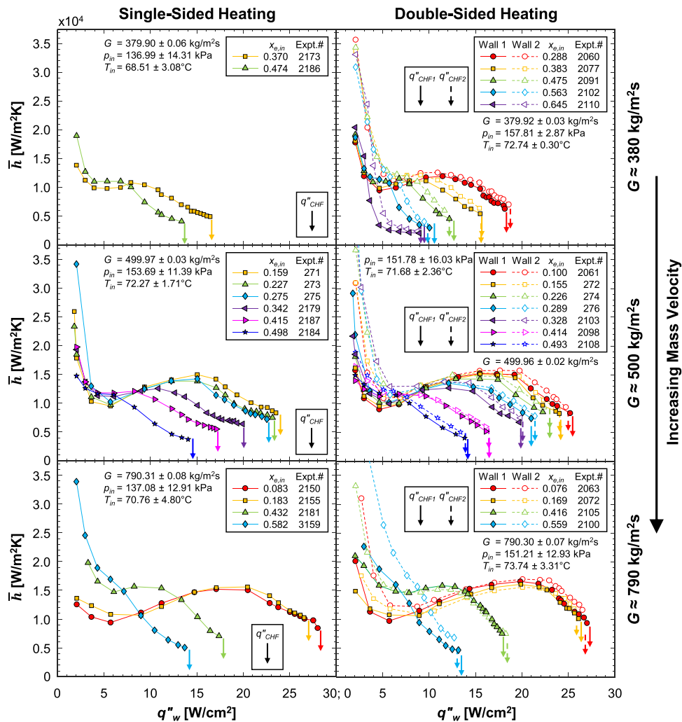
Fig. 30. Variations of average heat transfer coefficient, \bar{h} , versus wall heat flux, q''_w , for different inlet qualities, x_{e,in} , at six combinations of operating conditions and heating configuration: mass velocity, G , is increasing from the top to bottom plot, and single- and double-sided heating are respectively on the left and right.
