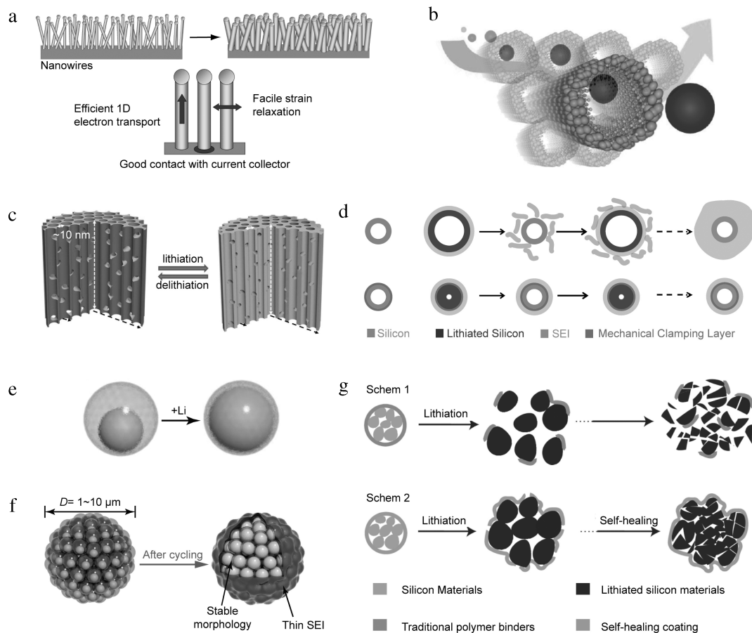
Fig. 3. Schematics showing the materials design to address the mechanical issues. (a) Si nanowires with good contact with current collector to avoid pulverization during cycling [47]. (b) Si nanotubes with hollow space to accommodate volume expansion [48]. (c) Si sponge with interconnected mesopores for tolerating volume expansion [49]. (d) Double-walled Si nanotubes with mechanically strong outer shells to prevent outward expansion and thus form stable SEI [51]. (e) A yolk-shell design that leaves void space within carbon shells to accommodate volume change [52]. (f) A pomegranate-like structure that significantly reduces the surface area and increases the packing density of nanostructures, which enables reduced side reactions and highly improved tap density [53]. (g) Schematic showing the self-healing polymer coating on the surface of Si microparticles, which can cure the breaks and guarantee good electrical contact with all wrapped Si even after pulverization [54].
