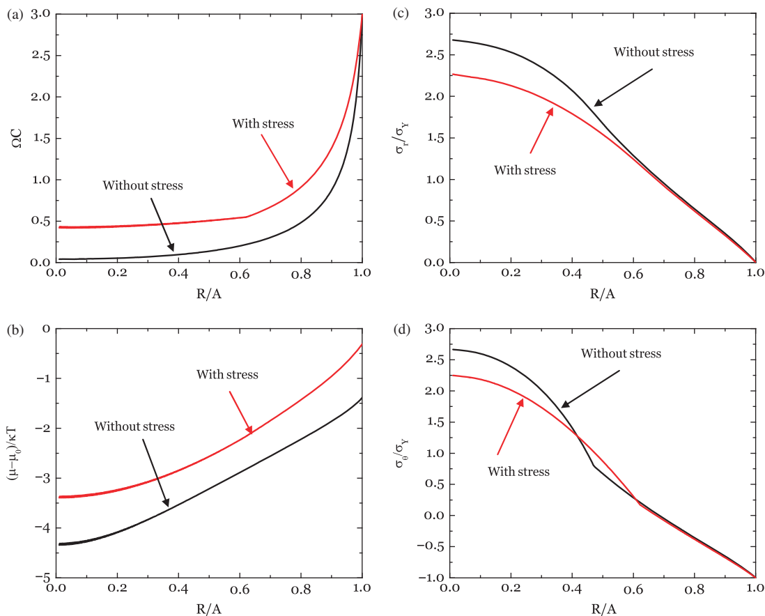
Fig. 6. Fields calculated with or without including the mean stress in the expression of the chemical potential of lithium are compared: (a) concentration of lithium, (b) chemical potential of lithium, (c) radial stress, and (d) hoop stress. The charging rate is \tau = 1 h, and both fields are given at the end of charge time, i.e., Dt/A^2 = 0.132 with stress calculation, Dt/A^2 = 0.009 without stress calculation.
