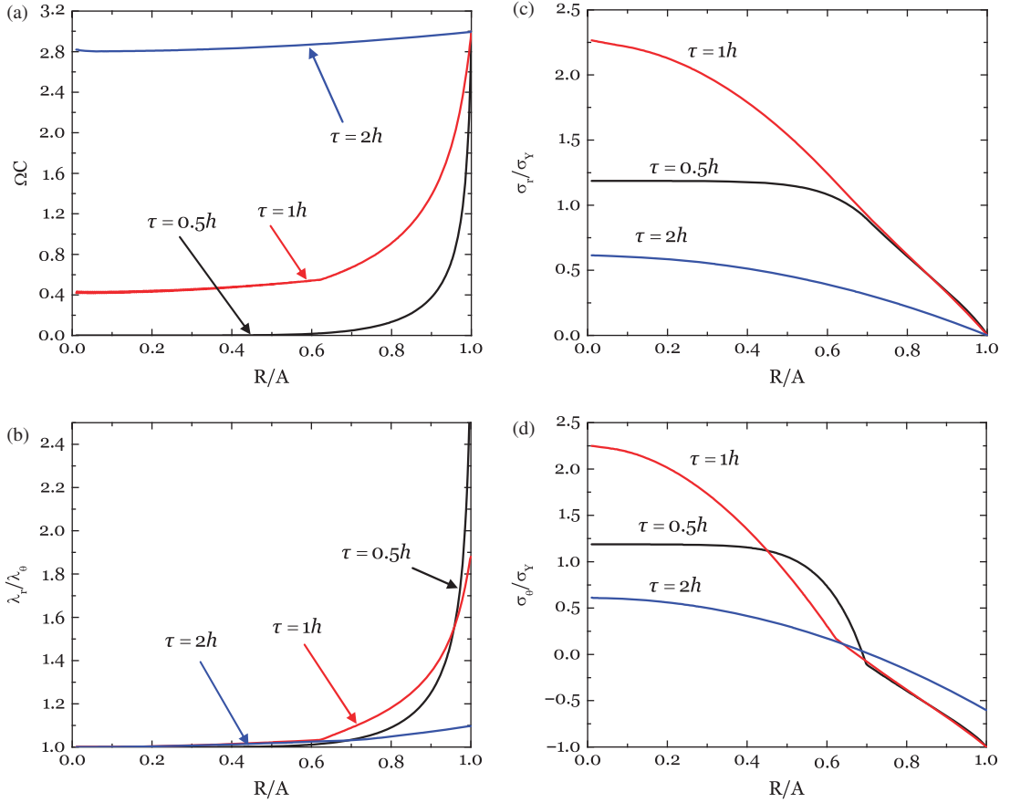
Fig. 7. The effect of the charging rate on various fields: (a) concentration of lithium, (b) ratio of radial stretch to hoop stretch, (c) radial stress, and (d) hoop stress.
