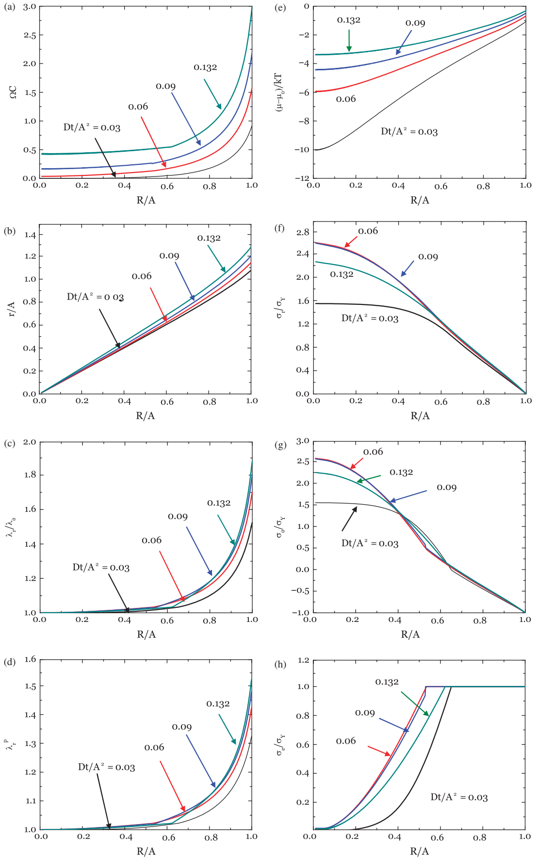
Fig. 4. As a spherical particle is being charged at the rate of \tau = 1 h, various fields evolve: (a) concentration of lithium, (b) deformation field, (c) ratio of the radial stretch to the hoop stretch, (d) plastic stretch in the radial direction, (e) chemical potential of lithium, (f) radial stress, (g) hoop stress, and (h) equivalent stress.
