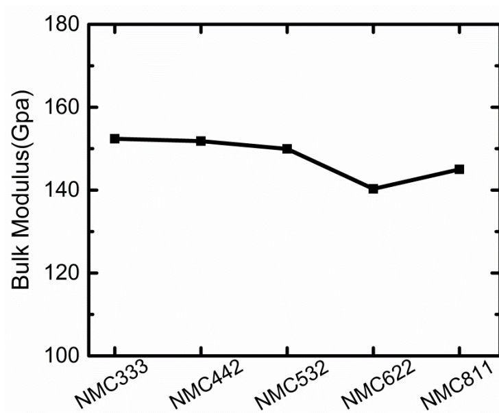
Figure S2. Bulk modulus of the five NMC compositions calculated from the VCA model.
