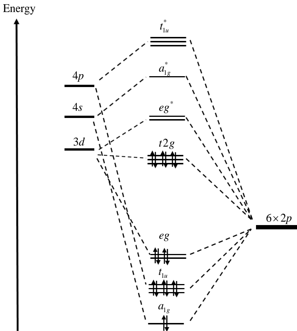
Figure S1. Molecular orbital diagram of the transition metal complex showing the d orbital electron population of \text{Co}^{3+} and O 2p orbital.
