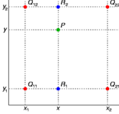
Figure 1: Bilinear Interpolation
