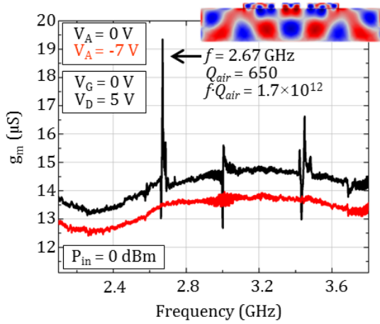
Fig. 9: Measured frequency response of PE drive-HEMT sense AlGaN/GaN resonator, in air. The transconductance, g_m = Y_{21} - Y_{12} , is suppressed when the 2DEG under the drive electrode is depleted.
