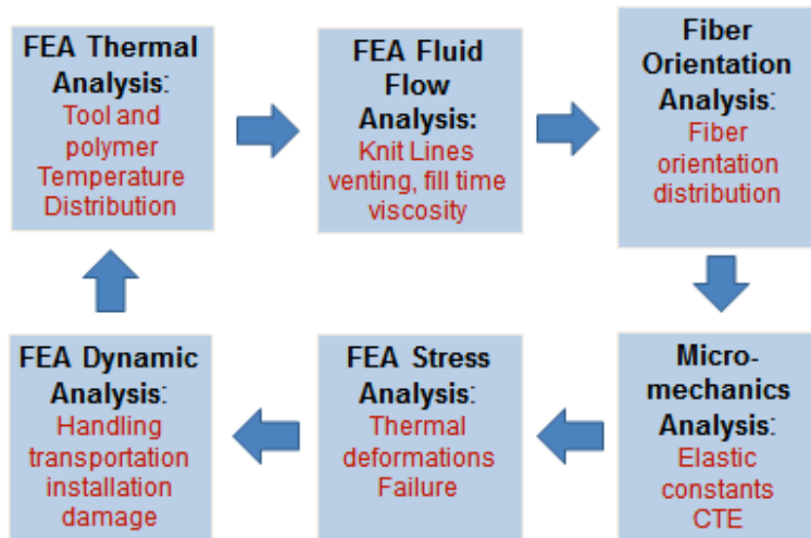
Figure 3 Composites molding simulation
