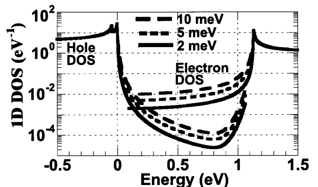
FIG. 3. One dimensional density of states for the electron and hole bands for three different coherent lifetimes: 33, 66, and 165 fs corresponding to the imaginary potentials 10, 5, and 2 meV, respectively.
