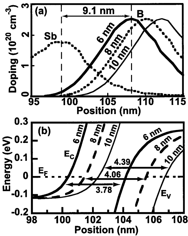
FIG. 8. (a) Sb and B SIMS distributions for the 700 °C anneal from Ref. 4. The B distribution is labeled by the nominal distance between Sb and B \delta doping of 6 nm. The actual peak-to-peak distance is 9.1 nm. This B distribution is then shifted to the right in 2 nm increments and labeled as 8 and 10 nm corresponding to our hypothetical experiment of increasing the nominal intrinsic layer distance. (b) Closeup of the tunnel junction resulting from the three B distributions shown in (a). The corresponding tunnel distance is shown.
