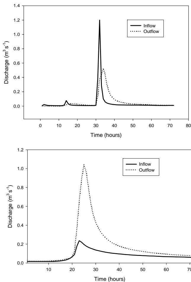
Figure 8. Inflow and outflow hydrograph for two storm flow events during 1994.
