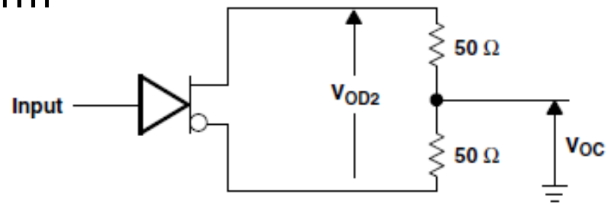
Figure 1. Differential and Common-Mode Output Voltages
