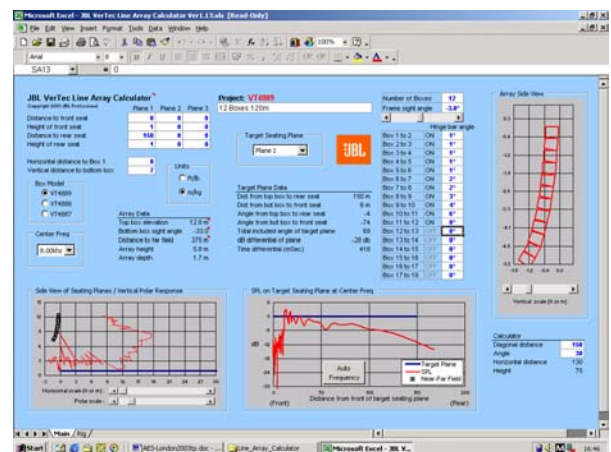
Fig A4. 12 Boxes 1,1,1,1,1,2,2,3,4,6,8 at 8kHz
