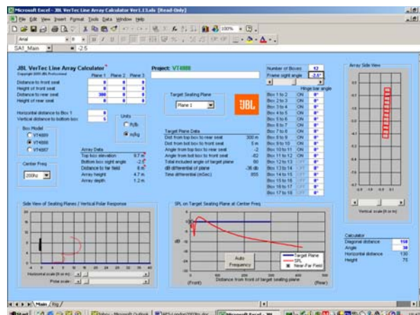
Fig 9. 12xVT4888 at 0deg splay angle, 200Hz.
