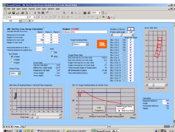
Fig A3. 6 Boxes 2,2,4,6,8 at 250Hz
