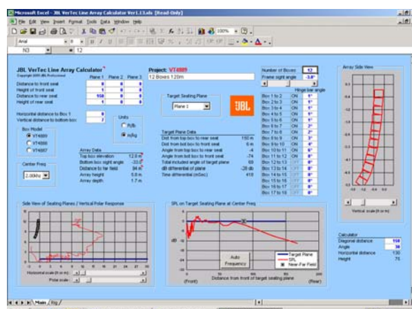
Fig 2. (A5) 12 Boxes 1,1,1,1,2,2,3,4,6,8 at 2kHz [~120m]
