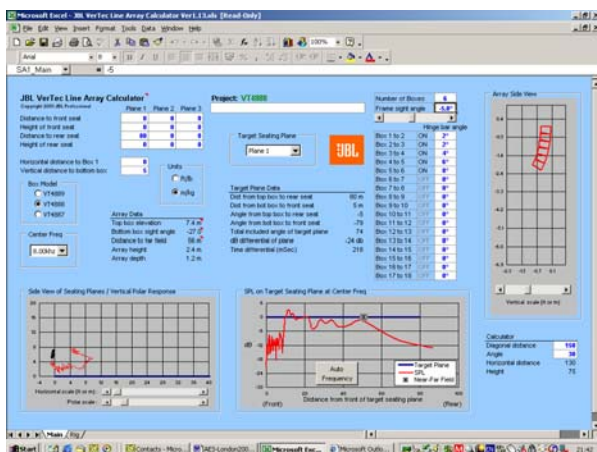
Fig 16. (A11) 6x VT4888 2,2,4,6,8 at 8kHz
