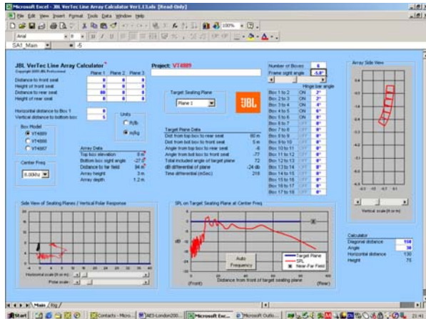
Fig A10. 6x VT4889 2,2,4,6,8 at 8kHz
