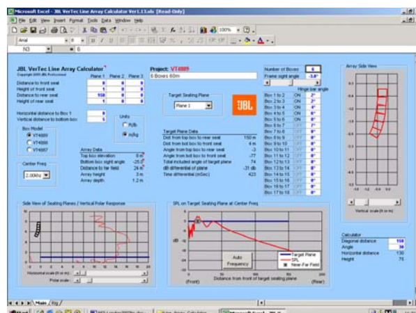
Fig 1. (A2) 6 Boxes 2,2,4,6,8 at 2kHz [~60m]
