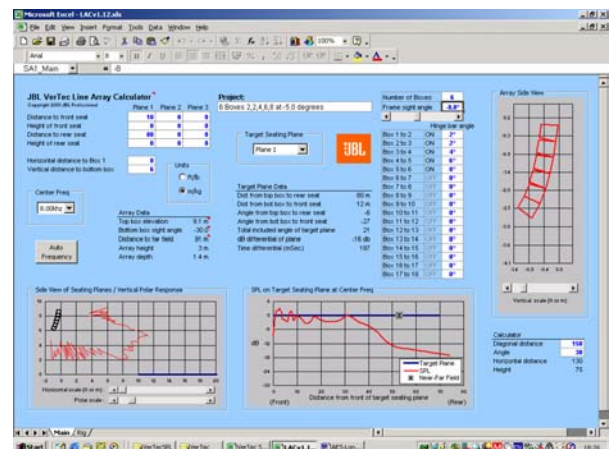
Fig 5. 6 boxes 2,2,4,6,8 at -8degrees
