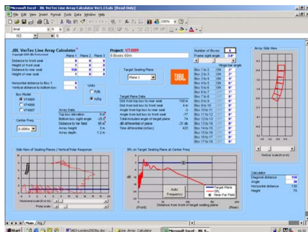
Fig A1. 6 Boxes 2,2,4,6,8 at 8kHz
