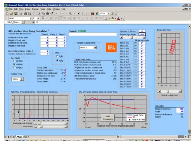
Fig A14. 6x VT4888 2,2,4,6,8 at 200Hz
