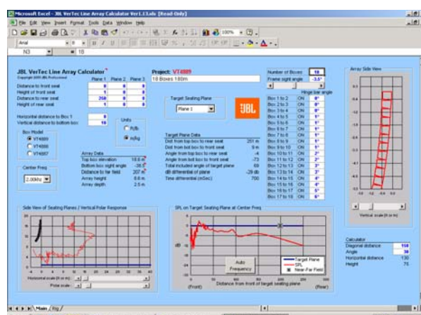
Fig 3. (A8) 18 Boxes 0,0,0,1,1,1,1,1,1,2,2,3,3,4,4,5,6 at 2kHz [~180m]
