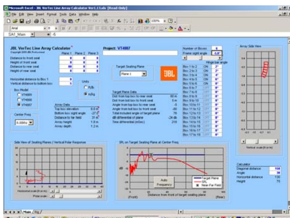
Fig A12. 6x VT4887 2,2,4,6,8 at 8kHz
