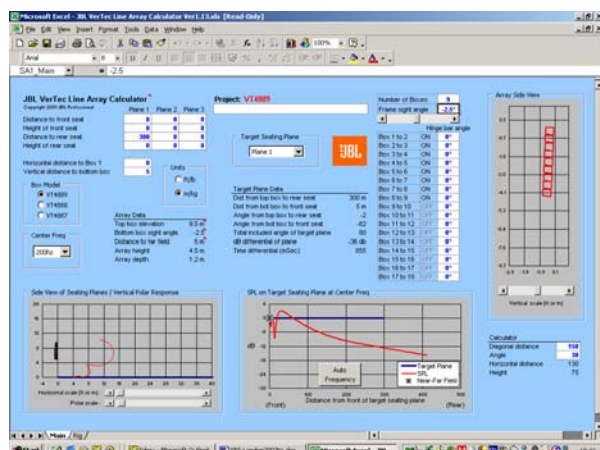
Fig 10. 9xVT4889 at 0deg splay angle, 200Hz. [-12dB@300m]
