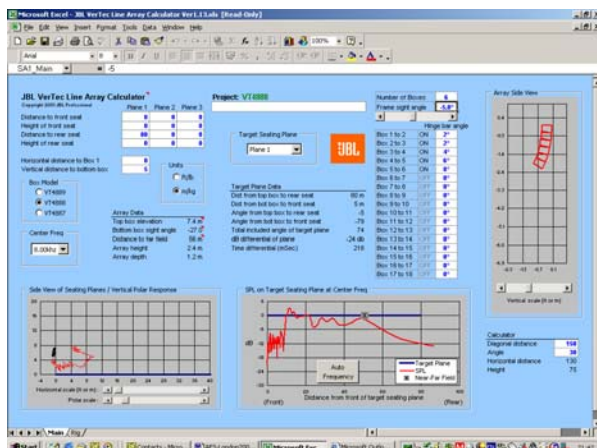
Fig A11. 6x VT4888 2,2,4,6,8 at 8kHz
