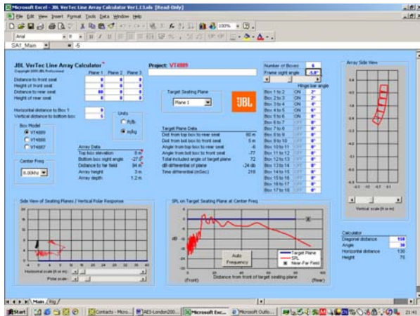
Fig 15. (A10) 6x VT4889 2,2,4,6,8 at 8kHz
