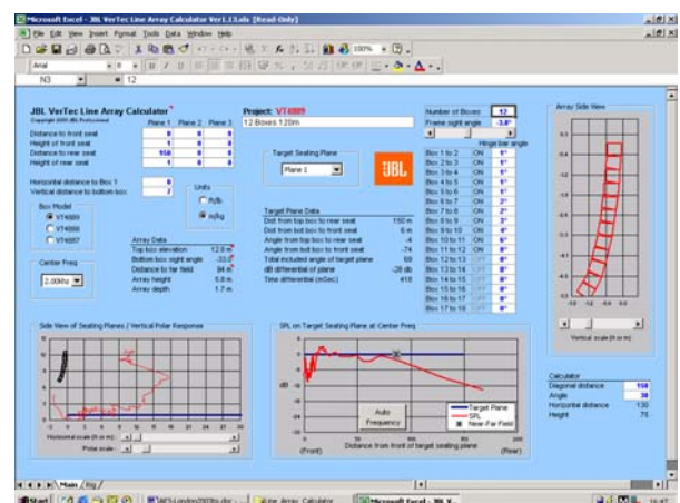
Fig A5. 12 Boxes 1,1,1,1,1,2,2,3,4,6,8 at 2kHz
