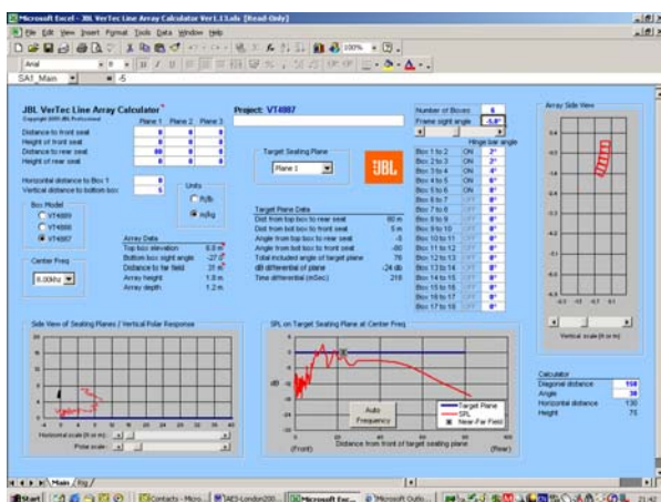
Fig 17. (A12) 6x VT4887 2,2,4,6,8 at 8kHz
