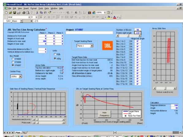
Fig 8. 18xVT4887 at 0deg splay angle, 200Hz. [-12dB@300m]
