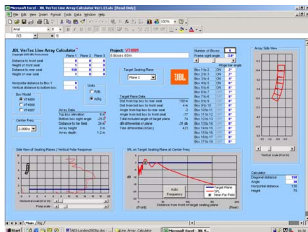
Fig A2. 6 Boxes 2,2,4,6,8 at 2kHz
