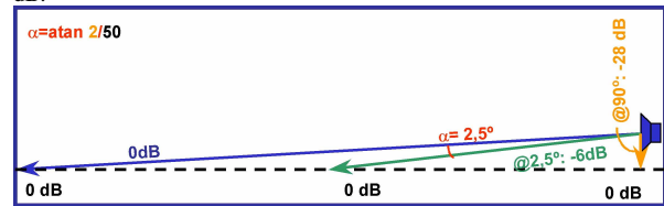
Figure 17: Typical Array loudspeaker design.
