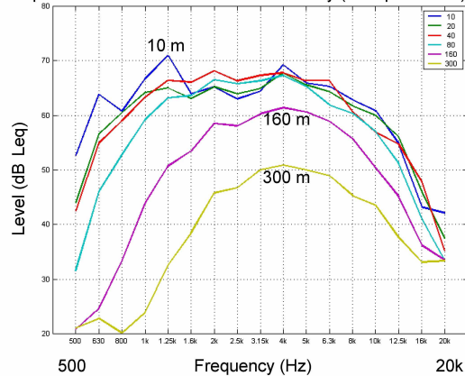
Figure 12: Measured sound levels (Leq) of an H.F. array.
