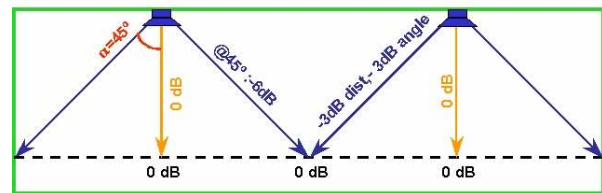
Figure 15: Typical ceiling speaker design
