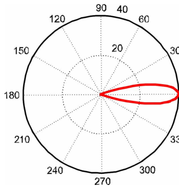
Figure 9b: 2D polar plot of the same array at 1000 Hz tone.
