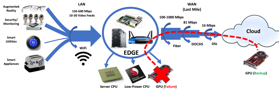
Figure 1: High-bandwidth edge services on the left generate dense video or less dense environmental data that needs to be processed on the edge. The high bandwidth of WiFi allows edge computers such as ARM-based Raspberry Pi’s, Routers, and traditional tower servers to process the data. When there is a failure, the data can be re-routed to the cloud, but this re-routing is limited by the capacity of the WAN system.
