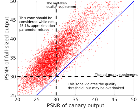
Figure 2: The PSNR of full-sized output versus the PSNR of canary output, for the 1-frames of 106 videos on one of our application Boxblur-Vignette-Dilation video filter pipeline. The PSNR of full output is higher for over 98% approximation settings and 45.1% of the approximation settings lie in such a zone that is ignored by IRA approach but actually satisfies the quality requirement.
