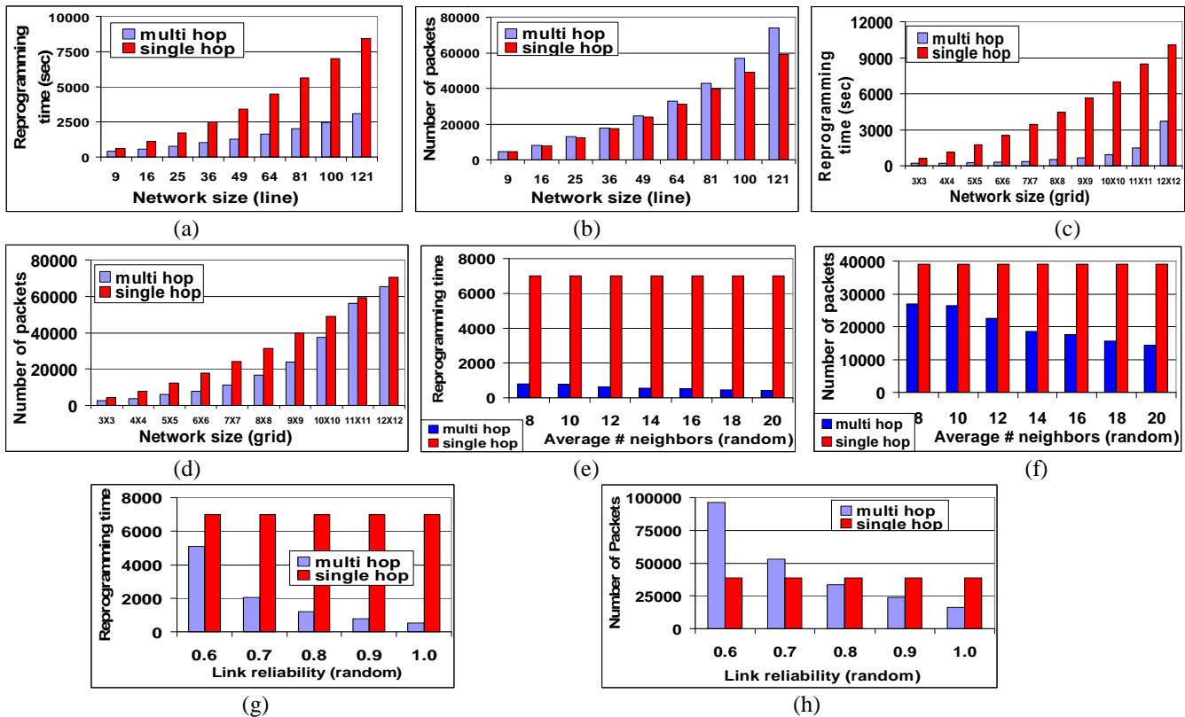
Figure 7: Simulation results. Reprogramming time as a function of network size for (a) linear and (c) grid networks (LRM=0.9). Number of transmitted packets as a function of network size for (b) linear and (d) grid networks (LRM=0.9). For random topology, (e) reprogramming time and (f) number of transmitted packets as a function of network density (LRM=0.9); (g) Reprogramming time and (h) number of transmitted packets as a function of link reliability for 100-random topology (Mean number of neighbors=8). The multi hop result bar is to the left of the single hop result bar.
