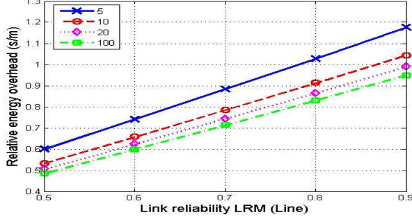
Figure 3. Relative energy overhead (single hop : multi-hop) as a function of link reliability for linear topologies
