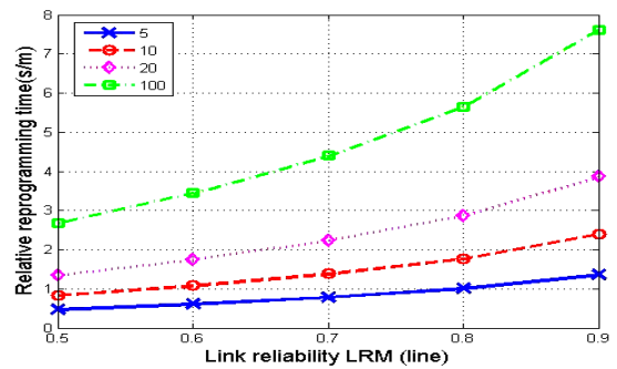
Figure 1. Relative reprogramming time (single hop : multi-hop) as a function of link reliability for linear topologies
