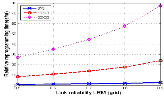
Figure 2. Relative reprogramming time (single hop : multi-hop) as a function of link reliability for grid topologies
