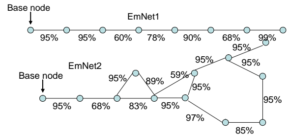
Figure 5: Two CSOnet networks: EmNet1 and EmNet2
