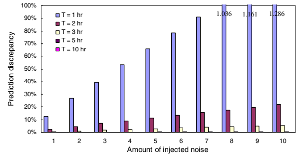
Figure 8. Prediction discrepancy with different amounts of noise injected to a training log for weekdays. T is the length of the future time window. Prediction discrepancy is the relative difference between the prediction results using the training data with and without noise injection respectively.
