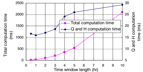
Figure 4. Computation time of resource availability prediction for time windows with different lengths. The prediction is to predict the probability that a resource will be available throughout a given time window.
