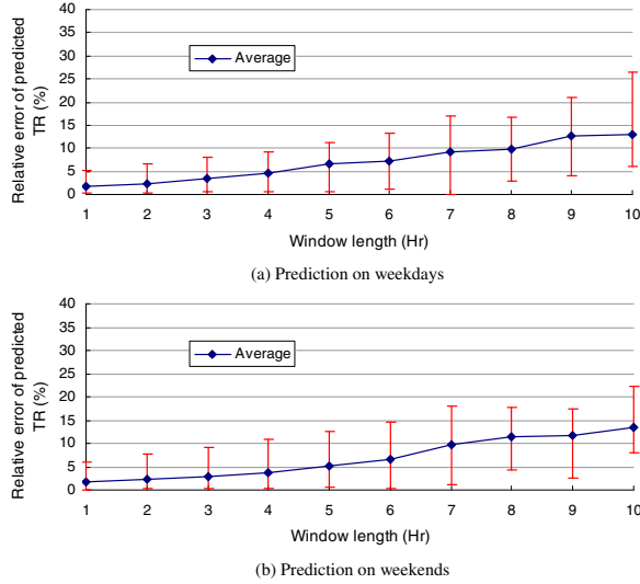
Figure 5. Relative errors of predicted TR. Each point plots the average error of predictions over 24 time windows with different start time ranging from 0:00 to 23:00, in steps of 1 hour. The bars show minimum and maximum prediction errors.
