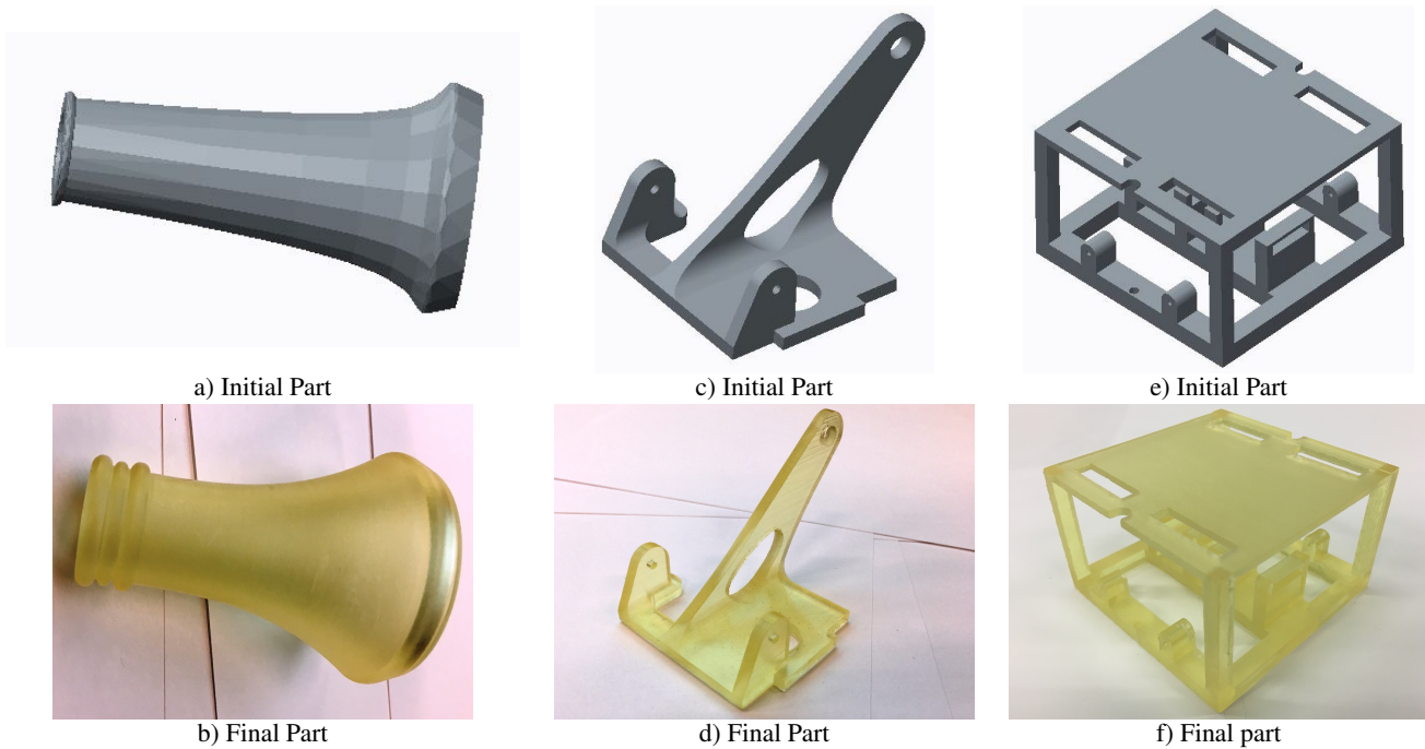
Fig. 3. Examples of parts from the second study. Sub-figures a) and b) show one of only three examples of any changes made. The other two examples show no change from pre to post. All three changes we observed were unrelated to improving the manufacturability.
