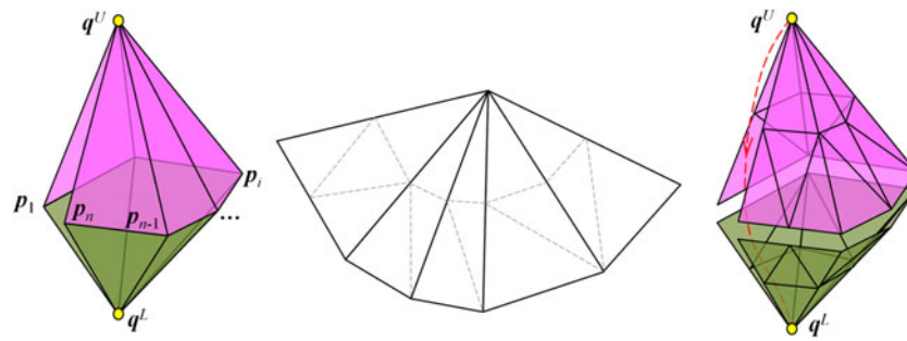
Fig. 5 When isometric deformation is conducted to optimize the shape of a flattenable mesh surface, the computation may not converge because of topological obstacles. (Left) If the optimal moving direction of a vertex q^U is pointing towards q^L and all p_i s are not allowed to move, the movement of q^U is prevented since the lengths of edges, \|q^U p_i\| , should not be changed during isometric deformation. Here,
