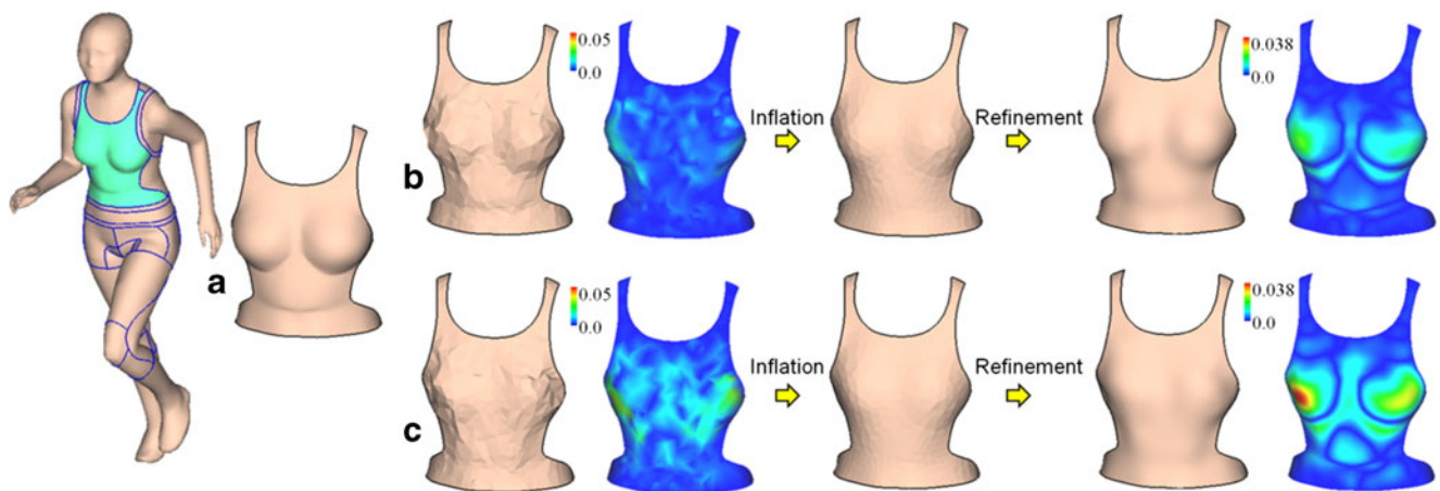
Fig. 10 For the highly curved surfaces, using a V-spring-based inflation can improve the shape of resultant patch in surface fitting. a The front piece of a sports vest is highly curved. b One flattenable mesh surface patch generated by shape perturbation and its results
