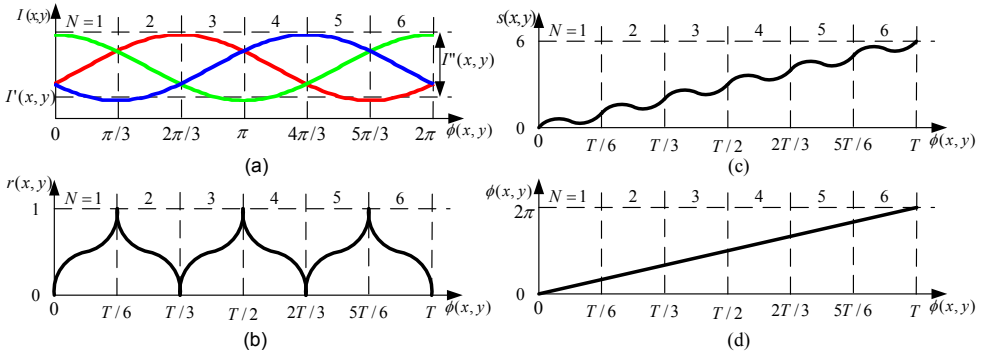
Fig. 8. Schematic illustration for fast three-step phase-shifting algorithm. (a) One period of fringe is uniformly divided into six regions; (b) The intensity ratio for one period of fringe; (c) After slope map after removing the sawtooth shape of the intensity ratio map; (d) The phase after compensate for the approximation error and scaled to its original phase value.
