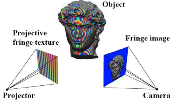
Figure 4: System setup.
