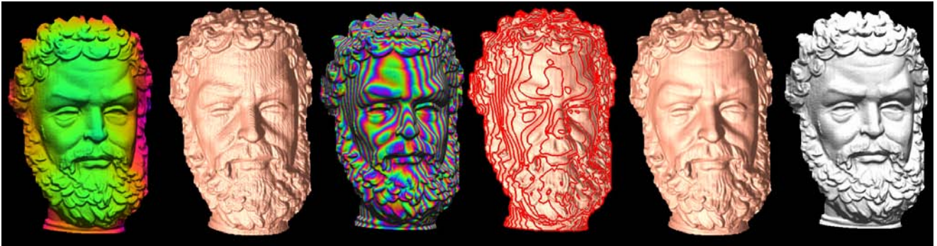
Figure 3: Two-wavelength phase unwrapping. The first image is a holoimage with spatial frequency 1Hz; the coarse reconstructed geometry is shown in the second image does not need phase unwrapping. This is used as a reference to phase unwrap holoimages with denser fringes. The 3rd image is a holoimage with spatial frequency 64Hz. The 4th image is the reconstructed geometry without phase unwrapping; the red contours show phase jumps. The 5th image is the reconstructed geometric surface after phase unwrapping to depth consistency with the 2nd image. The last image is a shaded image.
