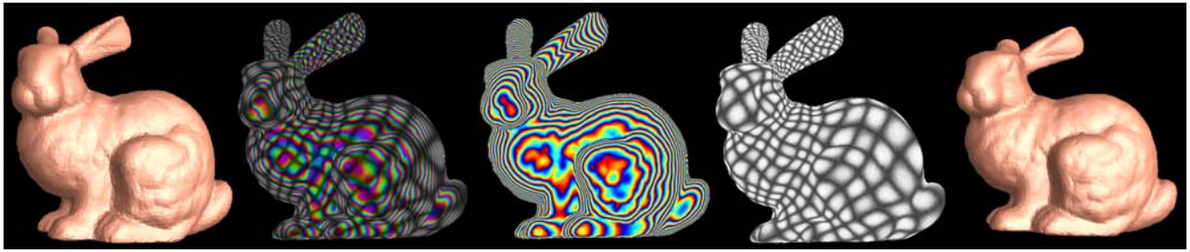
Figure 8: Holomap of texture mapped surfaces. The original geometric surface is flat shaded in the first image, the flat triangles are visible. The second image is the 24-bit holomap for the textured bunny surface. The third image shows the phase map. The fourth image shows the texture reconstructed from the holomap. The reconstructed geometry is shown in the last image, the flat triangles are recovered.
