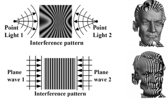
Figure 3: Principle of holoimages. Phase information is encoded in the interference fringe pattern. Geometric information is encoded in the phase information.
