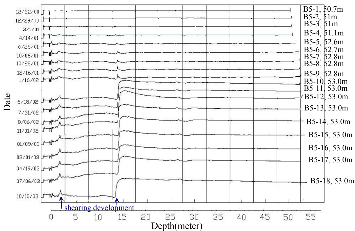
Fig.7 Recorded waveform at B-5 TDR monitoring station
