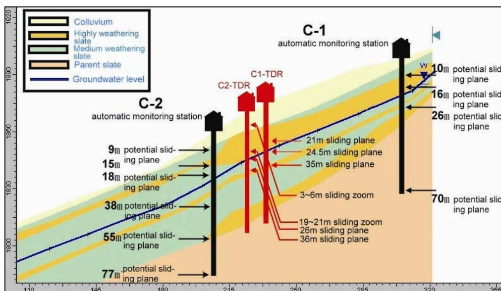
Fig. 13 Profile of slope including C1-TDR and C2-TDR cables
