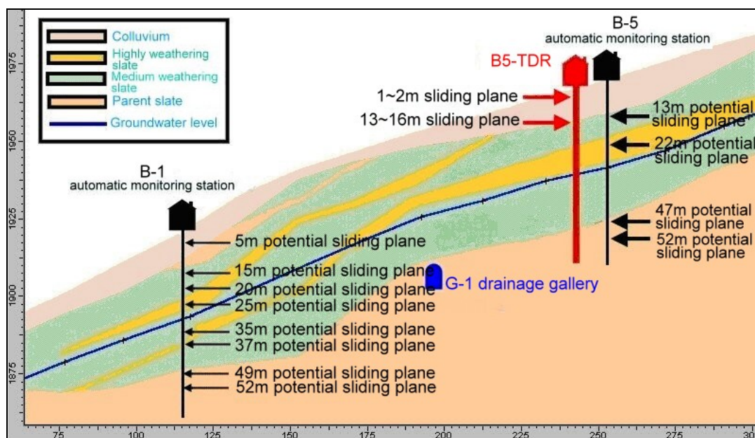
Fig.11 Profile of slope including B5-TDR cables
