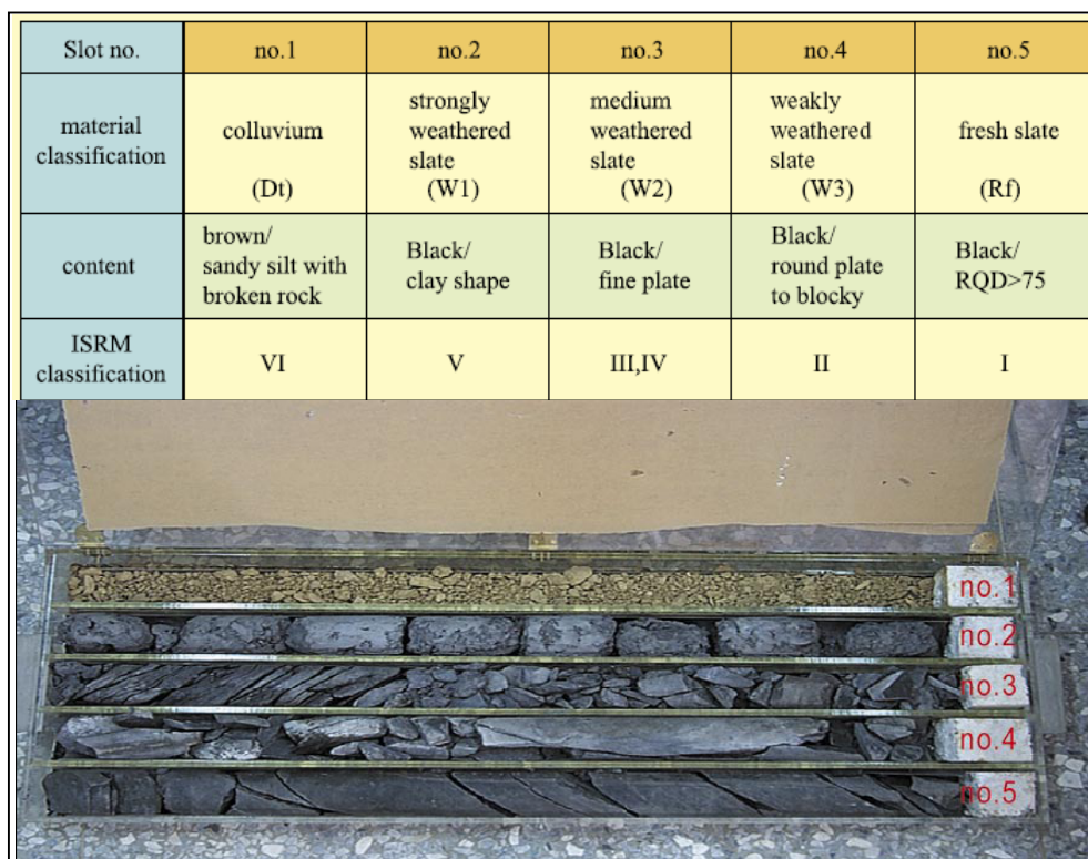
Fig. 2 Classification of Geo-materials
