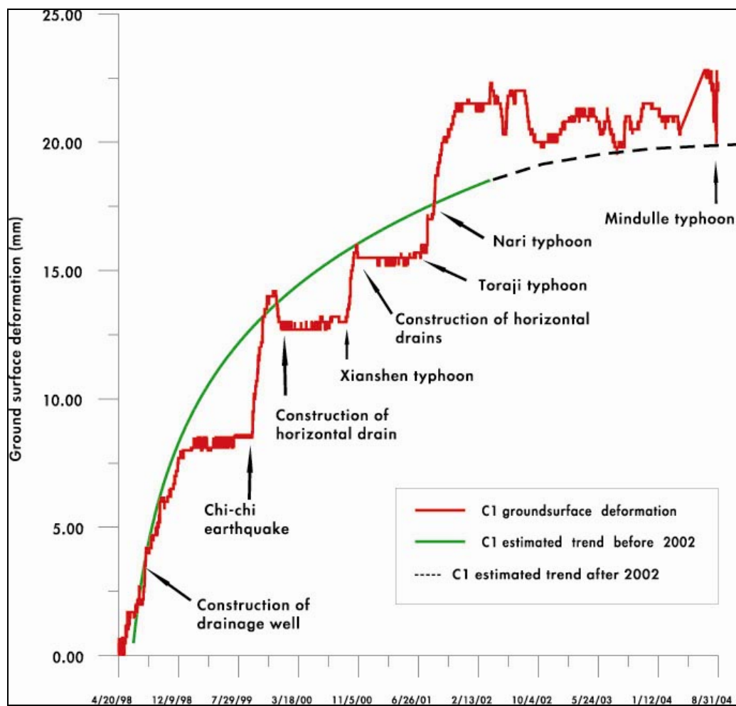
Fig.15 Ground surface deformation and its estimated trend for C1 station
