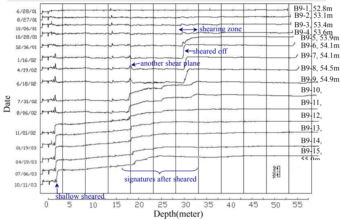
Fig.8 Recorded waveform at B-9 TDR monitoring station
