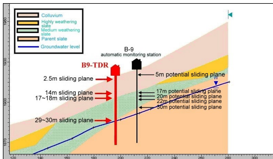
Fig.12 Profile of slope including B9-TDR cables
