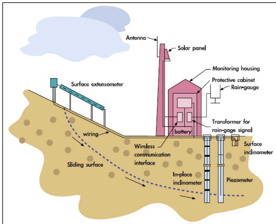
Fig. 3 Schematic of automatic monitoring system applied in Li-shan landslide area
