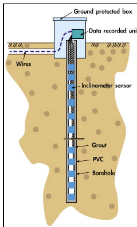
Fig.4 Setup of probe inclinometer
