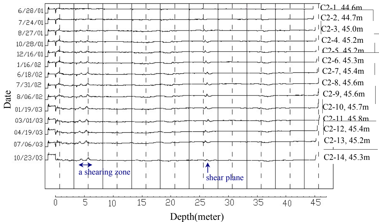
Fig.10 Recorded waveform at C-2 TDR monitoring station
