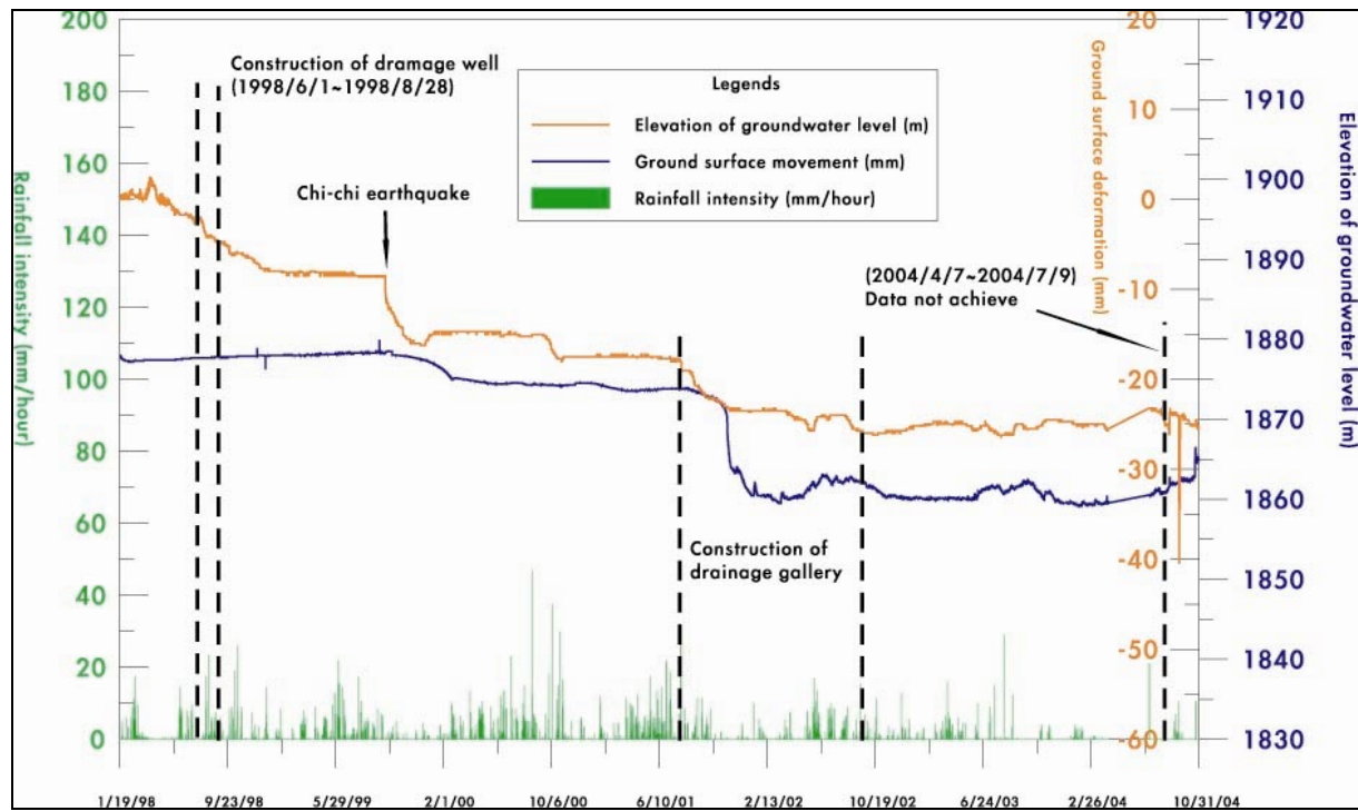
Fig.14 Relation between rainfall intensity, groundwater level and surface deformation in C1 station
