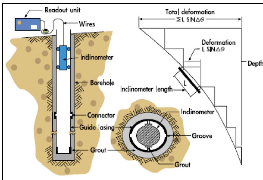
Fig.5 Sketch of probe inclinometer with manual readout
