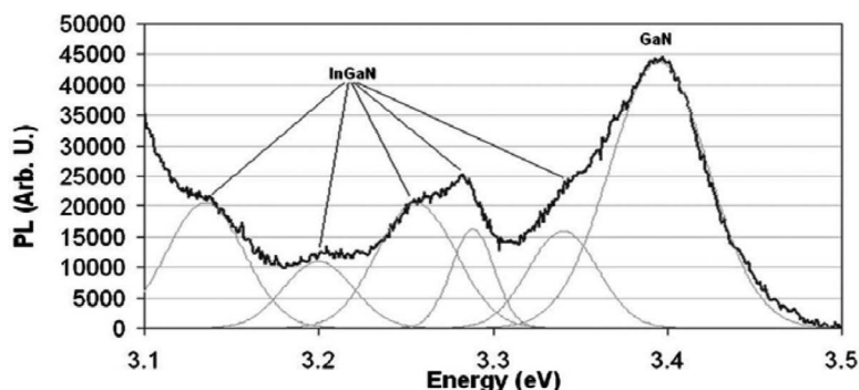
Figure 3. RT photoluminescence of MOCVD-grown GaN/InGaN solar cell indicating an apparent phase separation in InGaN. 48
