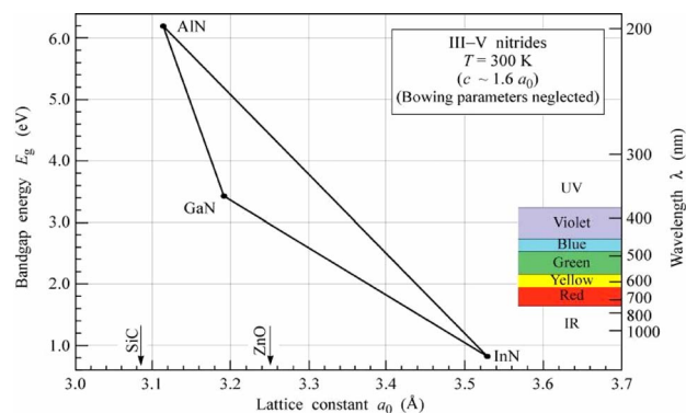
Figure 1. Bandgap vs. lattice constant for III-Nitrides. 2
