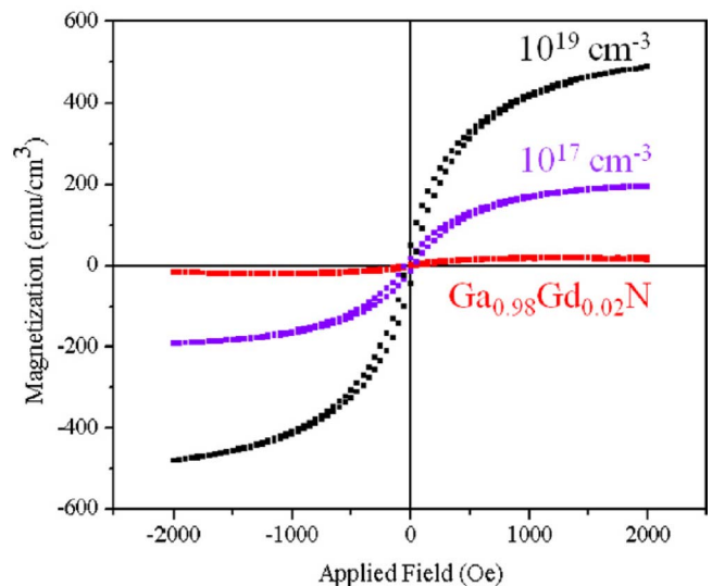
Figure 4. RT VSM measurements of p-doped GaGdN indicating carrier concentration for Mg-doped GaGdN. 85
