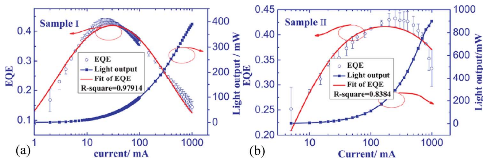
Figure 2. Quantum efficiency and light output as a function of current in (a) LED on sapphire substrate (b) LED on GaN substrate. The data points represent the measured results. The solid line on quantum efficiency represents the fitting curve based on carrier's rate equation. 30
