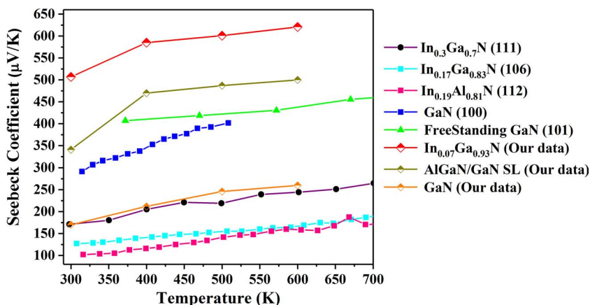
Figure 5. Temperature dependent Seebeck coefficient for various binary materials and alloys.
