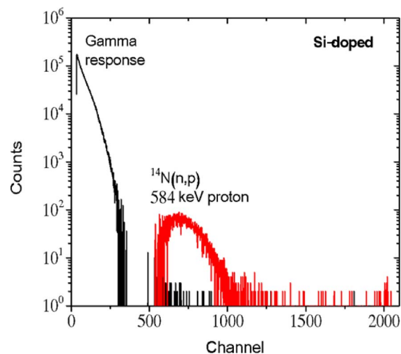
Figure 6. Gamma and thermal neutron scintillation spectra produced by bare Si-doped GaN scintillator.
