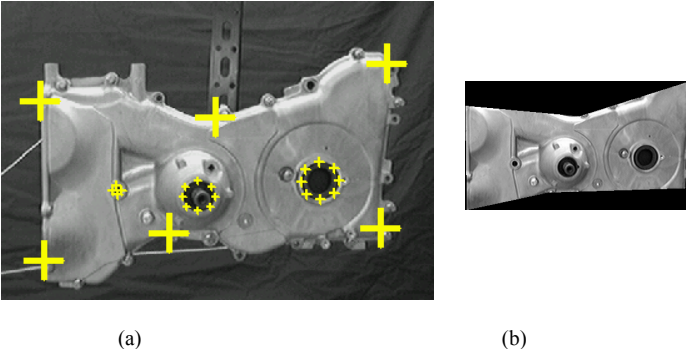
Figure 1. (a) The object image with the landmark points (cross mark), (b) The image region covered by the landmark points
