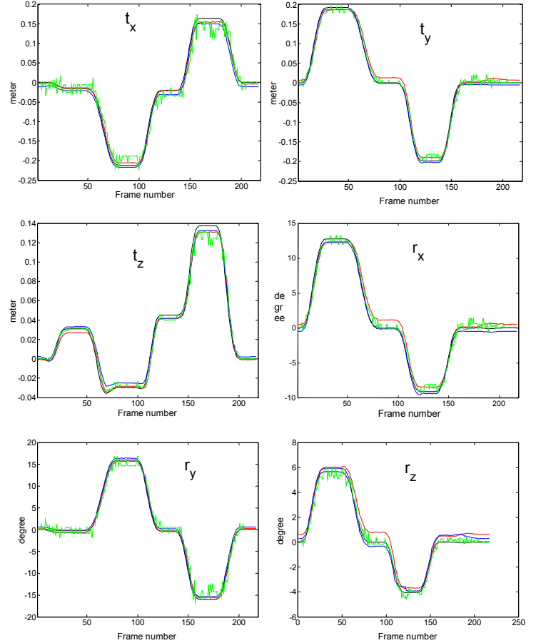
Figure 4. Groundtruth pose (black) and estimated pose of 1 st method (red), 2 nd method (blue) and geometrical-based method [14] (green).
