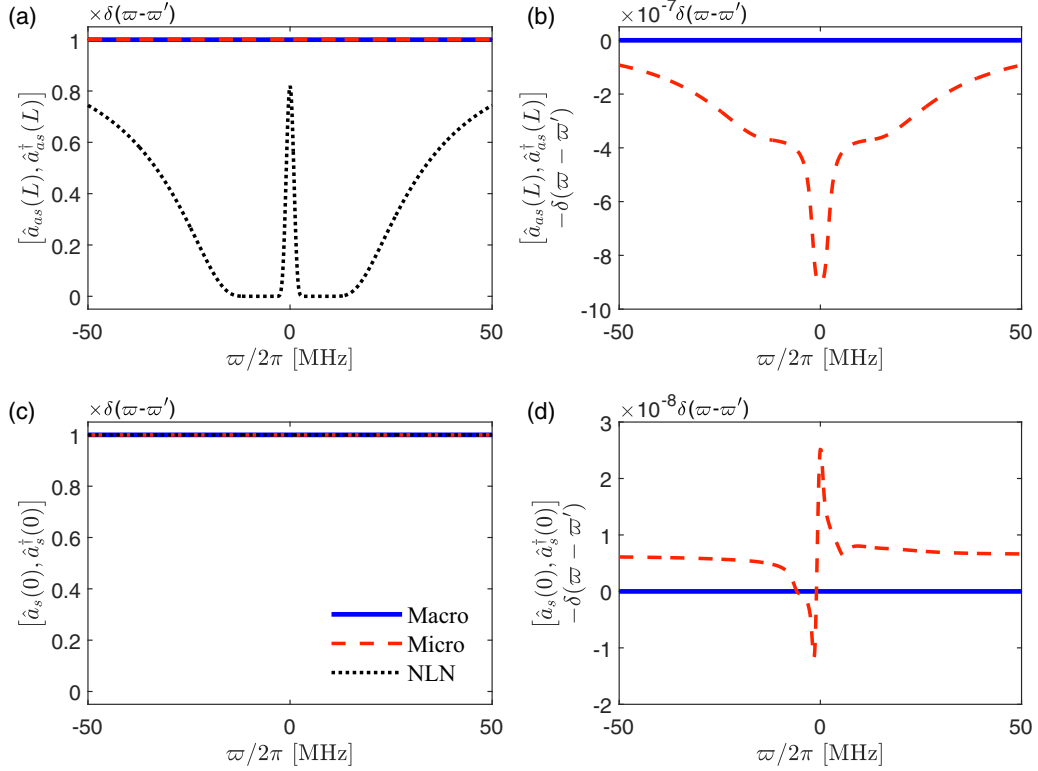
FIG. 3. Comparison of commutation relations between the macroscopic (Macro, blue solid lines) and microscopic (Micro, red dashed lines) approaches in the group delay regime: (a) [\hat{a}_{as}(L), \hat{a}_{as}^\dagger(L)] , (b) [\hat{a}_{as}(L), \hat{a}_{as}^\dagger(L)] - \delta(\omega - \omega') , (c) [\hat{a}_s(0), \hat{a}_s^\dagger(0)] , and (d) [\hat{a}_s(0), \hat{a}_s^\dagger(0)] - \delta(\omega - \omega') . The results with no Langevin noise operators (NLN) are shown as black dotted lines in (a) and (c).
