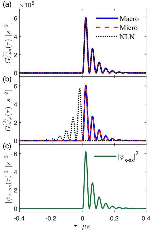
FIG. 10. Two-photon Glauber correlation in time domain in the damped Rabi oscillation regime: (a) G_{s,as}^{(2)}(\tau) and (b) G_{as,s}^{(2)}(\tau) . The simulation conditions are the same as those in Figs. 6–8. (c) The analytic solution for the biphoton waveform |\psi_{s-as}(\tau)|^2 . NLN: no Langevin noise included.
