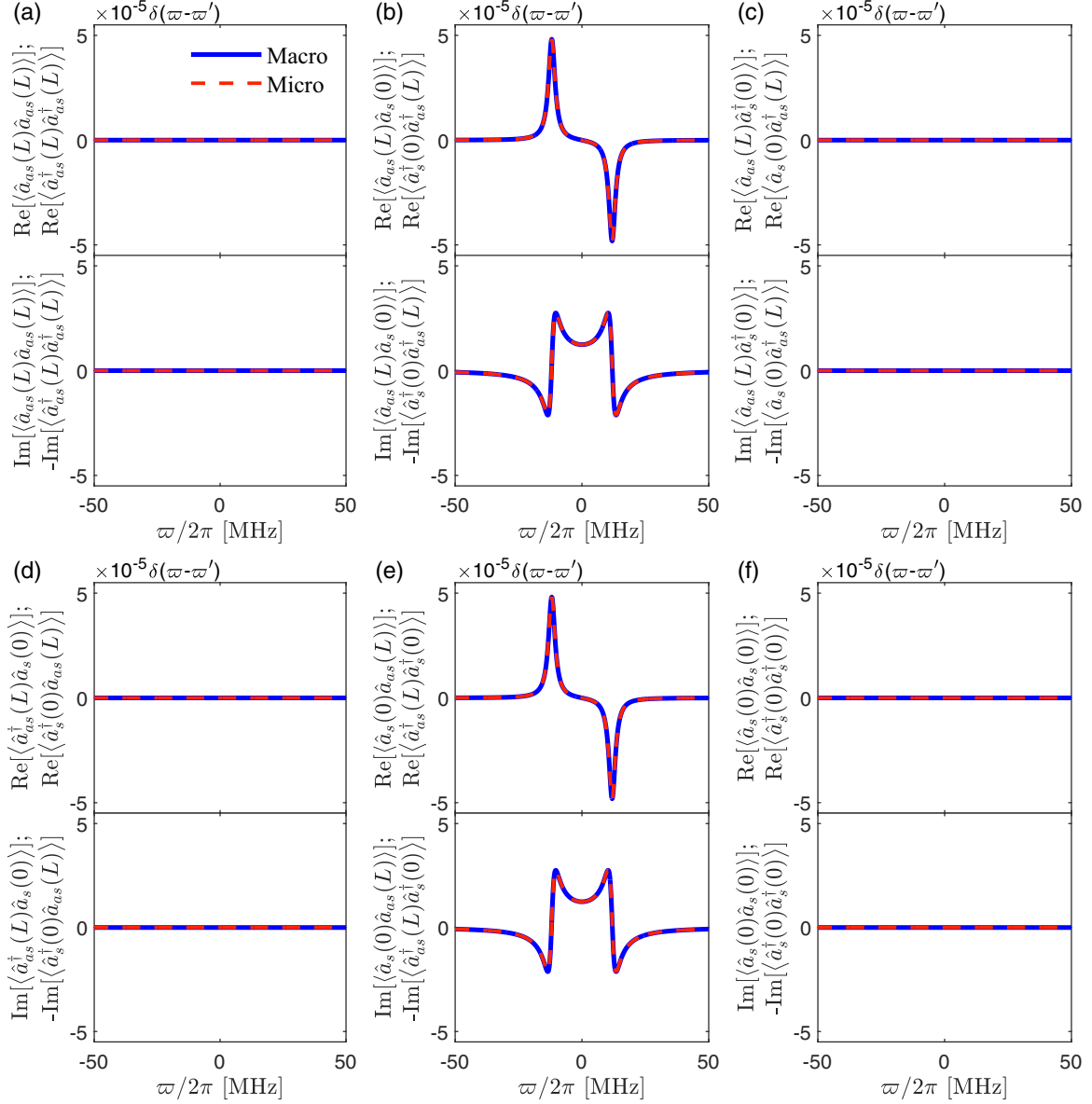
FIG. 8. Twelve complex correlations of Stokes and anti-Stokes fields in the damped Rabi oscillation regime: (a) \langle \hat{a}_{as}(L)\hat{a}_{as}(L) \rangle = \langle \hat{a}_{as}^\dagger(L)\hat{a}_{as}^\dagger(L) \rangle^* , (b) \langle \hat{a}_{as}(L)\hat{a}_s(0) \rangle = \langle \hat{a}_s^\dagger(0)\hat{a}_{as}^\dagger(L) \rangle^* , (c) \langle \hat{a}_{as}(L)\hat{a}_s^\dagger(0) \rangle = \langle \hat{a}_s(0)\hat{a}_{as}^\dagger(L) \rangle^* , (d) \langle \hat{a}_s^\dagger(L)\hat{a}_{as}(0) \rangle = \langle \hat{a}_{as}^\dagger(0)\hat{a}_s(L) \rangle^* , (e) \langle \hat{a}_s(0)\hat{a}_{as}(L) \rangle = \langle \hat{a}_{as}^\dagger(L)\hat{a}_s^\dagger(0) \rangle^* , and (f) \langle \hat{a}_s(0)\hat{a}_s(0) \rangle = \langle \hat{a}_s^\dagger(0)\hat{a}_s^\dagger(0) \rangle^* . The macroscopic (Macro) and microscopic (Micro) approaches are shown as blue solid and red dashed lines, respectively.
