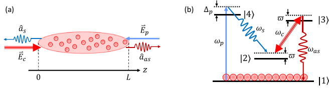
FIG. 2. Spontaneous four-wave mixing (SFWM) in a double- \Lambda four-level cold atomic medium. (a) Backward-wave geometry of SFWM optical configuration. Driven by counterpropagating pump ( E_p ) and coupling ( E_c ) beams, phase-matched backward Stokes ( \hat{a}_s ) and anti-Stokes ( \hat{a}_{as} ) are spontaneously generated from a laser-cooled atomic medium. (b) Atomic energy-level diagram. The pump ( \omega_p ) laser is detuned with \Delta_p from transition |1\rangle \rightarrow |4\rangle , and the coupling ( \omega_c ) laser is on-resonant with transition |2\rangle \rightarrow |3\rangle . Stokes ( \omega_s ) photons are spontaneously generated from transition |4\rangle \rightarrow |2\rangle , and anti-Stokes ( \omega_{as} ) photons from transition |3\rangle \rightarrow |1\rangle . \varpi = \omega_{as} - \omega_{13} is the anti-Stokes photon frequency detuning from transition |1\rangle \rightarrow |3\rangle .
