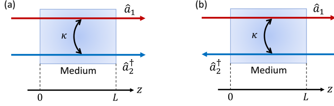
FIG. 1. Schematics of two coupled phase-conjugated electromagnetic waves: (a) forward-wave configuration, and (b) backward-wave configuration. \kappa is the nonlinear coupling coefficient between the two modes.
