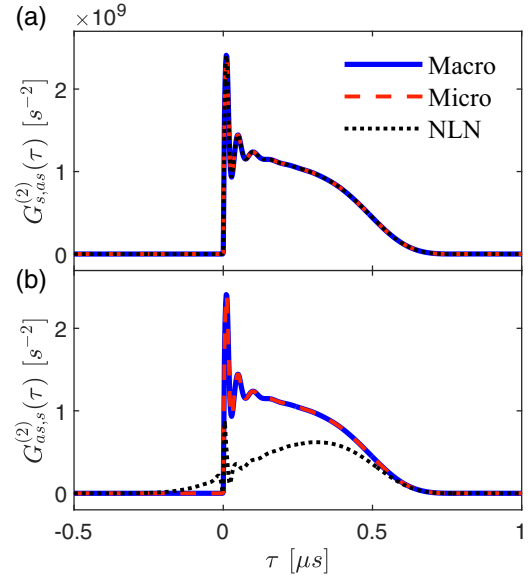
FIG. 9. Two-photon Glauber correlation in time domain in the group delay regime: (a) G_{s,as}^{(2)}(\tau) and (b) G_{as,s}^{(2)}(\tau) . The simulation conditions are the same as those in Figs. 3–5. NLN: no Langevin noise included.
