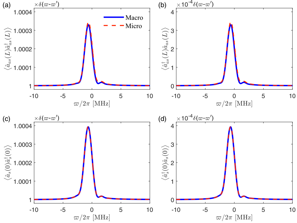
FIG. 4. Four real correlations of Stokes and anti-Stokes fields in the group delay regime: (a) \langle \hat{a}_{as}(L) \hat{a}_{as}^\dagger(L) \rangle , (b) \langle \hat{a}_{as}^\dagger(L) \hat{a}_{as}(L) \rangle , (c) \langle \hat{a}_s(0) \hat{a}_s^\dagger(0) \rangle , and (d) \langle \hat{a}_s^\dagger(0) \hat{a}_s(0) \rangle . The macroscopic (Macro) and microscopic (Micro) approaches are shown as blue solid and red dashed lines, respectively.
