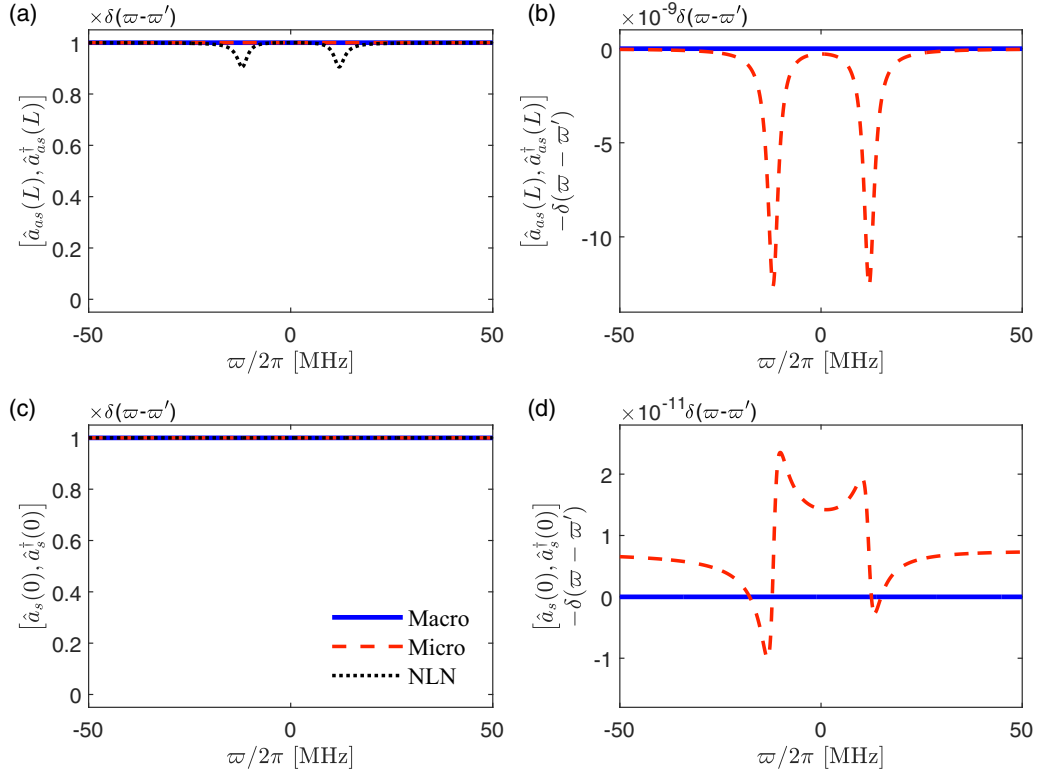
FIG. 6. Comparison of commutation relations between the macroscopic (Macro, blue solid lines) and microscopic (Micro, red dashed lines) approaches in the damped Rabi oscillation regime: (a) [\hat{a}_{as}(L), \hat{a}_{as}^\dagger(L)] , (b) [\hat{a}_{as}(L), \hat{a}_{as}^\dagger(L)] - \delta(\varpi - \varpi') , (c) [\hat{a}_s(0), \hat{a}_s^\dagger(0)] , and (d) [\hat{a}_s(0), \hat{a}_s^\dagger(0)] - \delta(\varpi - \varpi') . The results with no Langevin noise operators (“NLN”) are shown as black dotted lines in (a) and (c).
