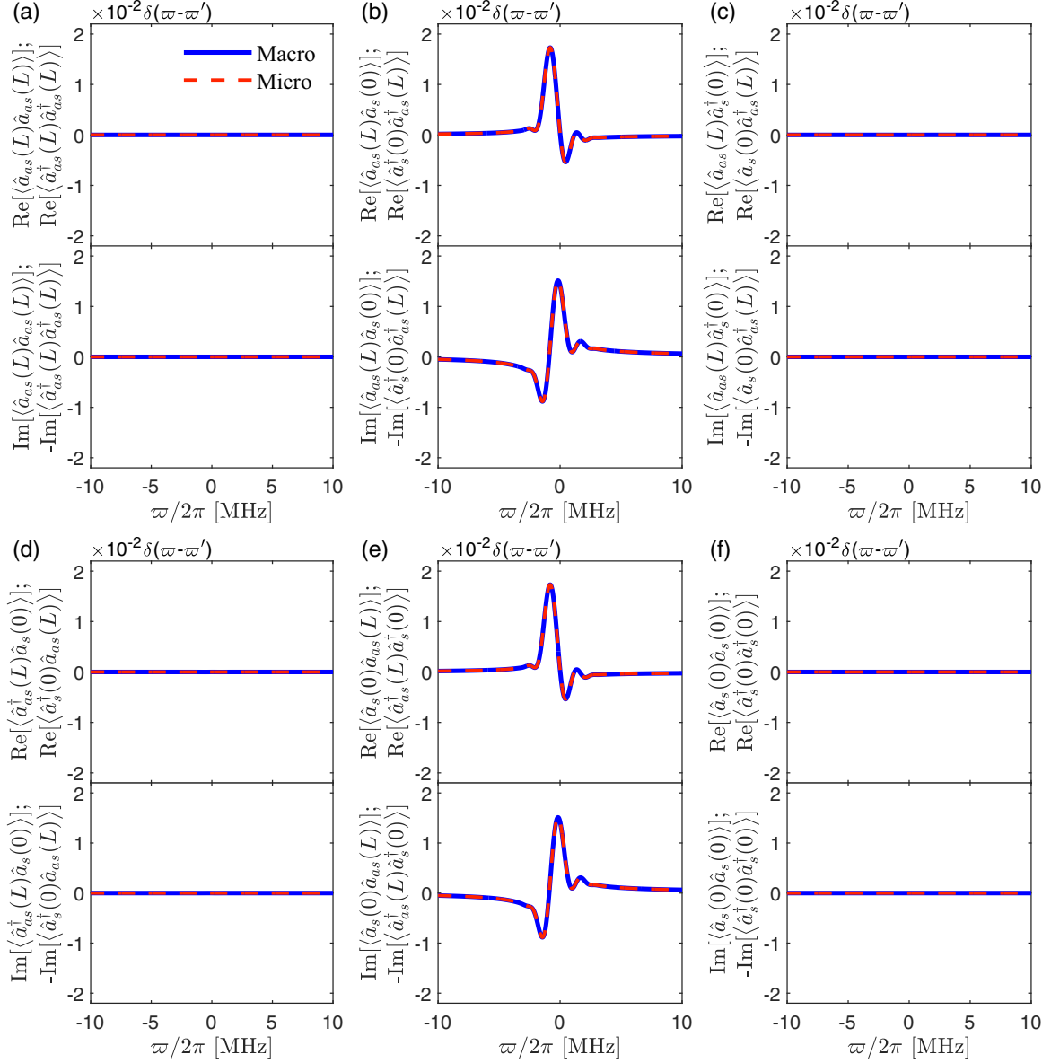
FIG. 5. Twelve complex correlations of Stokes and anti-Stokes fields in the group delay regime: (a) \langle \hat{a}_{as}(L)\hat{a}_{as}(L) \rangle = \langle \hat{a}_{as}^\dagger(L)\hat{a}_{as}^\dagger(L) \rangle^* , (b) \langle \hat{a}_{as}(L)\hat{a}_s(0) \rangle = \langle \hat{a}_s^\dagger(0)\hat{a}_{as}^\dagger(L) \rangle^* , (c) \langle \hat{a}_{as}(L)\hat{a}_s^\dagger(0) \rangle = \langle \hat{a}_s(0)\hat{a}_{as}^\dagger(L) \rangle^* , (d) \langle \hat{a}_s^\dagger(L)\hat{a}_s(0) \rangle = \langle \hat{a}_s^\dagger(0)\hat{a}_{as}(L) \rangle^* , (e) \langle \hat{a}_s(0)\hat{a}_{as}(L) \rangle = \langle \hat{a}_{as}^\dagger(L)\hat{a}_s^\dagger(0) \rangle^* , and (f) \langle \hat{a}_s(0)\hat{a}_s(0) \rangle = \langle \hat{a}_s^\dagger(0)\hat{a}_s^\dagger(0) \rangle^* . The macroscopic (Macro) and microscopic (Micro) approaches are shown as blue solid and red dashed lines, respectively.
