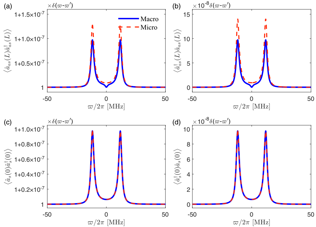
FIG. 7. Four real correlations of Stokes and anti-Stokes fields in the damped Rabi oscillation regime: (a) \langle \hat{a}_{as}(L) \hat{a}_{as}^\dagger(L) \rangle , (b) \langle \hat{a}_{as}^\dagger(L) \hat{a}_{as}(L) \rangle , (c) \langle \hat{a}_s(0) \hat{a}_s^\dagger(0) \rangle , and (d) \langle \hat{a}_s^\dagger(0) \hat{a}_s(0) \rangle . The macroscopic (Macro) and microscopic (Micro) approaches are shown as blue solid and red dashed lines, respectively.
