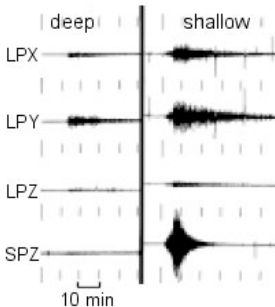
Representative lunar seismograms from the Apollo 16 station.
