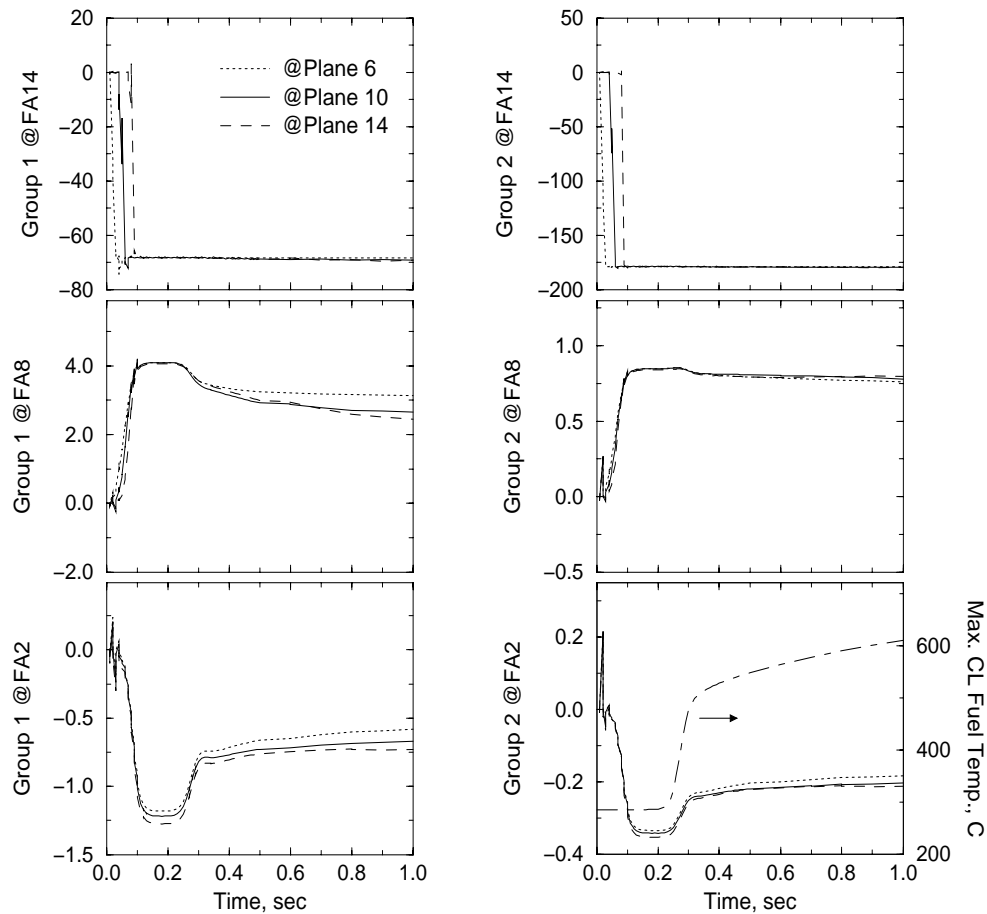
Figure 8.2: Assessment of Changes in the Corrective Nodal Coupling Coefficients
