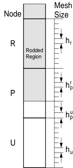
Figure 7.1: Geometry of Three-Node Problem
