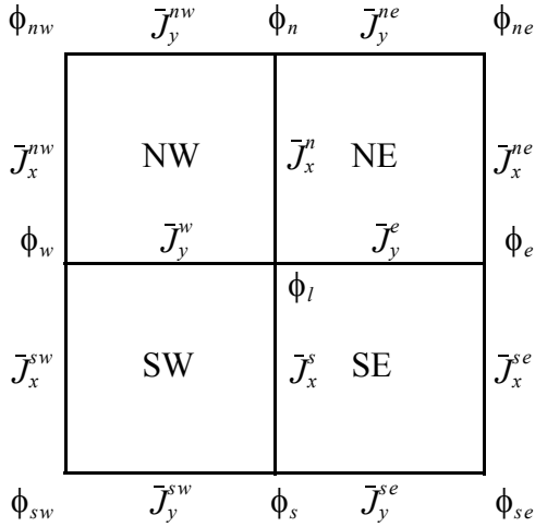
Figure 4.2: Variable Definition for Corner Flux Calculation
