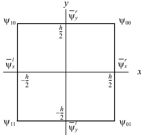
Figure 4.1: Coordinate and Boundary Conditions for Intranodal Expansion
