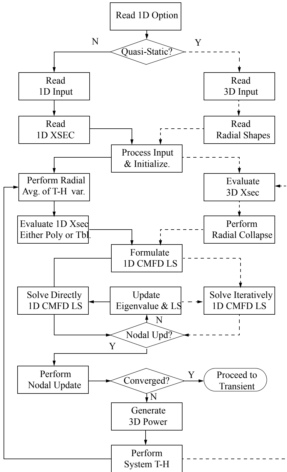
Figure 7.3: Steady-State 1-D Solution Sequence
