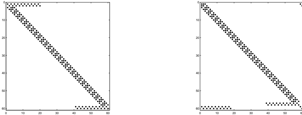
Figure 7.2: Matrix Structure of the Three-Node Problem; Left-Original, Right-Reordered
