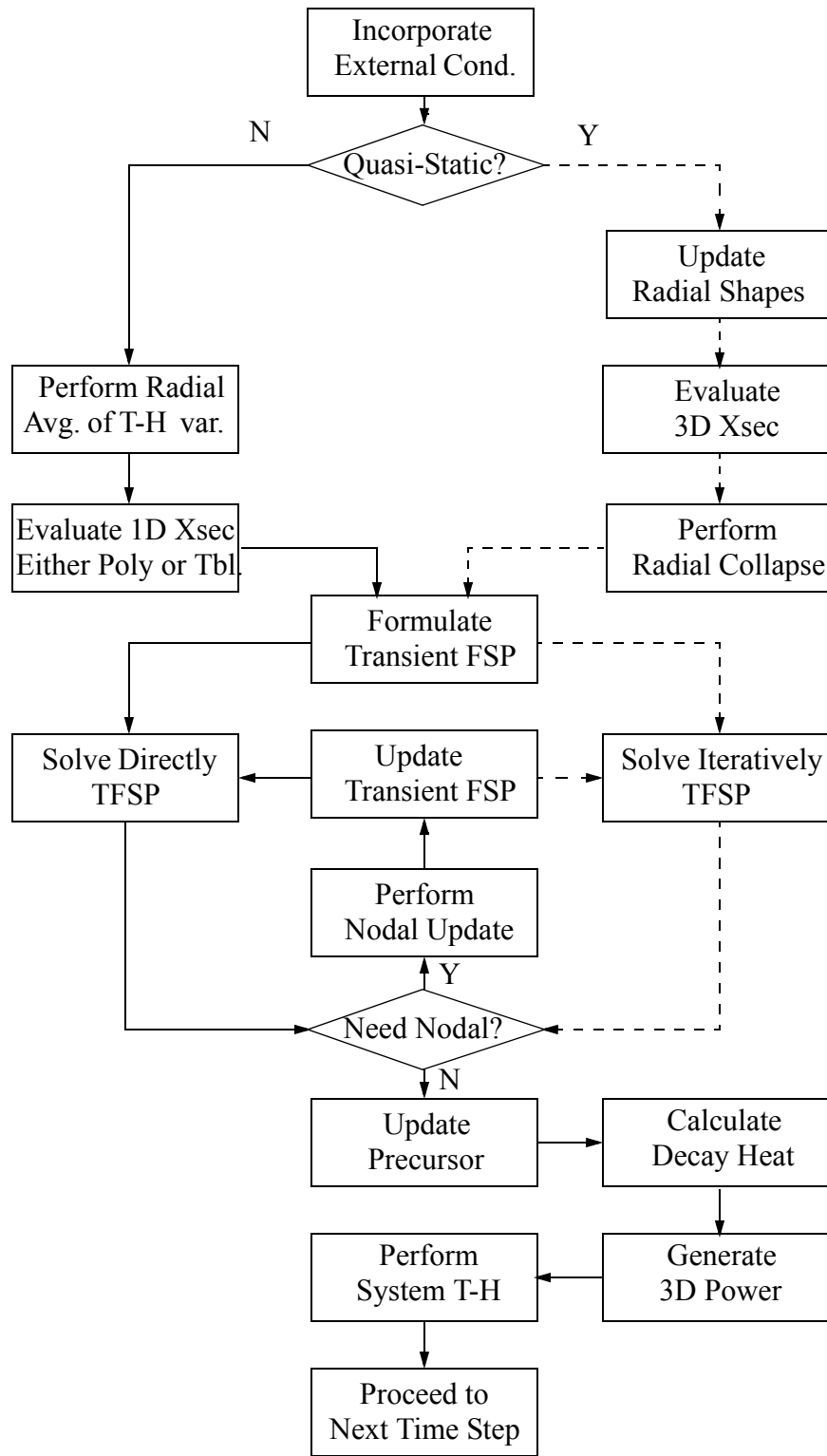
Figure 7.4: Transient 1-D Solution Sequence
