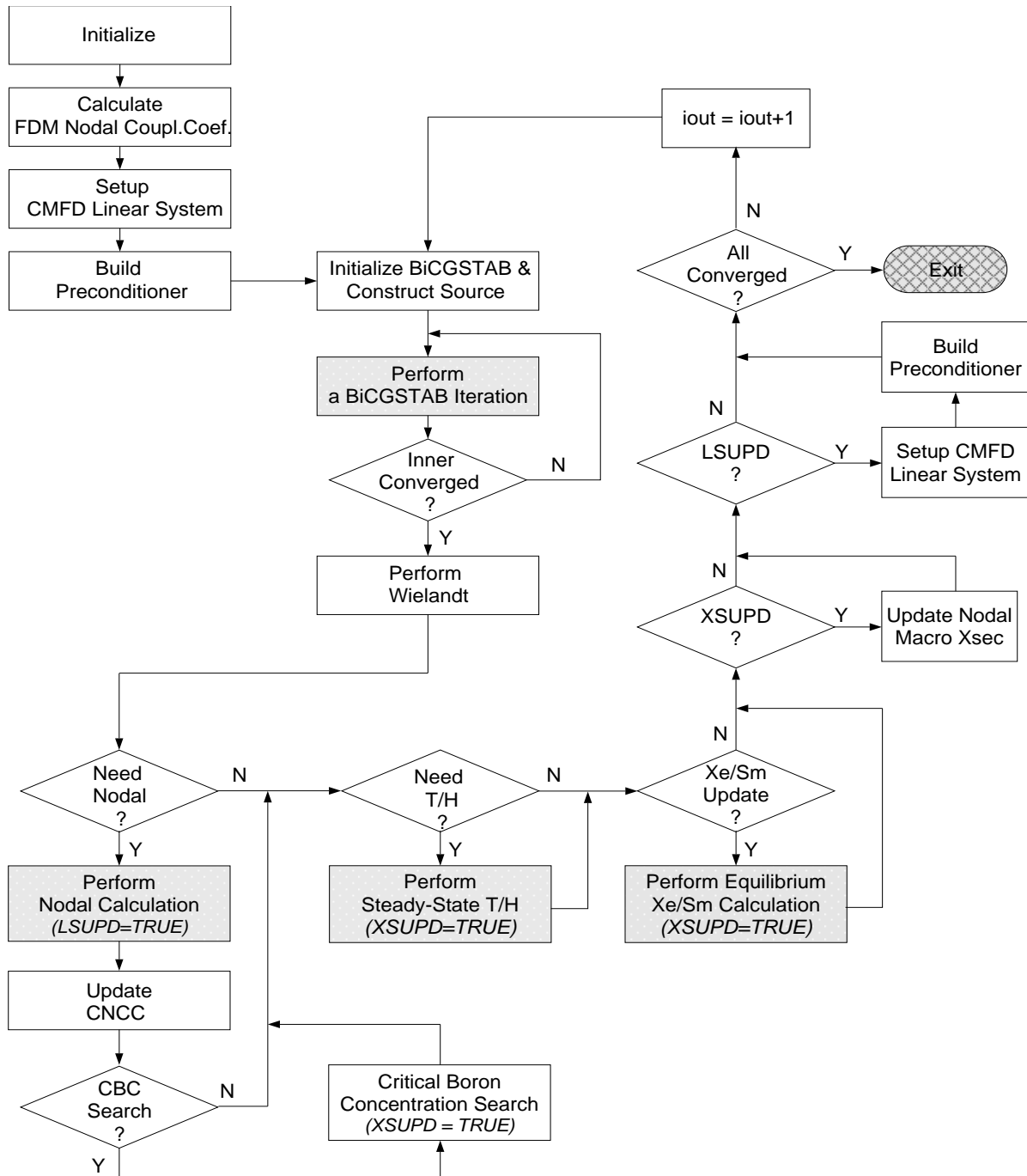
Figure 8.1: Eigenvalue Calculation Flow
