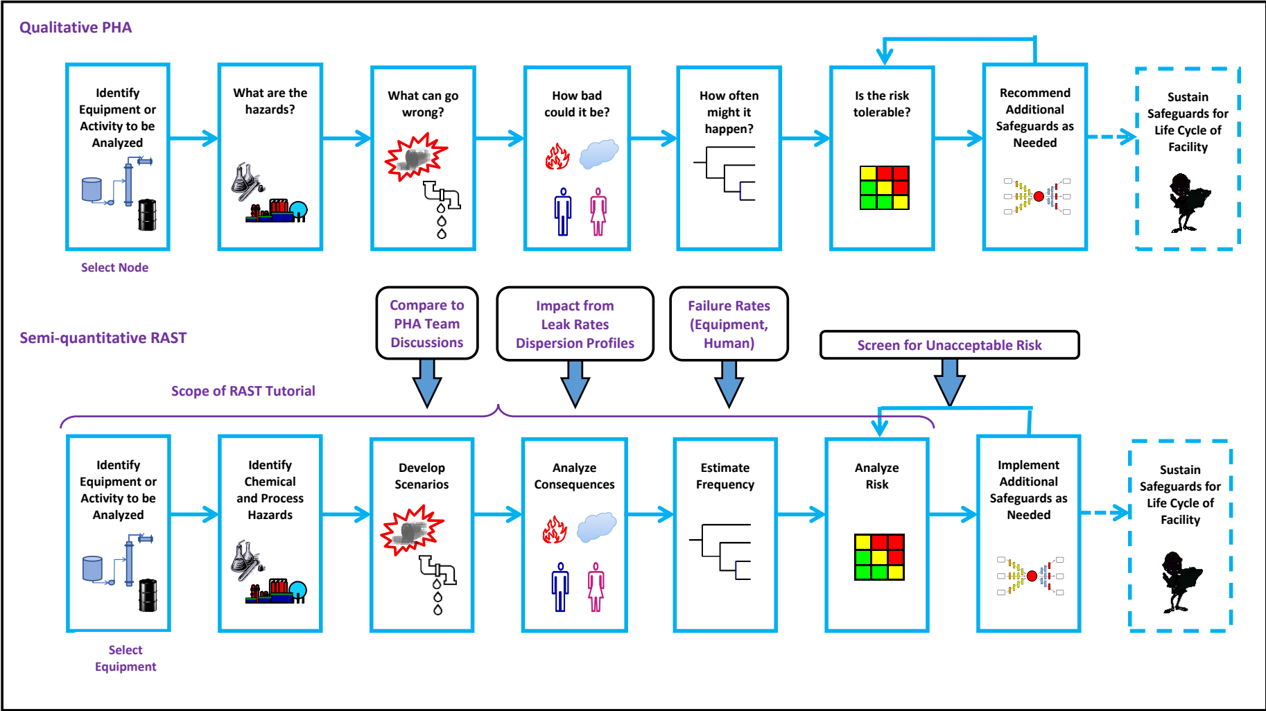
Figure 3 - A Hazards Identification and Risk Analysis (HIRA) Approach and how RAST is used to validate PHA Team's Scenarios
